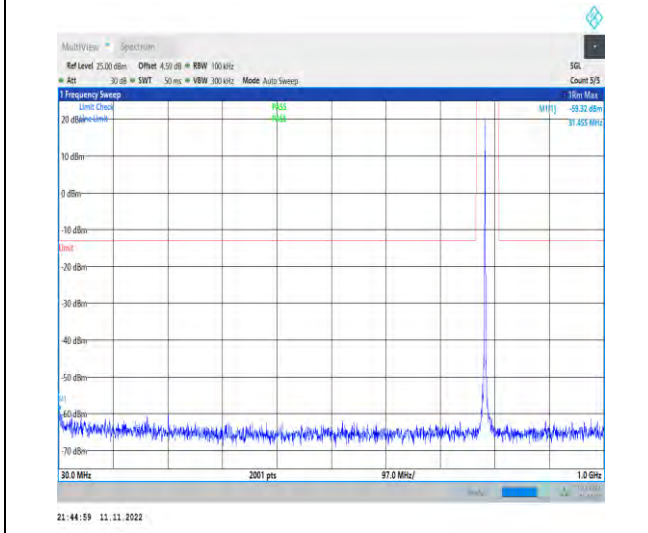
1-N14-PC3-15-10-H-1-DFT-PI2BPSK-Inner_1RB_L eft-1@1-30-1000-Ant1-31.46--59.32--13-PASS
