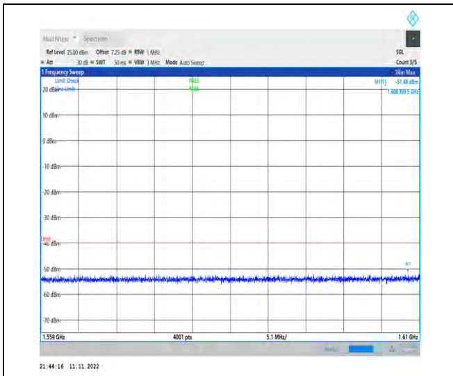
1-N14-PC3-15-10-M-1-DFT-PI2BPSK-Inner_1RB_L eft-1@1-1559-1610-Ant1-1608.39--51.48--40-PASS
