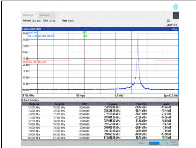
1-N14-PC3-15-10-H-2-DFT-PI2BPSK-Edge_1RB_Right-t-1@51-Ant1-1--PASS-see graph
