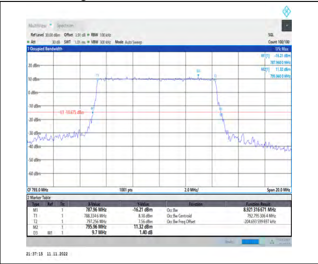
1-N14-PC3-15-10-L-3-DFT-16QAM-Outer_Full-50 @0-Ant1-8.921-9.700-≤10-PASS
