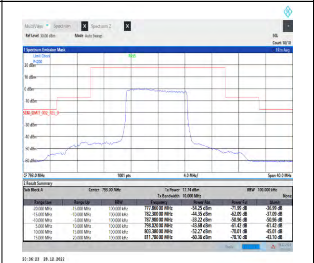
1-N14-PC3-15-10-H-3-DFT-PI2BPSK-Outer_Full-50@0-Ant1-1--PASS-see graph
