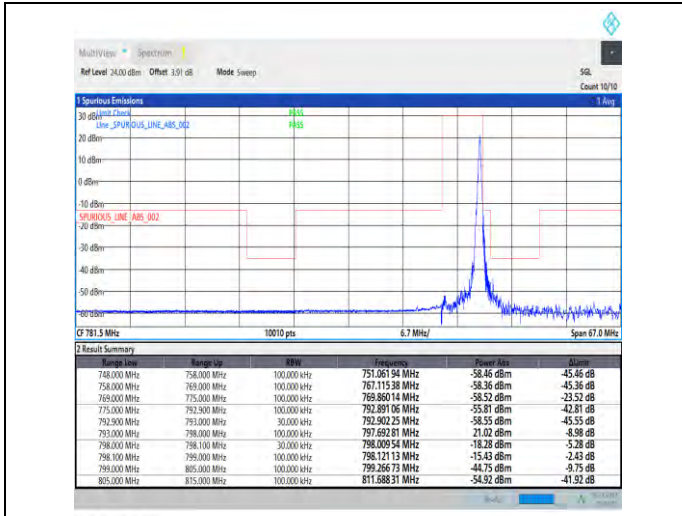
1-N14-PC3-15-5-H-2-DFT-PI2BPSK-Edge_1RB_Right-1@24-Ant1-1--PASS-see graph
