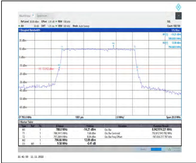
1-N14-PC3-15-10-H-4-DFT-64QAM-Outer_Full-50@ 0-Ant1-8.943-9.580-≤10-PASS
