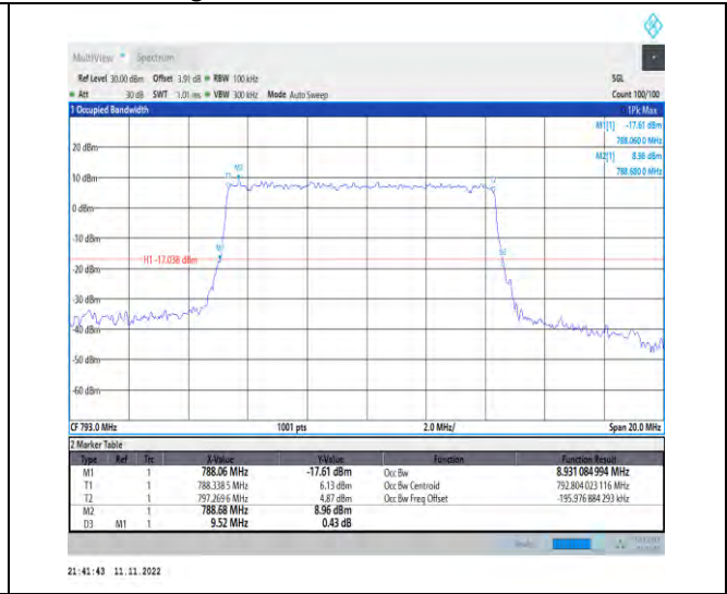
1-N14-PC3-15-10-H-5-DFT-256QAM-Outer_Full-50 @0-Ant1-8.931-9.520-≤10-PASS
