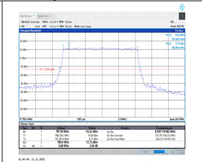
1-N14-PC3-15-10-H-1-DFT-QPSK-Outer_Full-50@0- Ant1-8.935-9.680-≤10-PASS
