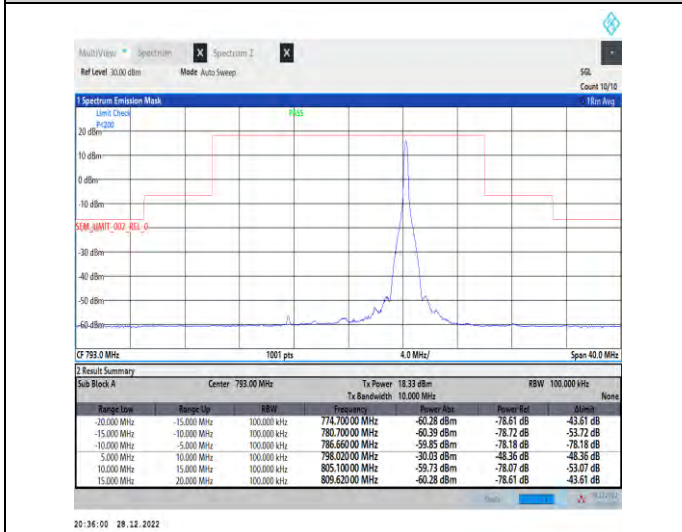
1-N14-PC3-15-10-H-2-DFT-PI2BPSK-Edge_1RB_Right-1@51-Ant1-1--PASS-see graph
