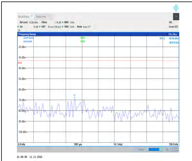
1-N14-PC3-15-10-H-1-DFT-PI2BPSK-Inner_1RB_L eft-1@1-0.009-0.15-Ant1-0.06--69.06--33-PASS
