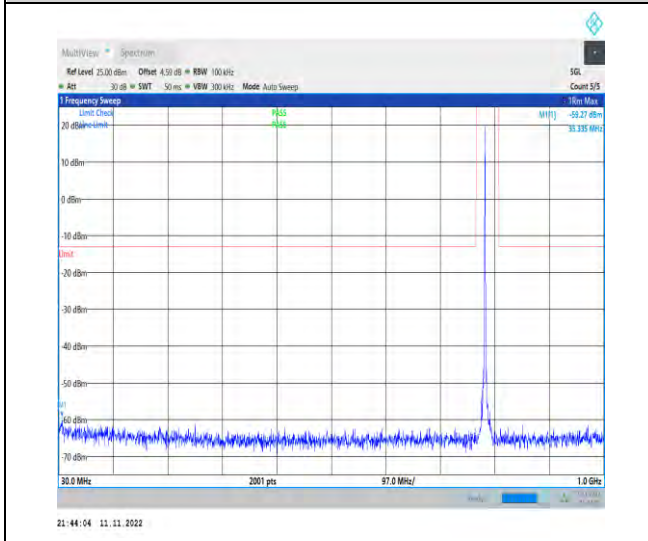
1-N14-PC3-15-10-M-1-DFT-PI2BPSK-Inner_1RB_L eft-1@1-30-1000-Ant1-35.34--59.27--13-PASS
