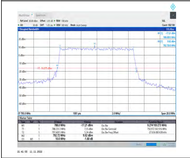
1-N14-PC3-15-10-H-6-CP-QPSK-Outer_Full-52@0- Ant1-9.274-10.000-≤10-PASS
