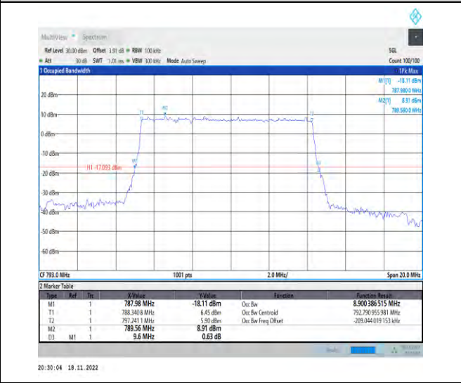
1-N14-PC3-15-10-L-5-DFT-256QAM-Outer_Full-50 @0-Ant1-8.9-9.600-≤10-PASS
