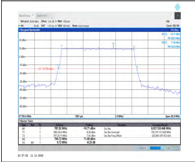
1-N14-PC3-15-10-L-4-DFT-64QAM-Outer_Full-50 @0-Ant1-8.922-9.720-≤10-PASS
