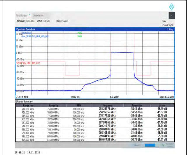
1-N14-PC3-15-10-L-6-CP-QPSK-Outer_Full-52@0-Ant1-1--PASS-see graph
