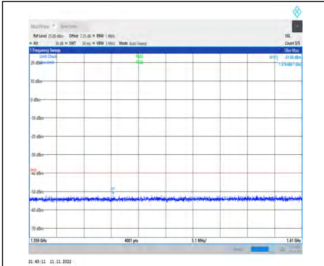
1-N14-PC3-15-10-H-1-DFT-PI2BPSK-Inner_1RB_L eft-1@1-1559-1610-Ant1-1574.67--51.84--40-PASS
