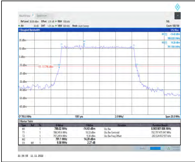
1-N14-PC3-15-10-L-2-DFT-PI2BPSK-Outer_Full-50 @0-Ant1-8.904-9.580-≤10-PASS
