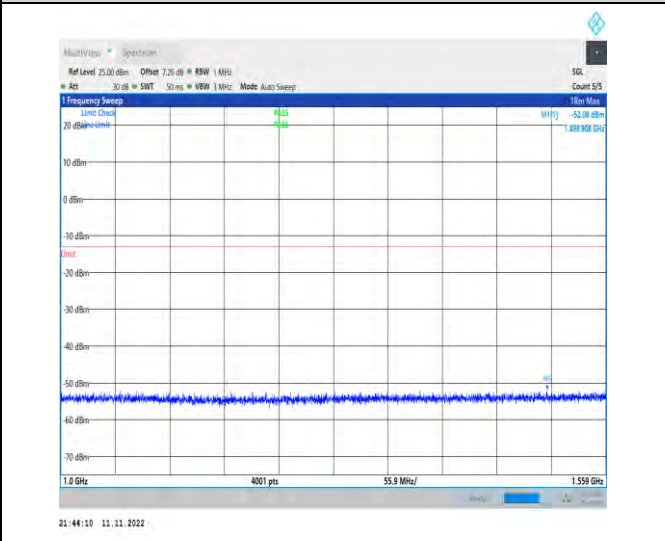
1-N14-PC3-15-10-M-1-DFT-PI2BPSK-Inner_1RB_Lef t-1@1-1000-1559-Ant1-1498.91--52.08--13-PASS
