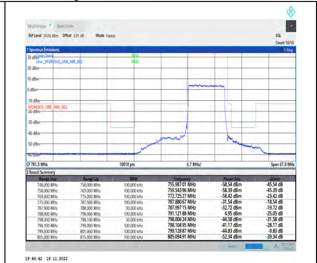
1-N14-PC3-15-10-L-3-DFT-PI2BPSK-Outer_Full-50@0-Ant1-1--PASS-see graph
