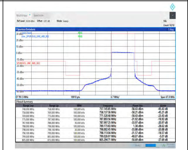
1-N14-PC3-15-10-H-3-DFT-PI2BPSK-Outer_Full-50@0-Ant1-1--PASS-see graph
