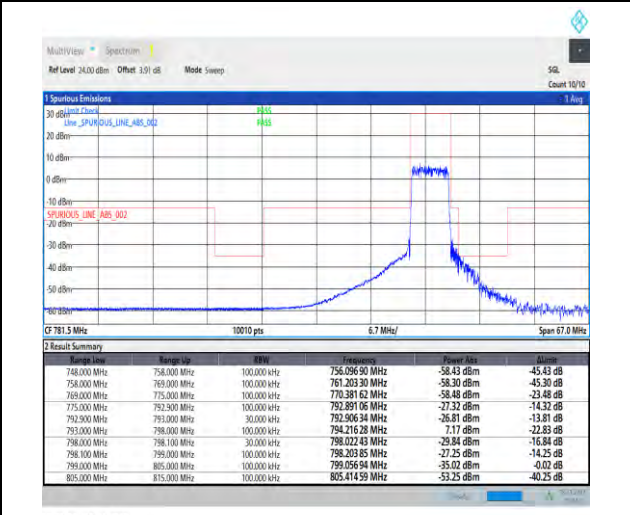
1-N14-PC3-15-5-H-3-DFT-PI2BPSK-Outer_Full-25@0-Ant1-1--PASS-see graph
