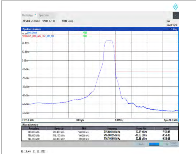
1-N12-PC3-15-10-H-2-DFT-PI2BPSK-Edge_1RB_Right-t-1@51-Ant1-1--PASS-see graph
