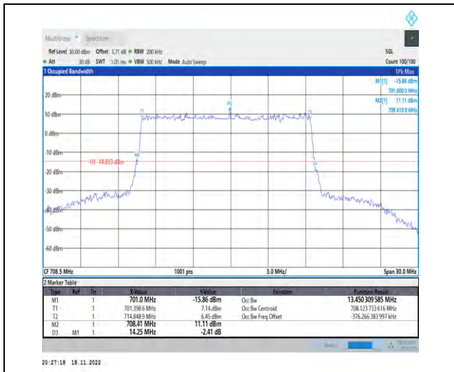
1-N12-PC3-15-15-H-5-DFT-256QAM-Outer_Full-75 @0-Ant1-13.45-14.250-≤15-PASS
