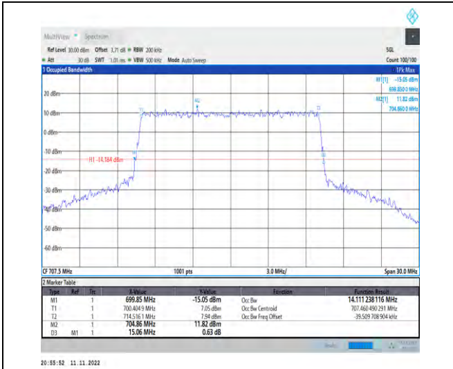
1-N12-PC3-15-15-M-6-CP-QPSK-Outer_Full-79@0-Ant1-14.111-15.060-≤15-PASS
