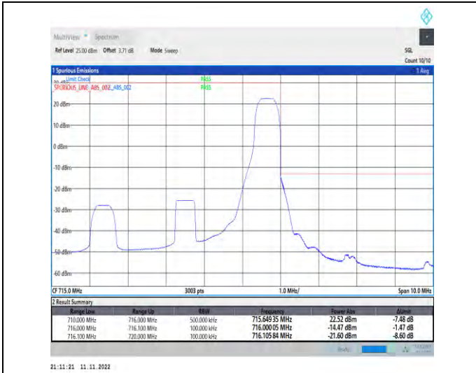
1-N12-PC3-15-5-H-2-DFT-PI2BPSK-Edge_1RB_Right-1@24-Ant1-1--PASS-see graph
