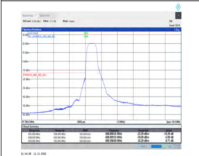
1-N12-PC3-15-10-L-4-CP-QPSK-Edge_1RB_Left-1@0-Ant1-1--PASS-see graph
