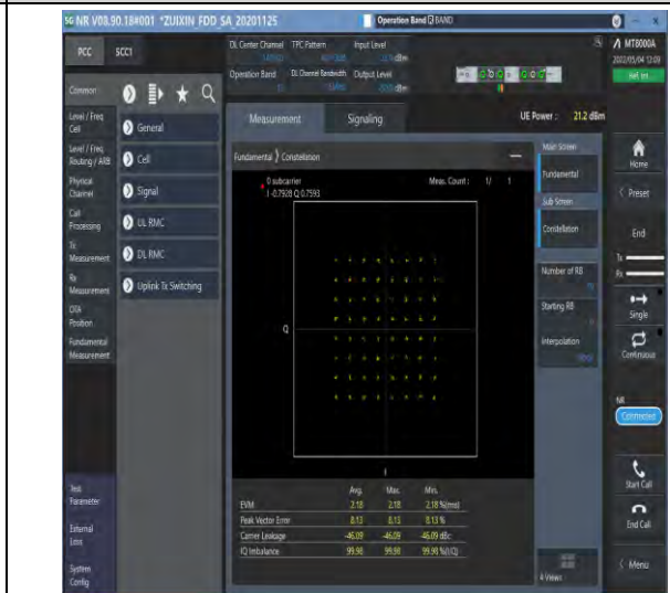
1-N12-PC3-15-15-M-8-CP-64QAM-Outer_Full-79@0-Ant1-see graph-PASS
