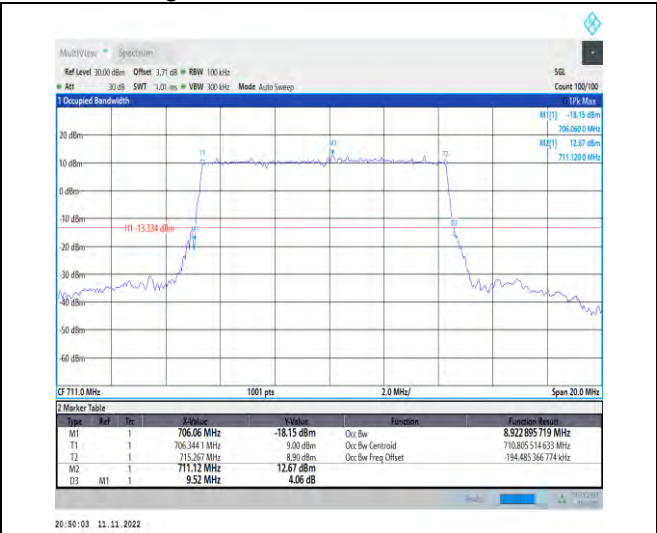
1-N12-PC3-15-10-H-1-DFT-QPSK-Outer_Full-50@ 0-Ant1-8.923-9.520-≤10-PASS
