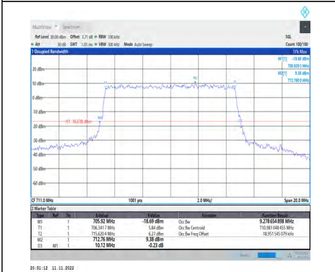
1-N12-PC3-15-10-H-6-CP-QPSK-Outer_Full-52@0- Ant1-9.279-10.120-≤10-PASS
