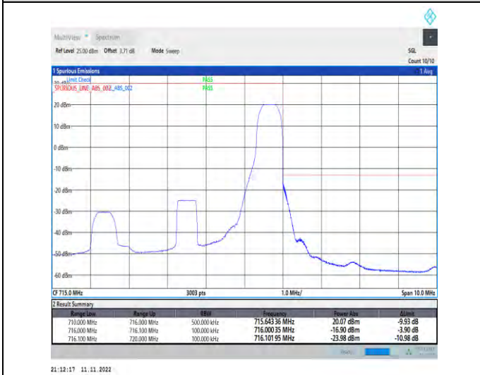
1-N12-PC3-15-5-H-5-CP-QPSK-Edge_1RB_Right-1@24-Ant1-1--PASS-see graph
