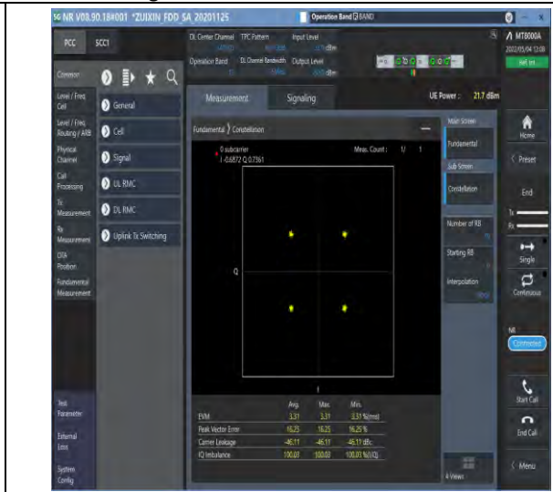
1-N12-PC3-15-15-M-6-CP-QPSK-Outer_Full-79@0-Ant1-see graph-PASS
