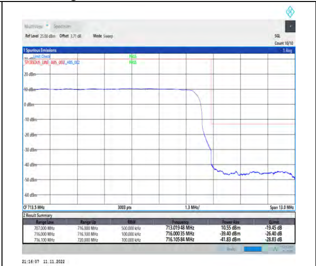
1-N12-PC3-15-10-H-3-DFT-PI2BPSK-Outer_Full-50@0-Ant1-1--PASS-see graph
