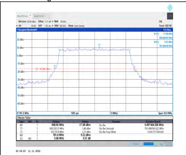
1-N12-PC3-15-5-L-6-CP-QPSK-Outer_Full-25@0-Ant1-4.498-5.080-<math>\leq</math>5-PASS
