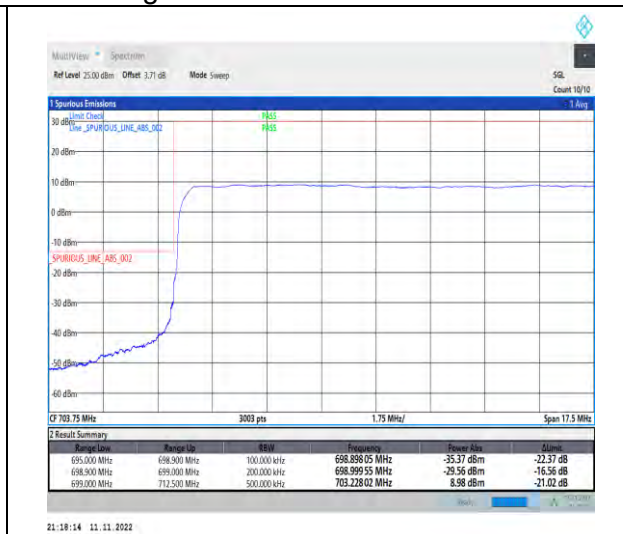
1-N12-PC3-15-15-L-3-DFT-PI2BPSK-Outer_Full-75@0-Ant1-1--PASS-see graph
