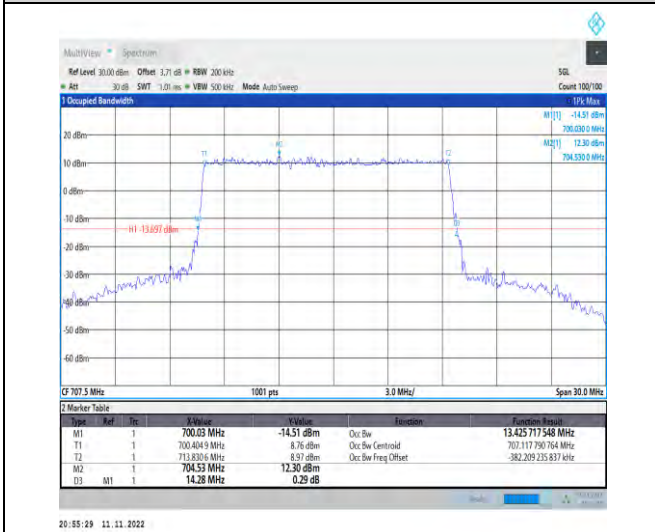
1-N12-PC3-15-15-M-4-DFT-64QAM-Outer_Full-75 @0-Ant1-13.426-14.280-≤15-PASS
