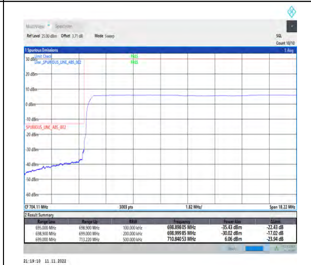
1-N12-PC3-15-15-L-6-CP-QPSK-Outer_Full-79@0-Ant1-1--PASS-see graph
