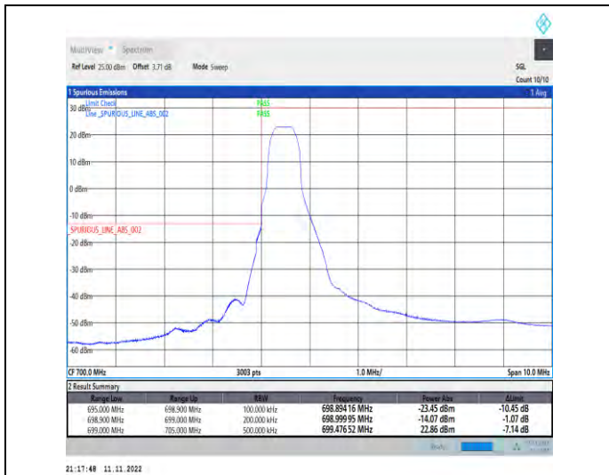
1-N12-PC3-15-15-L-1-DFT-PI2BPSK-Edge_1RB_Left-1@0-Ant1-1--PASS-see graph
