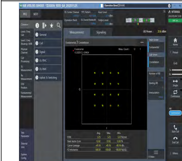
1-N12-PC3-15-15-M-7-CP-16QAM-Outer_Full-79@0-Ant1-see graph-PASS
