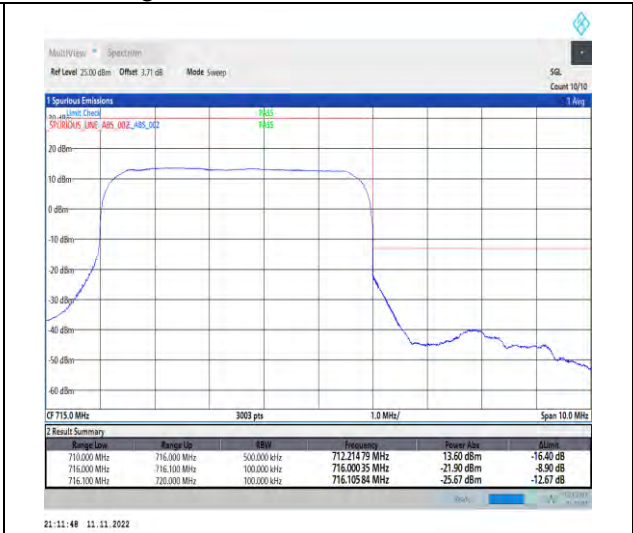
1-N12-PC3-15-5-H-3-DFT-PI2BPSK-Outer_Full-25@0-Ant1-1--PASS-see graph
