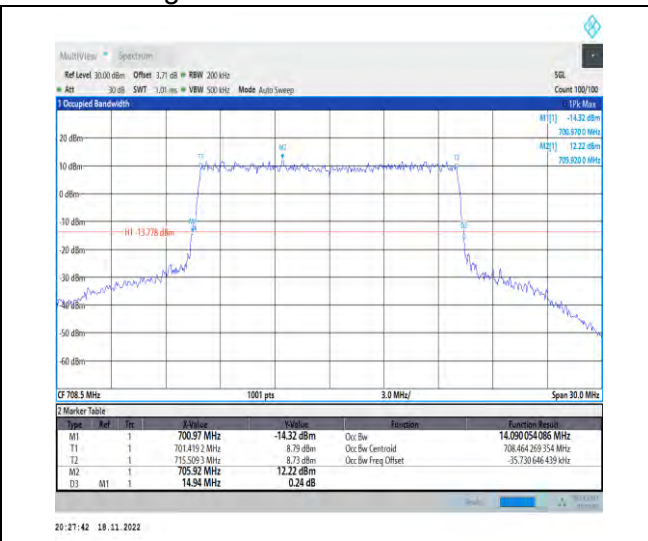
1-N12-PC3-15-15-H-6-CP-QPSK-Outer_Full-79@0-Ant1-14.09-14.940-≤15-PASS
