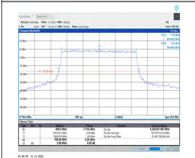
1-N12-PC3-15-10-L-8-CP-64QAM-Outer_Full-52@0- Ant1-9.259-9.980-≤10-PASS
