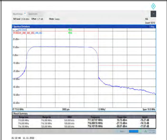
1-N12-PC3-15-5-H-6-CP-QPSK-Outer_Full-25@0-Ant1-1--PASS-see graph
