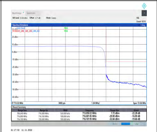
1-N12-PC3-15-10-H-6-CP-QPSK-Outer_Full-52@0-Ant1-1--PASS-see graph
