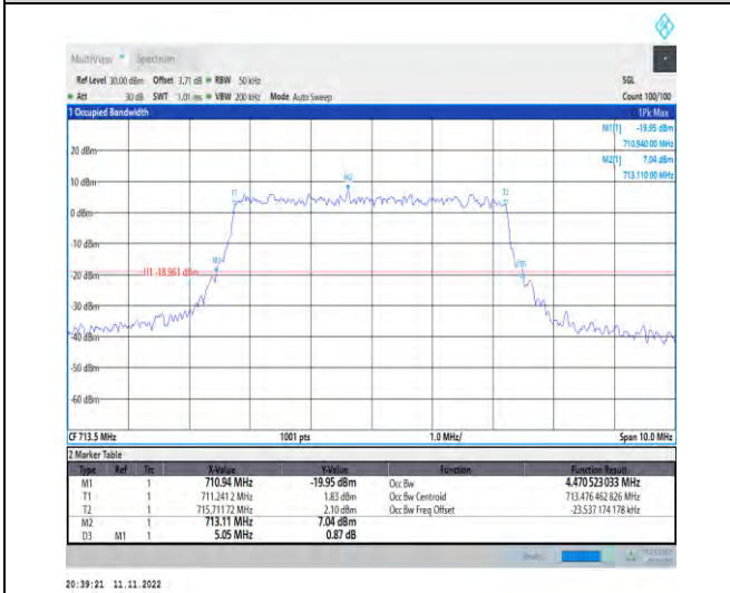
1-N12-PC3-15-5-H-9-CP-256QAM-Outer_Full-25@0-Ant1-4.471-5.050-≤5-PASS
