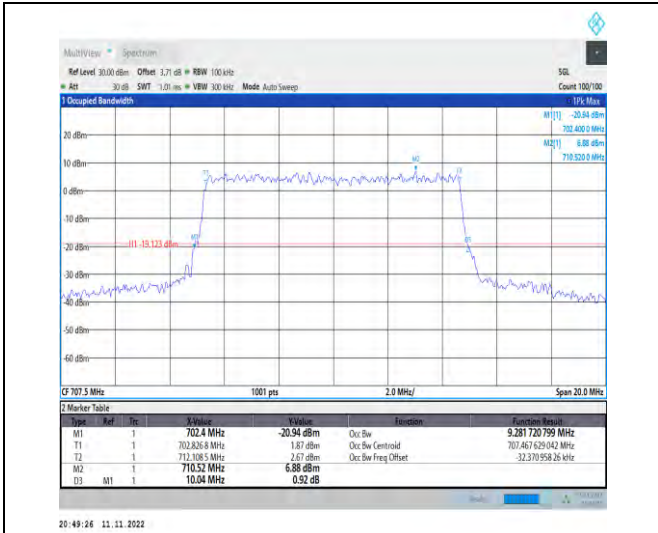
1-N12-PC3-15-10-M-9-CP-256QAM-Outer_Full-52@ 0-Ant1-9.282-10.040-≤10-PASS
