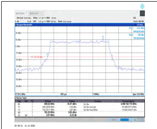
1-N12-PC3-15-5-L-5-DFT-256QAM-Outer_Full-25@0-Ant1-4.49-4.970-<math>\leq</math>5-PASS
