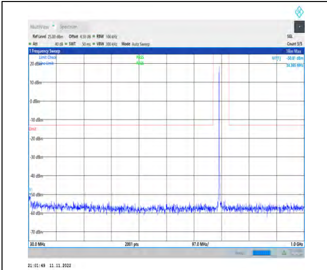
1-N12-PC3-15-15-M-1-DFT-PI2BPSK-Inner_1RB_L eft-1@1-30-1000-Ant1-34.37--50.81--13-PASS
