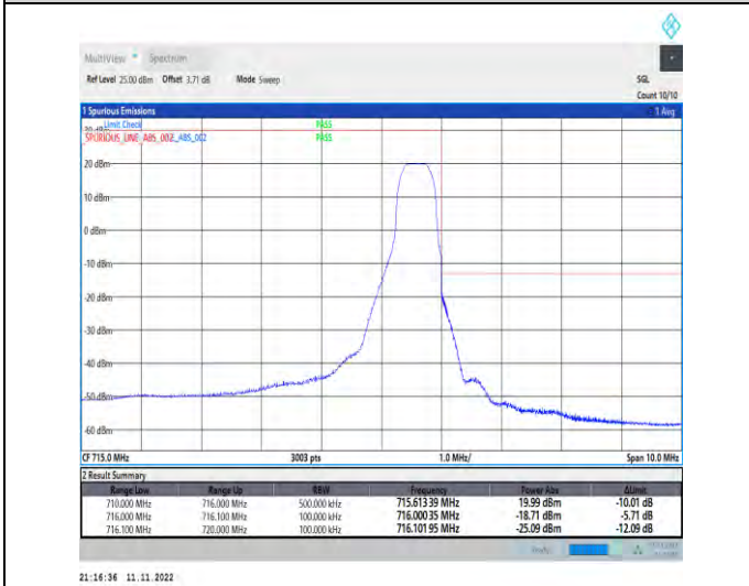
1-N12-PC3-15-10-H-5-CP-QPSK-Edge_1RB_Right-1@51-Ant1-1--PASS-see graph
