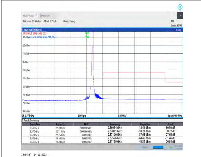
1-N7-PC3-15-40-H-5-CP-QPSK-Edge_1RB_Right-1@215-Ant1-1--PASS-see graph
