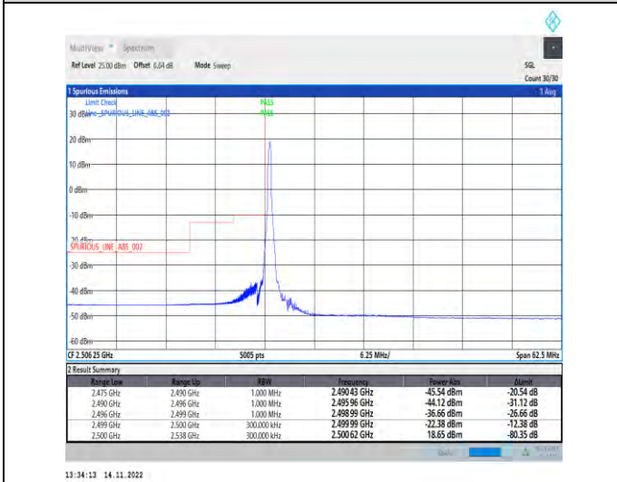
1-N7-PC3-15-25-L-4-CP-QPSK-Edge_1RB_Left-1@0-Ant1-1--PASS-see graph
