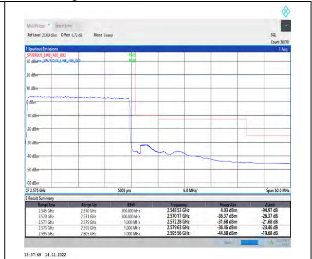
1-N7-PC3-15-25-H-3-DFT-PI2BPSK-Outer_Full-128@0-Ant1-1--PASS-see graph
