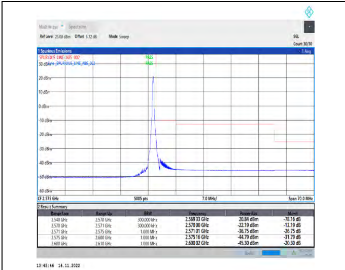
1-N7-PC3-15-30-H-2-DFT-PI2BPSK-Edge_1RB_Right-1@159-Ant1-1--PASS-see graph
