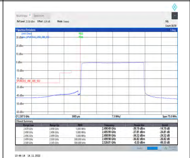
1-N7-PC3-15-30-L-6-CP-QPSK-Outer_Full-160 @0-Ant1-1--PASS-see graph
