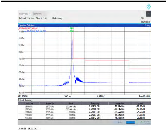
1-N7-PC3-15-25-H-5-CP-QPSK-Edge_1RB_Right-1@132-Ant1-1--PASS-see graph
