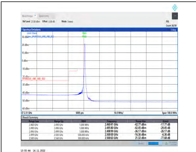
1-N7-PC3-15-40-L-1-DFT-PI2BPSK-Edge_1RB_Left-1 @0-Ant1-1--PASS-see graph
