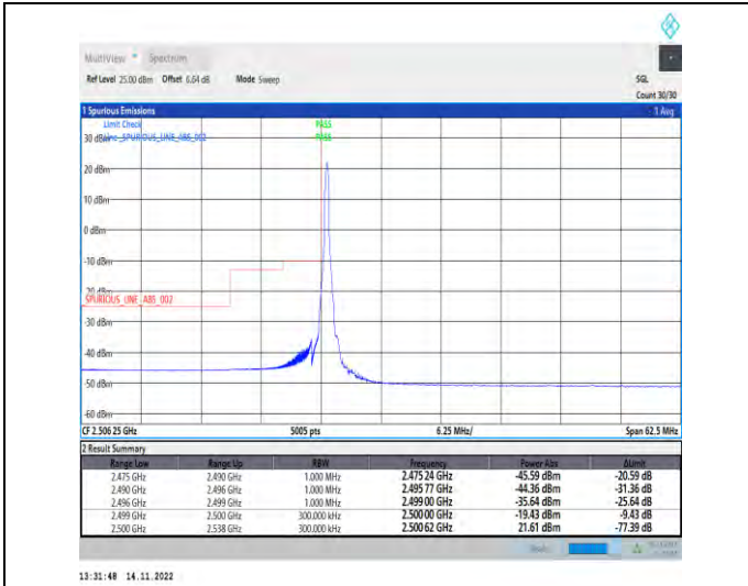
1-N7-PC3-15-25-L-1-DFT-PI2BPSK-Edge_1RB_Left-1 @0-Ant1-1--PASS-see graph
