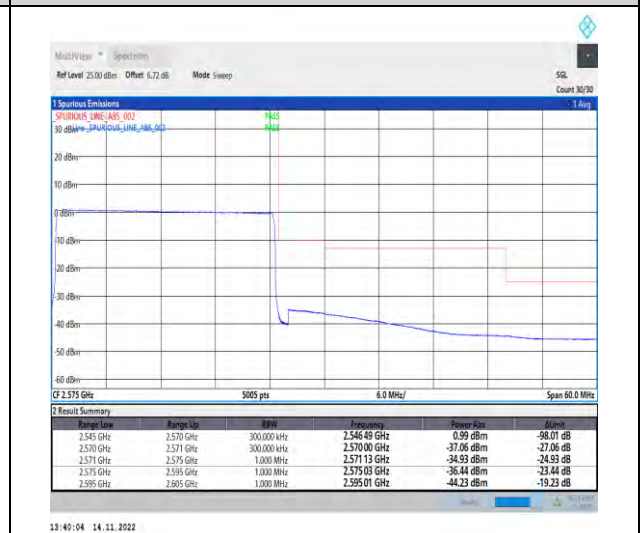
1-N7-PC3-15-25-H-6-CP-QPSK-Outer_Full-133@0-Ant1-1--PASS-see graph
