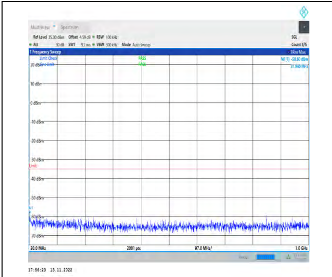
1-N7-PC3-15-40-M-1-DFT-PI2BPSK-Inner_1RB_Lef t-1@1-30-1000-Ant1-31.94--58.80--35-PASS
