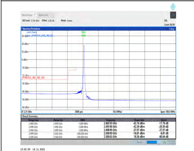
1-N7-PC3-15-40-L-4-CP-QPSK-Edge_1RB_Left-1@0-Ant1-1--PASS-see graph
