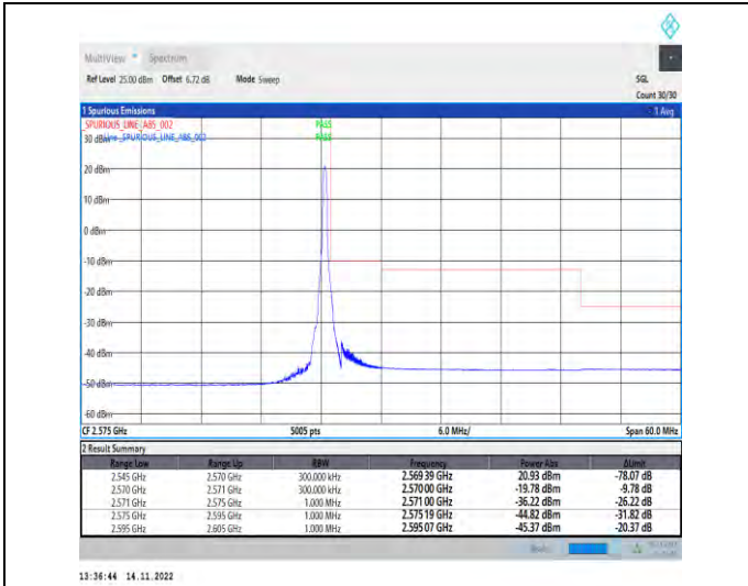
1-N7-PC3-15-25-H-2-DFT-PI2BPSK-Edge_1RB_Right-1@132-Ant1-1--PASS-see graph
