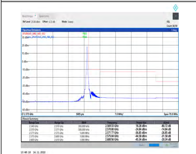
1-N7-PC3-15-30-H-5-CP-QPSK-Edge_1RB_Right-1@159-Ant1-1--PASS-see graph
