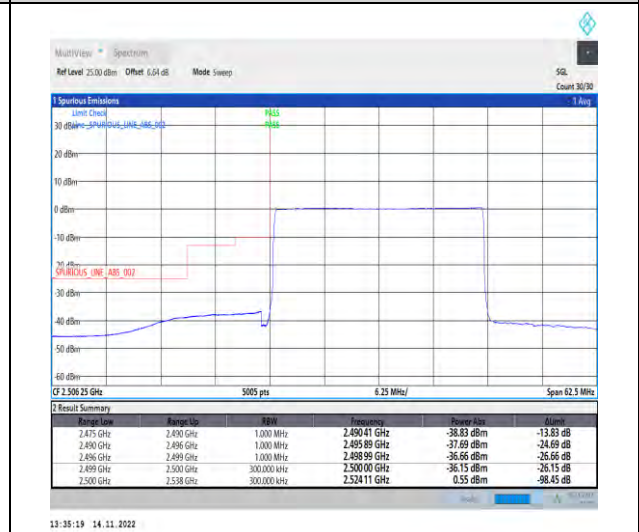
1-N7-PC3-15-25-L-6-CP-QPSK-Outer_Full-133@0-Ant1-1--PASS-see graph
