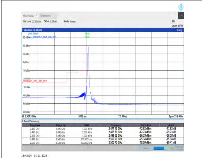
1-N7-PC3-15-30-L-4-CP-QPSK-Edge_1RB_Left-1 @0-Ant1-1--PASS-see graph
