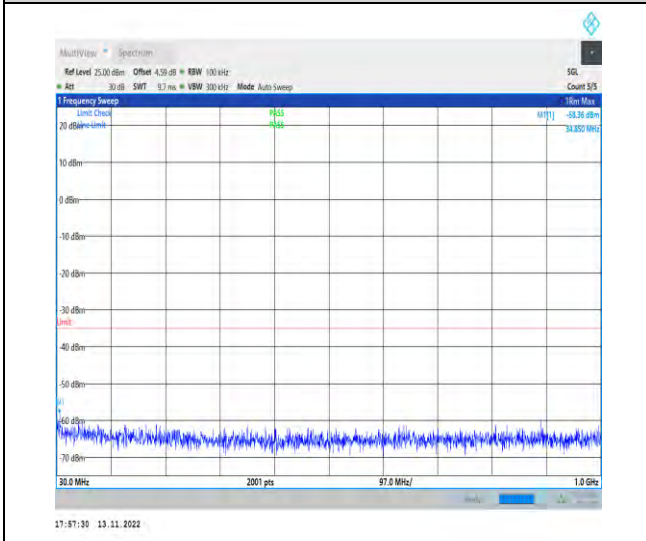
1-N7-PC3-15-40-H-1-DFT-PI2BPSK-Inner_1RB_Lef t-1@1-30-1000-Ant1-34.85--58.36--35-PASS
