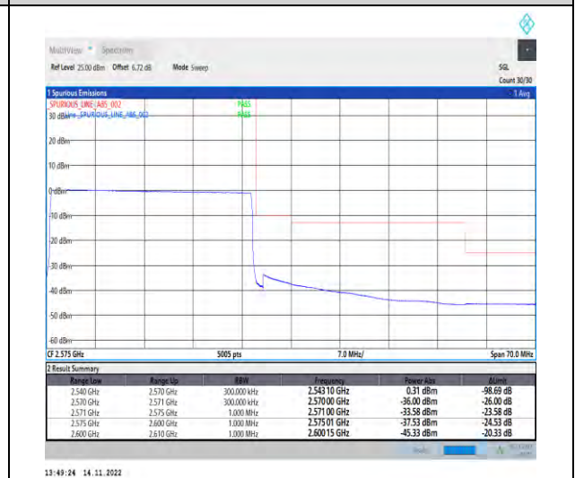
1-N7-PC3-15-30-H-6-CP-QPSK-Outer_Full-160@0-Ant1-1--PASS-see graph
