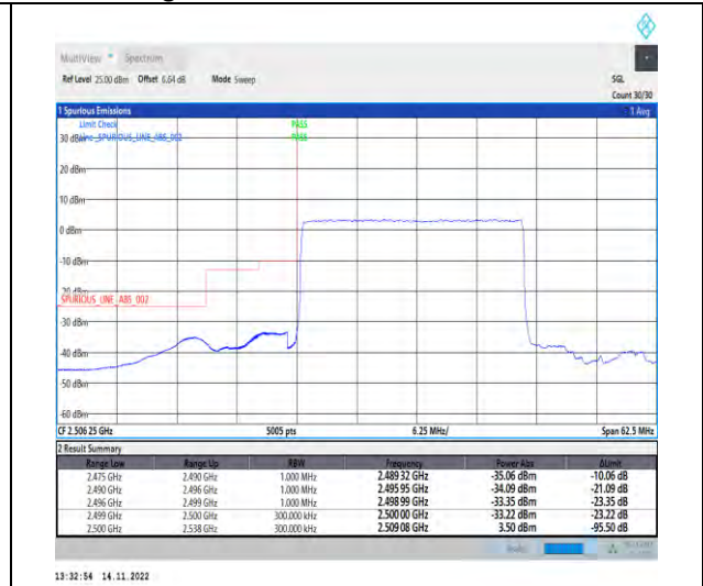
1-N7-PC3-15-25-L-3-DFT-PI2BPSK-Outer_Full-12 8@0-Ant1-1--PASS-see graph
