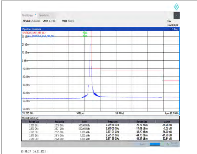
1-N7-PC3-15-40-H-2-DFT-PI2BPSK-Edge_1RB_Right-1@215-Ant1-1--PASS-see graph
