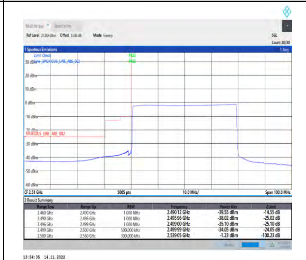
1-N7-PC3-15-40-L-6-CP-QPSK-Outer_Full-216@0-Ant1-1--PASS-see graph
