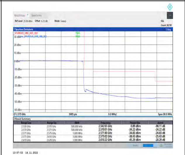
1-N7-PC3-15-40-H-6-CP-QPSK-Outer_Full-216@0-Ant1-1--PASS-see graph
