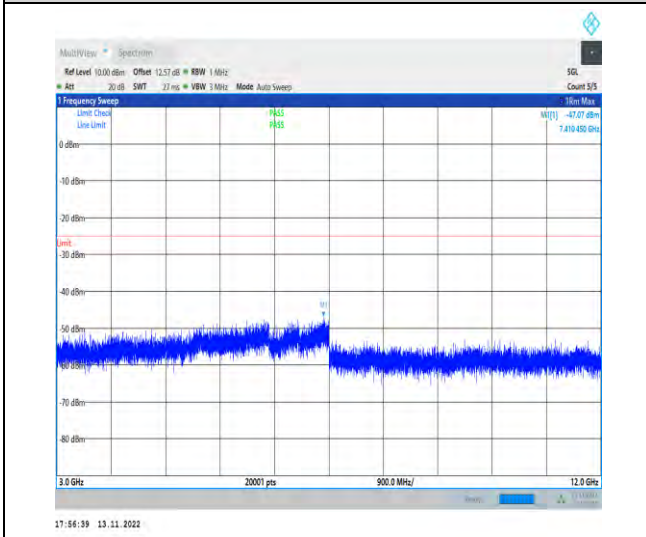
1-N7-PC3-15-40-M-1-DFT-PI2BPSK-Inner_1RB_Lef t-1@1-3000-12000-Ant1-7410.45--47.07--25-PASS
