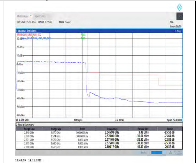
1-N7-PC3-15-30-H-3-DFT-PI2BPSK-Outer_Full-160@0-Ant1-1--PASS-see graph
