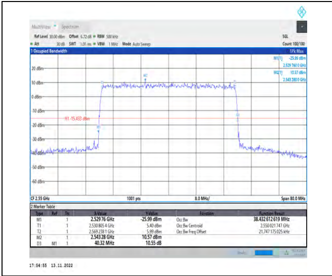
1-N7-PC3-15-40-H-5-DFT-256QAM-Outer_Full-216 @0-Ant1-38.433-40.320-≤40-PASS
