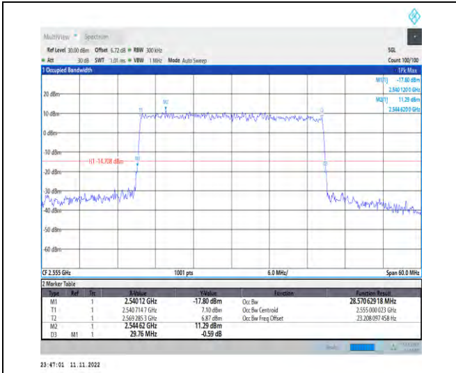
1-N7-PC3-15-30-H-4-DFT-64QAM-Outer_Full-160@ 0-Ant1-28.571-29.760-≤30-PASS
