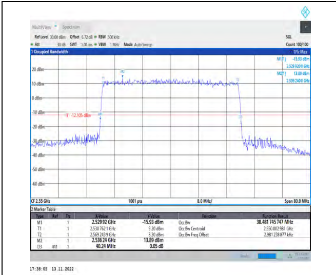
1-N7-PC3-15-40-H-1-DFT-QPSK-Outer_Full-216@0-Ant1-38.482-40.240-<math>\leq 40</math>-PASS
