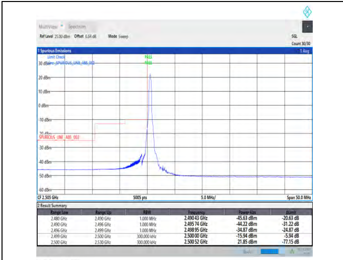
1-N7-PC3-15-20-L-1-DFT-PI2BPSK-Edge_1RB_Left-1 @0-Ant1-1--PASS-see graph
