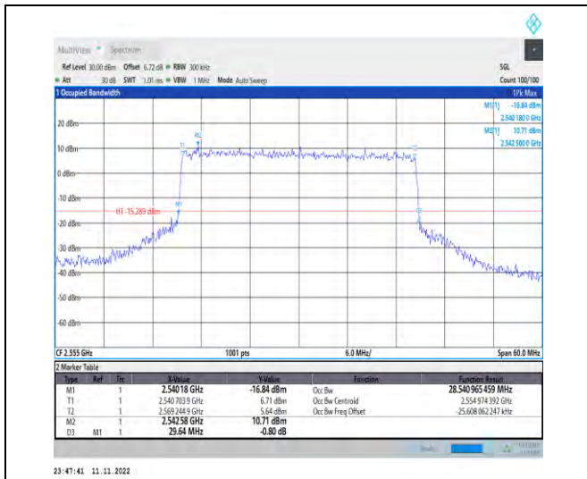
1-N7-PC3-15-30-H-8-CP-64QAM-Outer_Full-160@0 -Ant1-28.541-29.640-≤30-PASS
