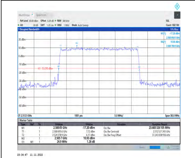
1-N7-PC3-15-25-L-7-CP-16QAM-Outer_Full-133@0-Ant1-23.683-24.900-≤25-PASS
