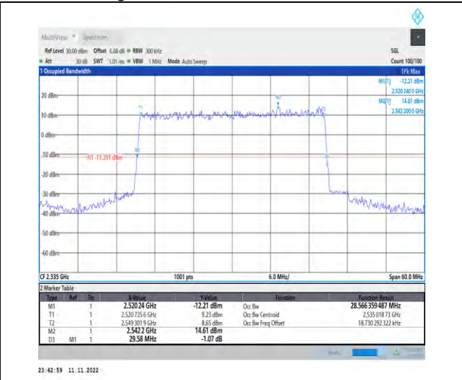
1-N7-PC3-15-30-M-2-DFT-PI2BPSK-Outer_Full-160@0-Ant1-28.566-29.580-≤30-PASS
