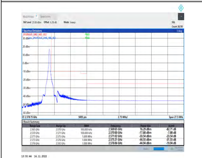
1-N7-PC3-15-5-H-5-CP-QPSK-Edge_1RB_Right-1@2 4-Ant1-1--PASS-see graph
