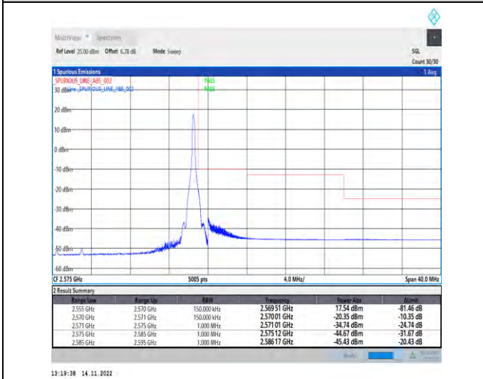
1-N7-PC3-15-15-H-5-CP-QPSK-Edge_1RB_Right-1@78-Ant1-1--PASS-see graph
