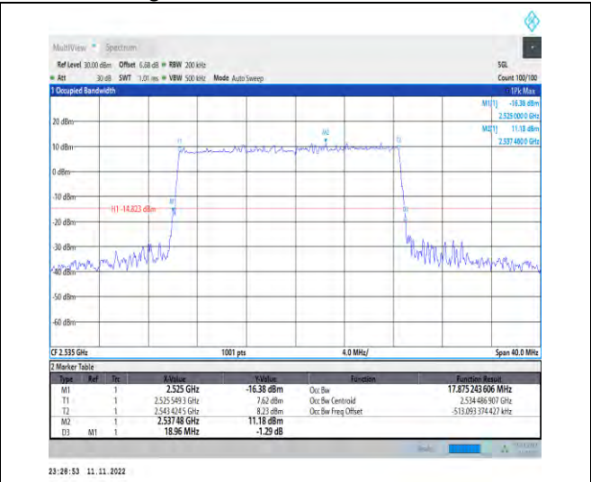
1-N7-PC3-15-20-M-4-DFT-64QAM-Outer_Full-100@ 0-Ant1-17.875-18.960-≤20-PASS
