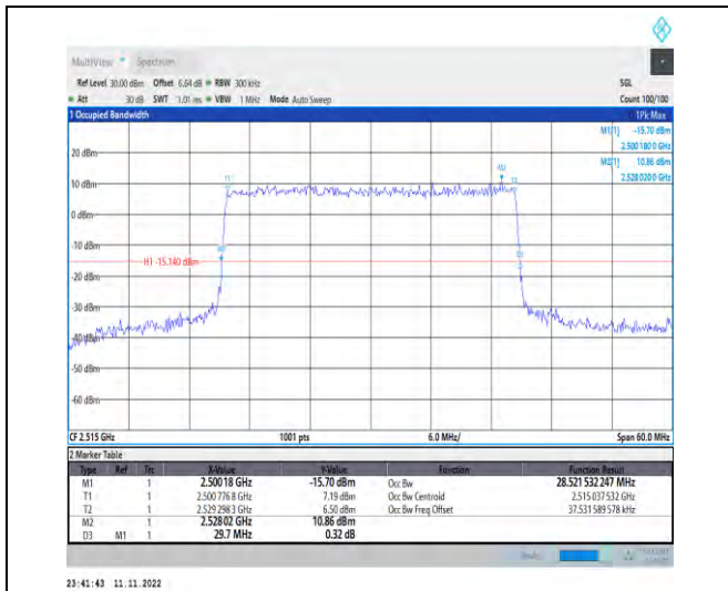
1-N7-PC3-15-30-L-6-CP-QPSK-Outer_Full-160@0-A Ant1-28.522-29.700-≤30-PASS
