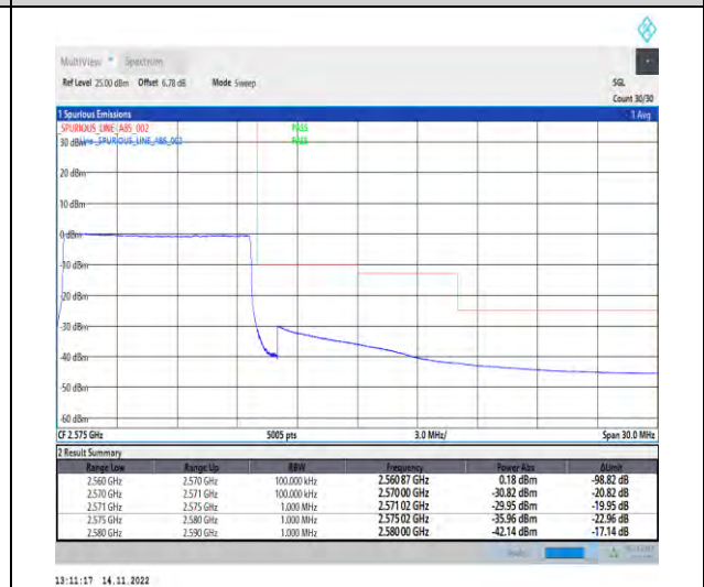
1-N7-PC3-15-10-H-6-CP-QPSK-Outer_Full-52@0-Ant1-1--PASS-see graph
