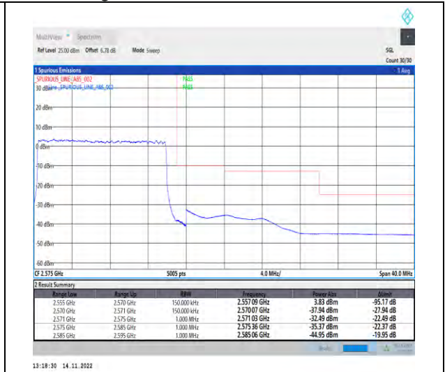
1-N7-PC3-15-15-H-3-DFT-PI2BPSK-Outer_Full-75@0-Ant1-1--PASS-see graph
