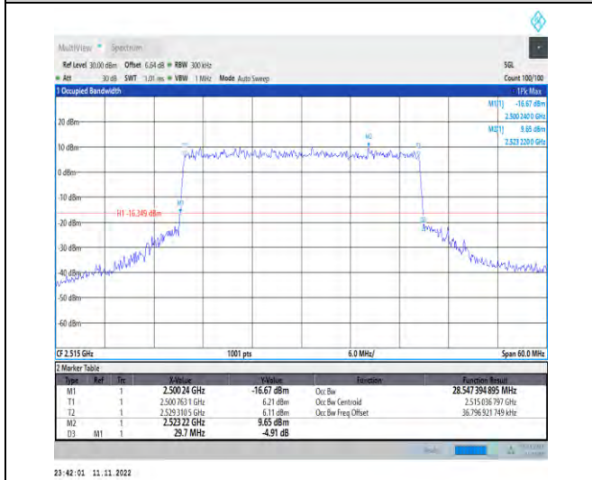
1-N7-PC3-15-30-L-8-CP-64QAM-Outer_Full-160@0- Ant1-28.547-29.700-≤30-PASS
