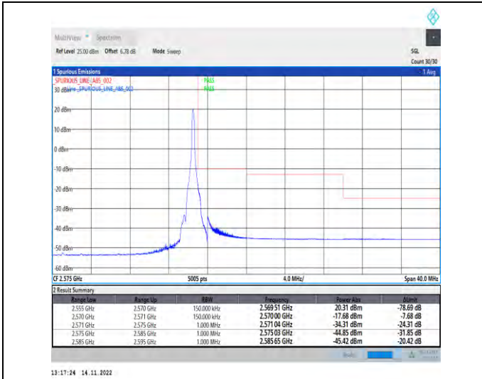
1-N7-PC3-15-15-H-2-DFT-PI2BPSK-Edge_1RB_Right-1@78-Ant1-1--PASS-see graph
