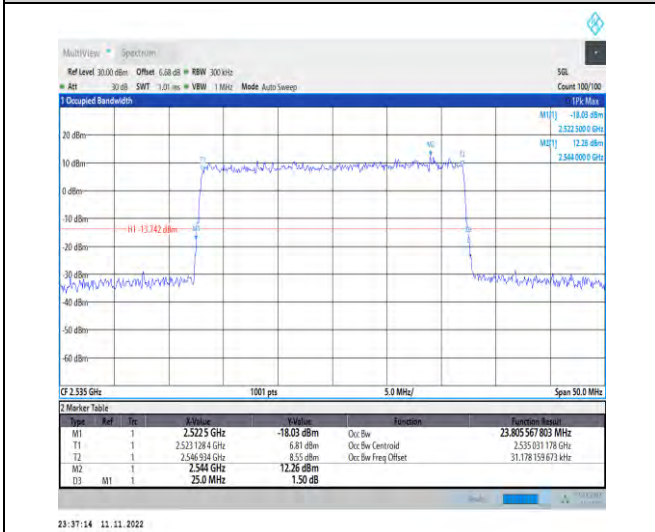
1-N7-PC3-15-25-M-6-CP-QPSK-Outer_Full-133@0- Ant1-23.806-25.000-≤25-PASS
