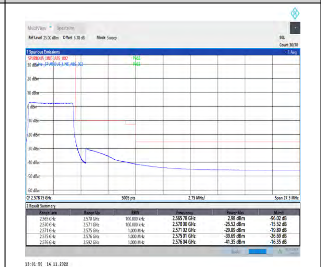
1-N7-PC3-15-5-H-6-CP-QPSK-Outer_Full-25@0-Ant1-1--PASS-see graph
