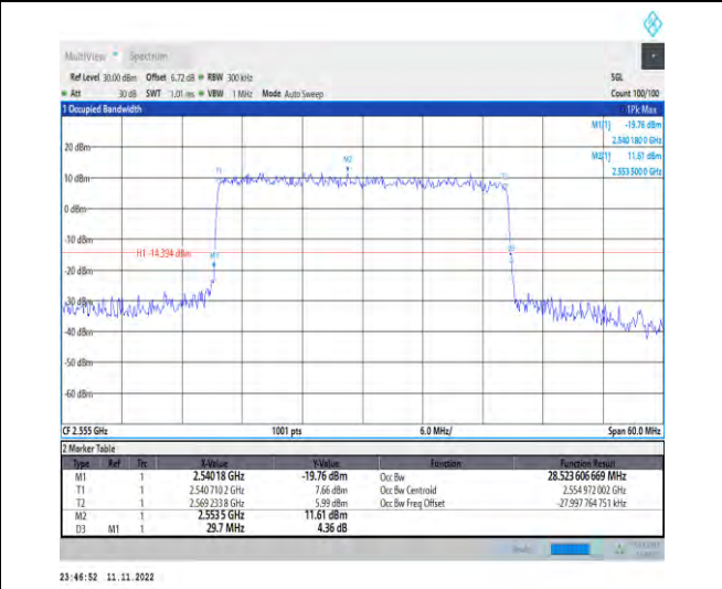
1-N7-PC3-15-30-H-3-DFT-16QAM-Outer_Full-160@ 0-Ant1-28.524-29.700-≤30-PASS
