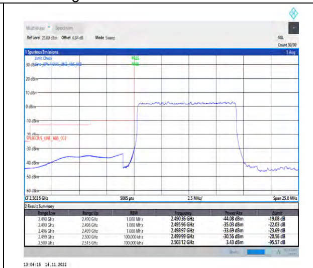
1-N7-PC3-15-10-L-3-DFT-PI2BPSK-Outer_Full-50 @0-Ant1-1--PASS-see graph
