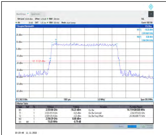
1-N7-PC3-15-15-H-9-CP-256QAM-Outer_Full-79@0 -Ant1-14.119-15.030-≤15-PASS
