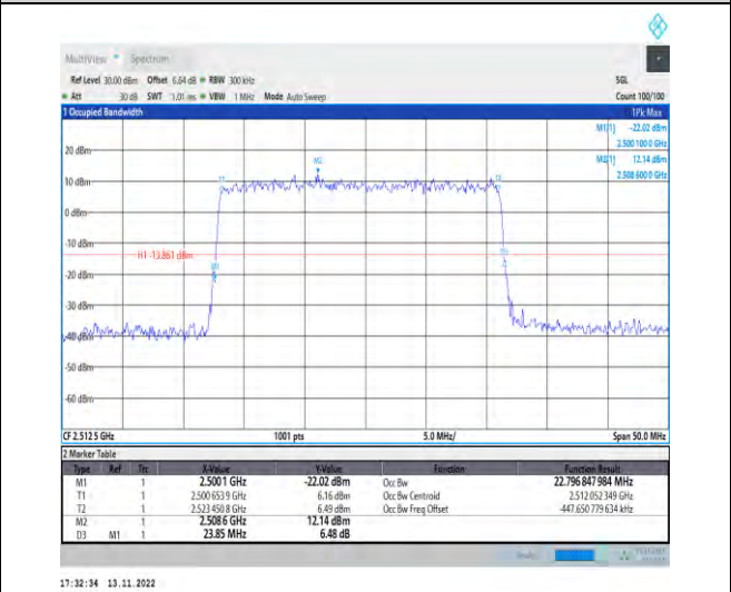
1-N7-PC3-15-25-L-4-DFT-64QAM-Outer_Full-128@0-Ant1-22.797-23.850-≤25-PASS
