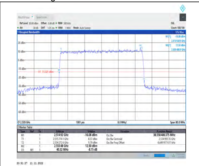
1-N7-PC3-15-40-M-3-DFT-16QAM-Outer_Full-216 @0-Ant1-38.558-40.320-≤40-PASS
