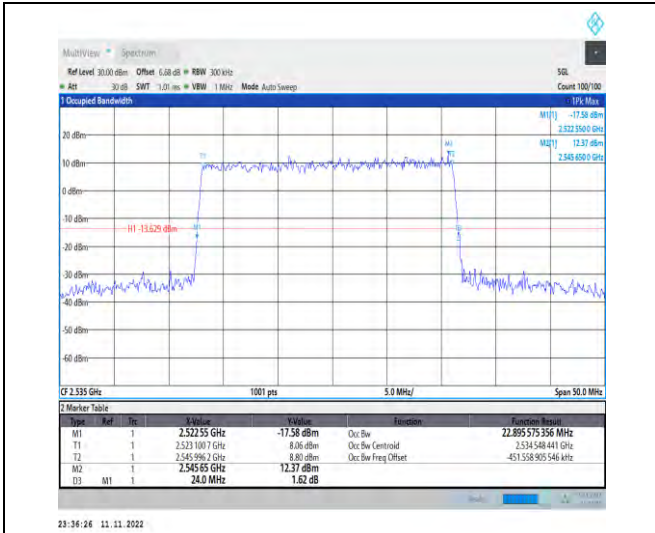
1-N7-PC3-15-25-M-4-DFT-64QAM-Outer_Full-128@ 0-Ant1-22.896-24.000-≤25-PASS
