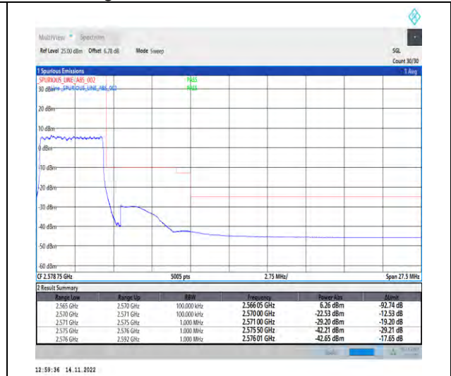
1-N7-PC3-15-5-H-3-DFT-PI2BPSK-Outer_Full-25 @0-Ant1-1--PASS-see graph
