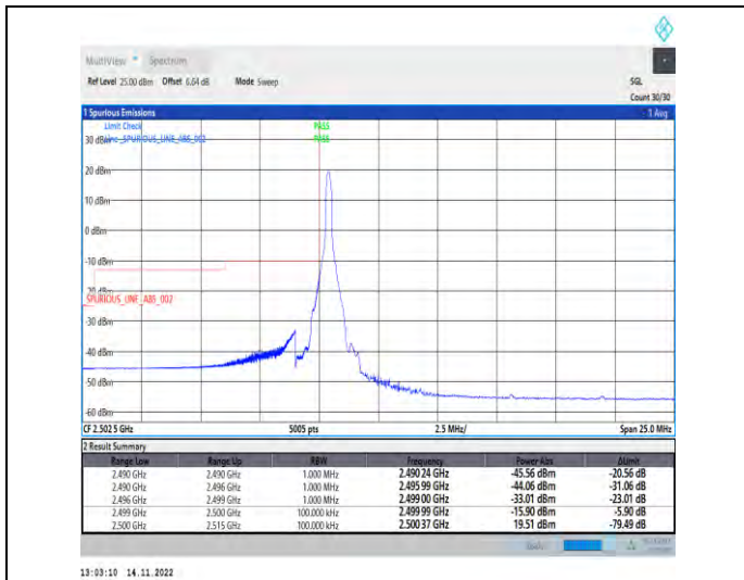
1-N7-PC3-15-10-L-1-DFT-PI2BPSK-Edge_1RB_Left-1 @0-Ant1-1--PASS-see graph
