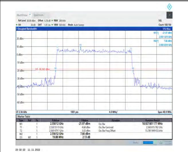
1-N7-PC3-15-20-H-9-CP-256QAM-Outer_Full-106@0-Ant1-18.928-19.880-<math>\leq 20</math>-PASS
