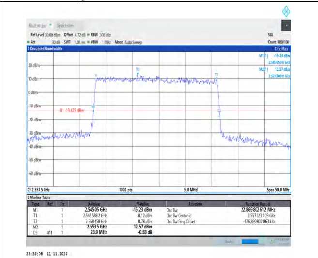
1-N7-PC3-15-25-H-4-DFT-64QAM-Outer_Full-128@ 0-Ant1-22.87-23.900-≤25-PASS
