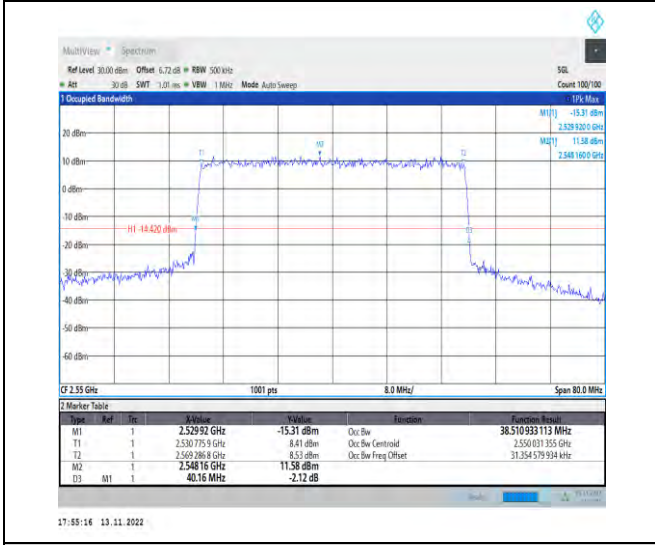
1-N7-PC3-15-40-H-7-CP-16QAM-Outer_Full-216@0 -Ant1-38.511-40.160-≤40-PASS
