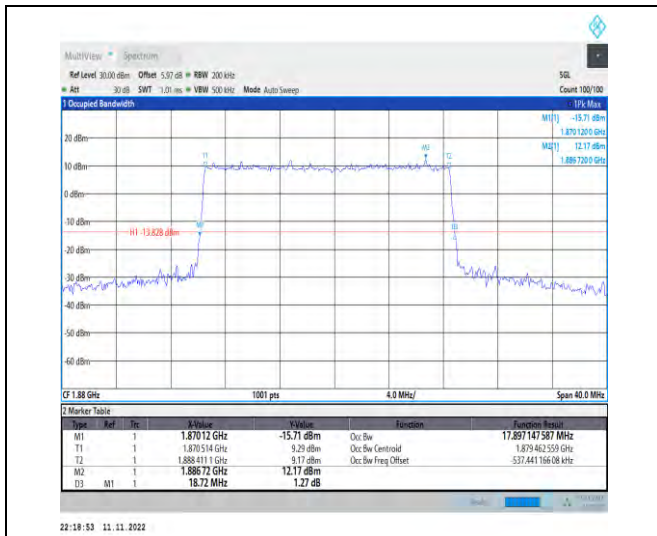
1-N2-PC3-15-20-M-3-DFT-16QAM-Outer_Full-100@ 0-Ant1-17.897-18.720-≤20-PASS
