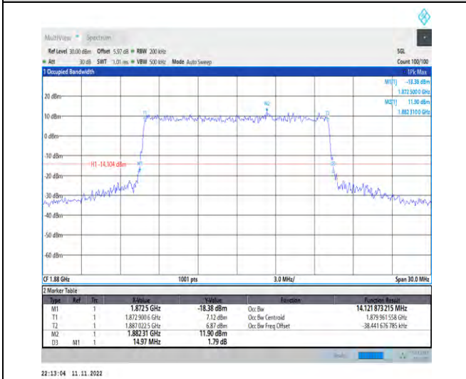
1-N2-PC3-15-15-M-8-CP-64QAM-Outer_Full-79@0-A Ant1-14.122-14.970-≤15-PASS
