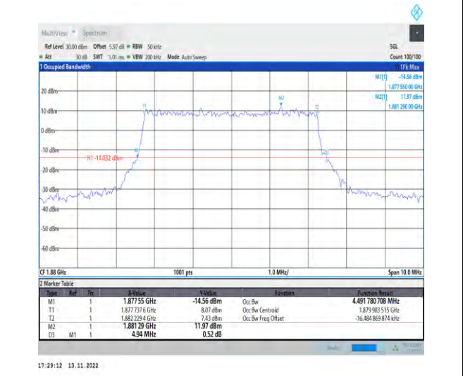
1-N2-PC3-15-5-M-3-DFT-16QAM-Outer_Full-25@0-Ant1-4.492-4.940-≤5-PASS
