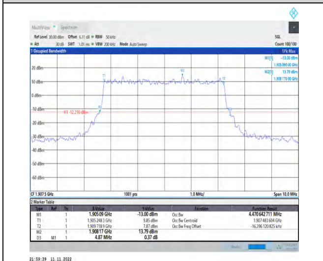
1-N2-PC3-15-5-H-1-DFT-QPSK-Outer_Full-25@0-A nt1-4.471-4.870-≤5-PASS
