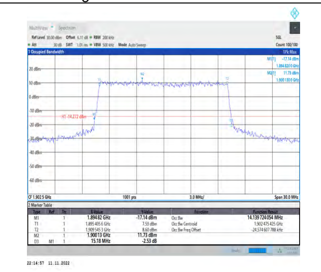
1-N2-PC3-15-15-H-6-CP-QPSK-Outer_Full-79@0-A nt1-14.14-15.180-≤15-PASS
