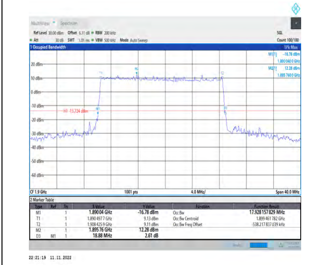
1-N2-PC3-15-20-H-4-DFT-64QAM-Outer_Full-100 @0-Ant1-17.928-18.880-≤20-PASS
