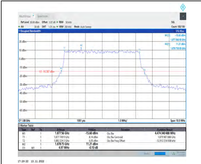
1-N2-PC3-15-5-M-4-DFT-64QAM-Outer_Full-25@0-Ant1-4.474-4.970-≤5-PASS
