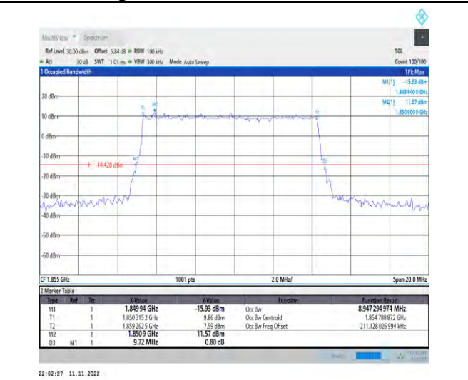
1-N2-PC3-15-10-L-3-DFT-16QAM-Outer_Full-50@0-Ant1-8.947-9.720-≤10-PASS
