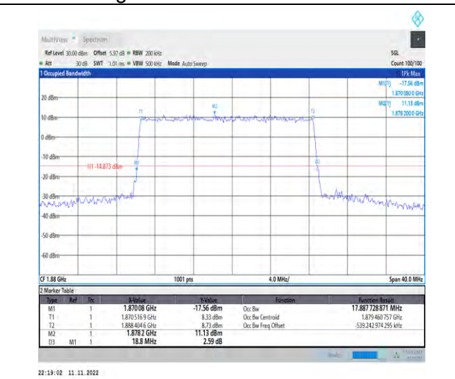
1-N2-PC3-15-20-M-4-DFT-64QAM-Outer_Full-100@ 0-Ant1-17.888-18.800-≤20-PASS
