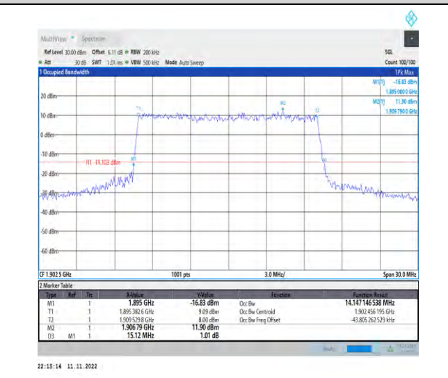
1-N2-PC3-15-15-H-8-CP-64QAM-Outer_Full-79@0- Ant1-14.147-15.120-≤15-PASS
