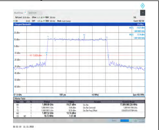
1-N2-PC3-15-20-H-3-DFT-16QAM-Outer_Full-100 @0-Ant1-17.895-18.720-≤20-PASS
