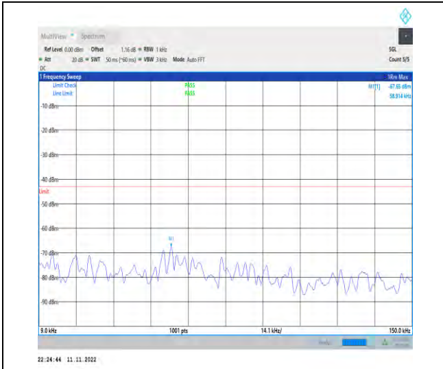
1-N2-PC3-15-20-H-1-DFT-PI2BPSK-Inner_1RB_Lef t-1@1-0.009-0.15-Ant1-0.06--67.65--43-PASS
