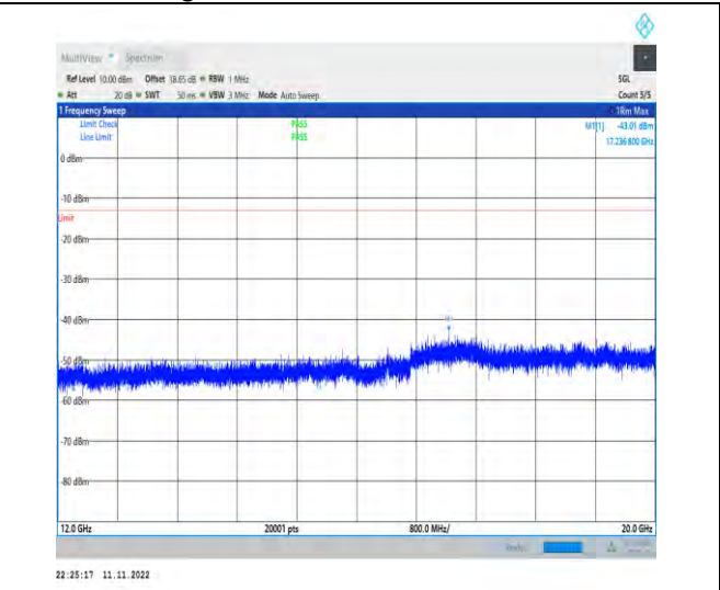
1-N2-PC3-15-20-H-1-DFT-PI2BPSK-Inner_1RB_Left- 1@1-12000-20000-Ant1-17236.80--43.01--13-PASS
