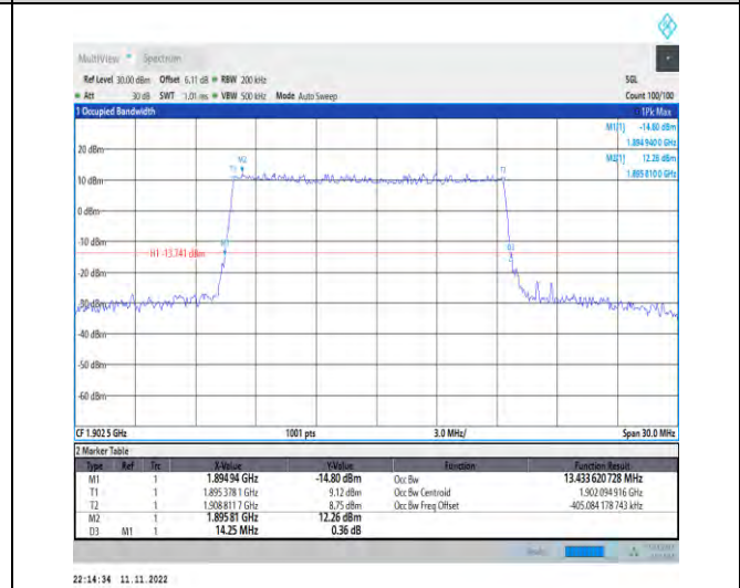
1-N2-PC3-15-15-H-4-DFT-64QAM-Outer_Full-75@0-Ant1-13.434-14.250-≤15-PASS
