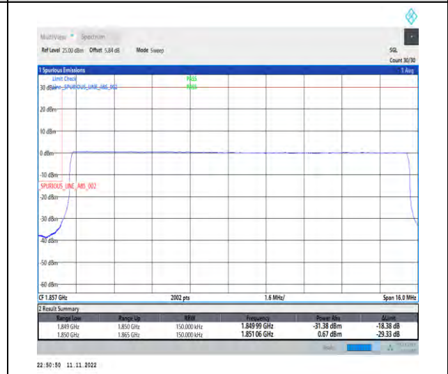
1-N2-PC3-15-15-L-6-CP-QPSK-Outer_Full-79@0-Ant1-1-seegraph-PASS-see graph
