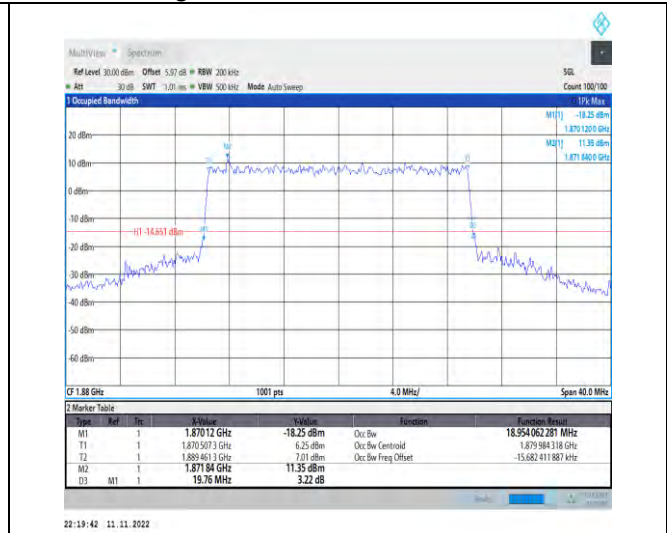
1-N2-PC3-15-20-M-8-CP-64QAM-Outer_Full-106@0 -Ant1-18.954-19.760-≤20-PASS
