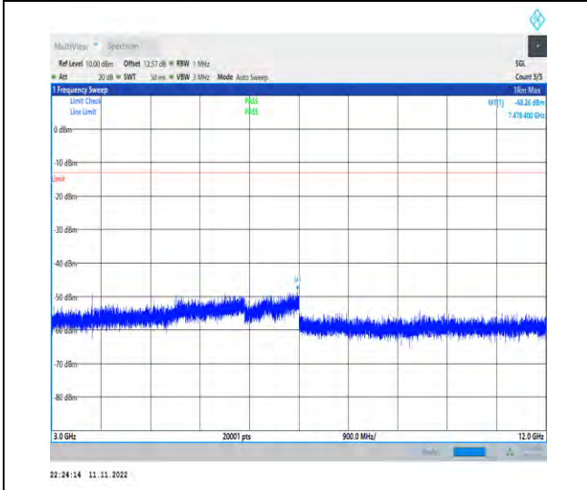
1-N2-PC3-15-20-M-1-DFT-PI2BPSK-Inner_1RB_Lef t-1@1-3000-12000-Ant1-7478.40--48.26--13-PASS
