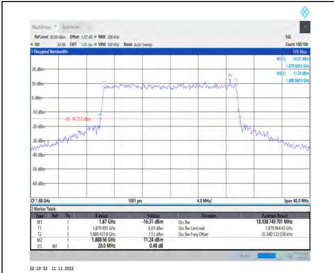
1-N2-PC3-15-20-M-7-CP-16QAM-Outer_Full-106@0 -Ant1-18.939-20.000-≤20-PASS
