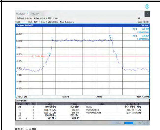
1-N2-PC3-15-5-H-2-DFT-PI2BPSK-Outer_Full-25@0- -Ant1-4.475-5.010-≤5-PASS
