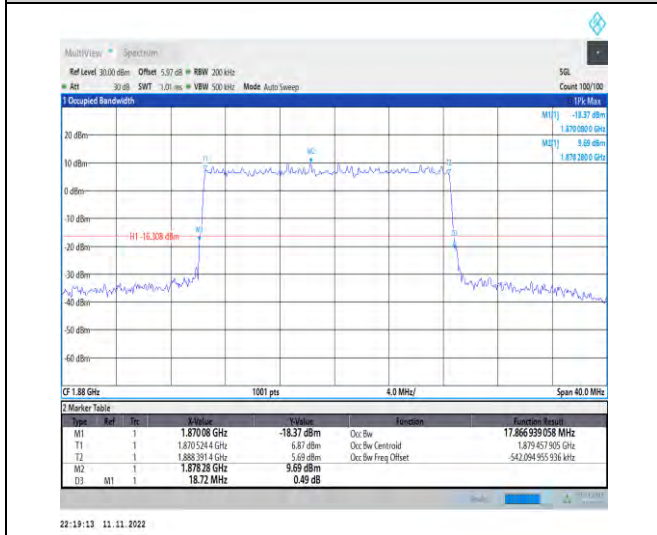
1-N2-PC3-15-20-M-5-DFT-256QAM-Outer_Full-100 @0-Ant1-17.867-18.720-≤20-PASS
