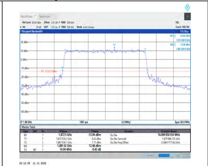
1-N2-PC3-15-15-M-7-CP-16QAM-Outer_Full-79@0-A Ant1-14.1-14.940-≤15-PASS
