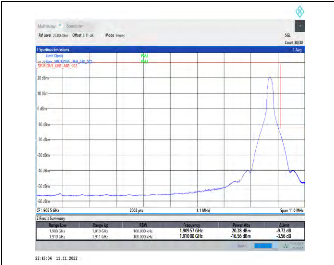
1-N2-PC3-15-10-H-2-DFT-PI2BPSK-Edge_1RB_Right-1@51-Ant1-1-seegraph-PASS-see graph
