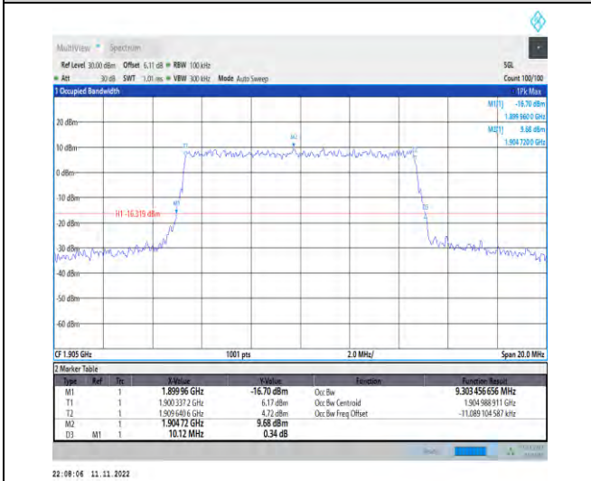
1-N2-PC3-15-10-H-6-CP-QPSK-Outer_Full-52@0-A nt1-9.303-10.120-≤10-PASS
