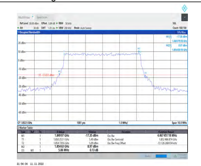
1-N2-PC3-15-5-L-6-CP-QPSK-Outer_Full-25@0-Ant1-4.467-5.060-≤5-PASS
