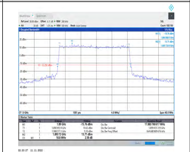
1-N2-PC3-15-20-H-1-DFT-QPSK-Outer_Full-100@0- Ant1-17.884-18.800-≤20-PASS
