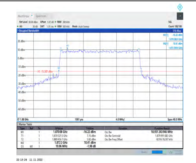
1-N2-PC3-15-20-M-6-CP-QPSK-Outer_Full-106@0- Ant1-18.931-19.960-≤20-PASS
