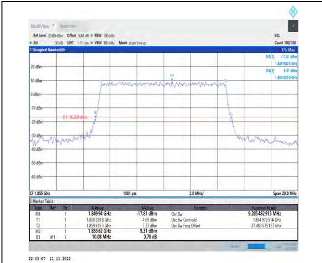
1-N2-PC3-15-10-L-6-CP-QPSK-Outer_Full-52@0-A nt1-9.285-10.080-≤10-PASS
