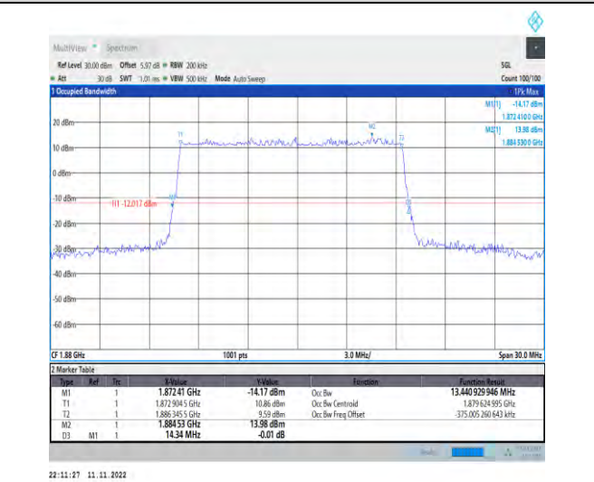
1-N2-PC3-15-15-M-1-DFT-QPSK-Outer_Full-75@0-Ant1-13.441-14.340-≤15-PASS
