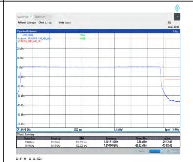
1-N2-PC3-15-10-H-6-CP-QPSK-Outer_Full-52@0-Ant1-1-seegraph-PASS-see graph
