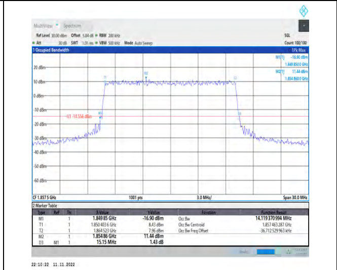
1-N2-PC3-15-15-L-6-CP-QPSK-Outer_Full-79@0-Ant1-14.119-15.150-≤15-PASS
