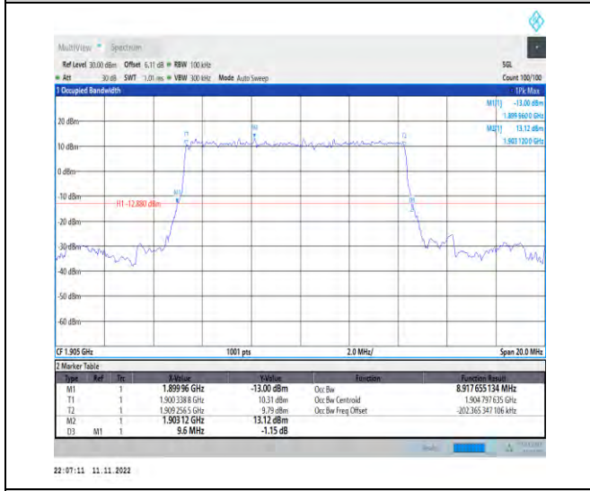
1-N2-PC3-15-10-H-2-DFT-PI2BPSK-Outer_Full-50@0- Ant1-8.918-9.600-≤10-PASS
