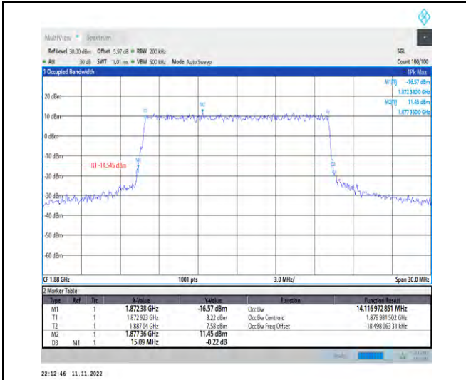
1-N2-PC3-15-15-M-6-CP-QPSK-Outer_Full-79@0-A Ant1-14.117-15.090-≤15-PASS
