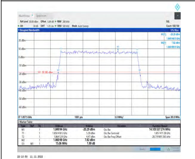
1-N2-PC3-15-15-L-9-CP-256QAM-Outer_Full-79@0-Ant1-14.106-15.060-≤15-PASS
