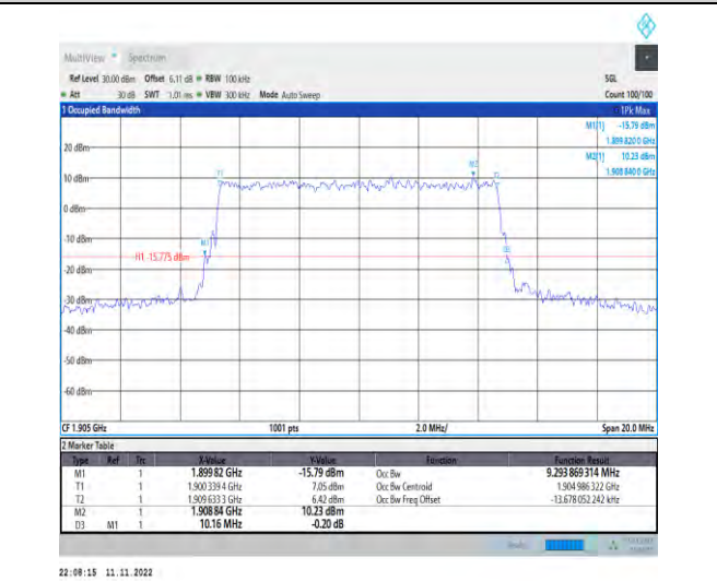
1-N2-PC3-15-10-H-7-CP-16QAM-Outer_Full-52@0- Ant1-9.294-10.160-≤10-PASS
