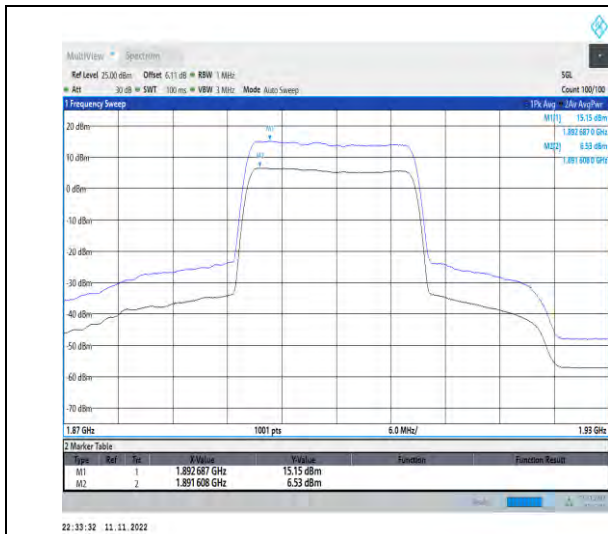
1-N2-PC3-15-20-H-1-DFT-256QAM-Outer_Full-100 @0-Ant1-8.62-100%-0.00-8.62-PASS-≤13
