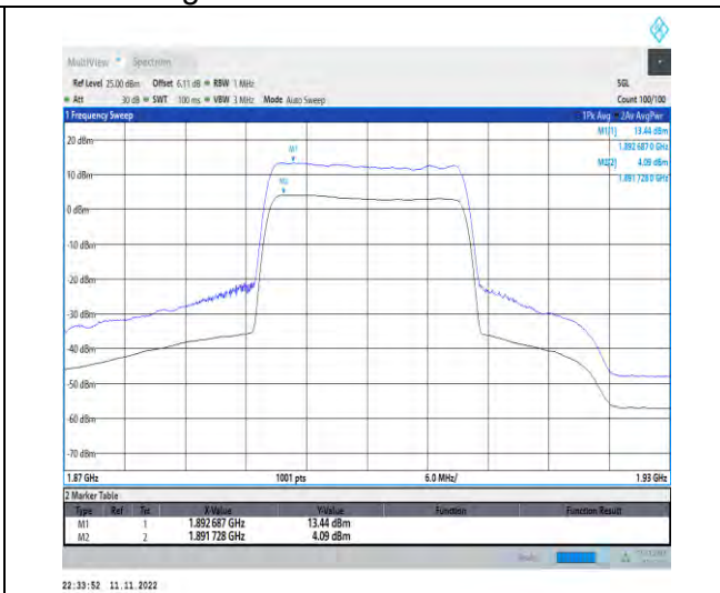
1-N2-PC3-15-20-H-2-CP-256QAM-Outer_Full-106 @0-Ant1-9.35-100%-0.00-9.35-PASS-≤13
