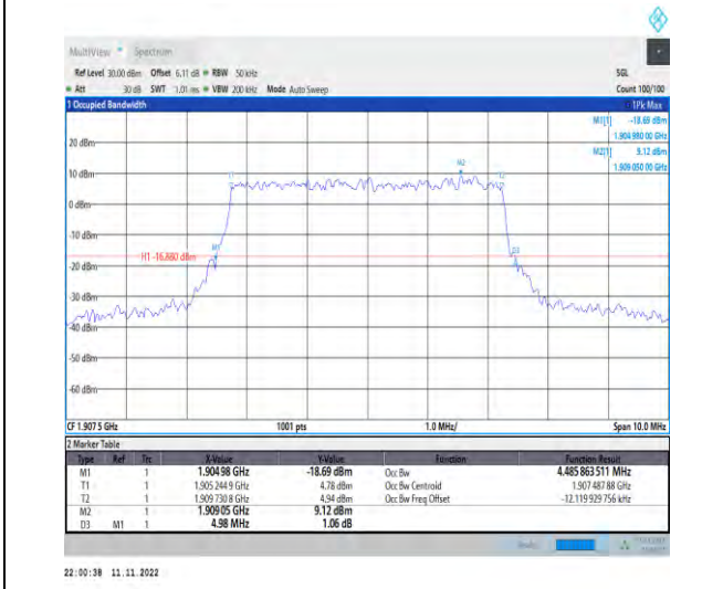
1-N2-PC3-15-5-H-5-DFT-256QAM-Outer_Full-25@0-Ant1-4.486-4.980-≤5-PASS
