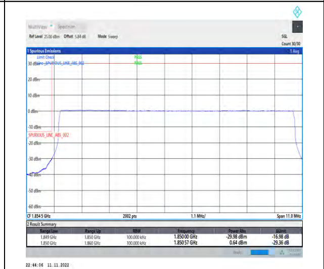
1-N2-PC3-15-10-L-6-CP-QPSK-Outer_Full-52@0-Ant1-1-seegraph-PASS-see graph
