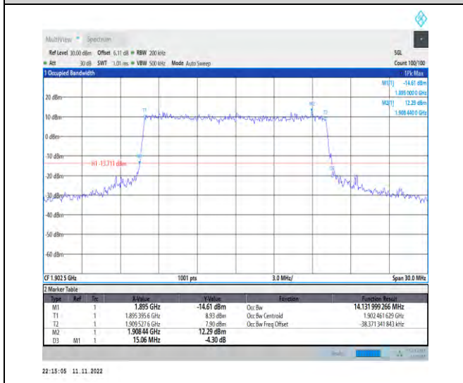
1-N2-PC3-15-15-H-7-CP-16QAM-Outer_Full-79@0- Ant1-14.132-15.060-≤15-PASS
