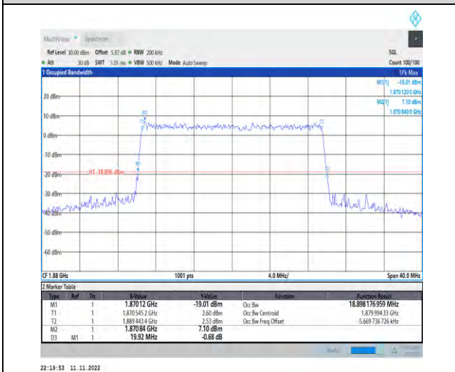
1-N2-PC3-15-20-M-9-CP-256QAM-Outer_Full-106@0 0-Ant1-18.898-19.920-≤20-PASS
