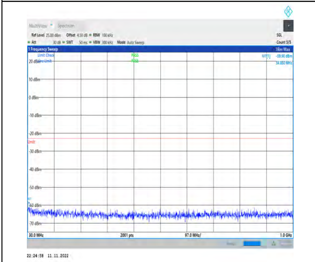
1-N2-PC3-15-20-H-1-DFT-PI2BPSK-Inner_1RB_Lef t-1@1-30-1000-Ant1-34.85--59.90--23-PASS
