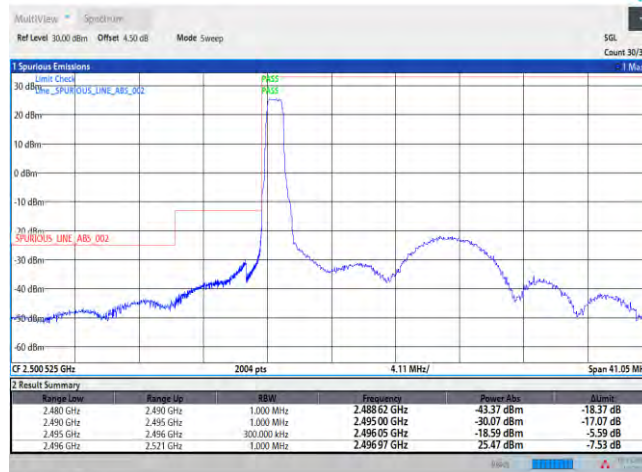
41-41-10MHz-15MHz-QPSK-QPSK-39703-39823-50RB#0-75RB#0
