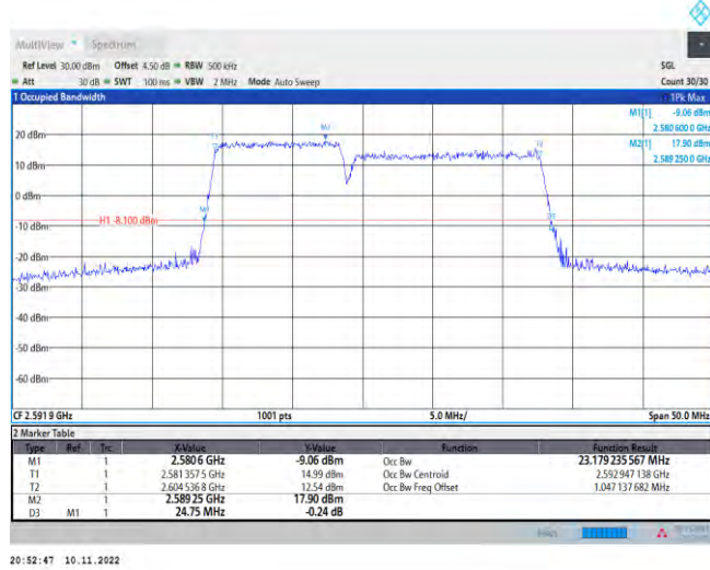
41-41-10MHz-15MHz-QPSK-QPSK-40549-40669-50RB#0-75RB#0
