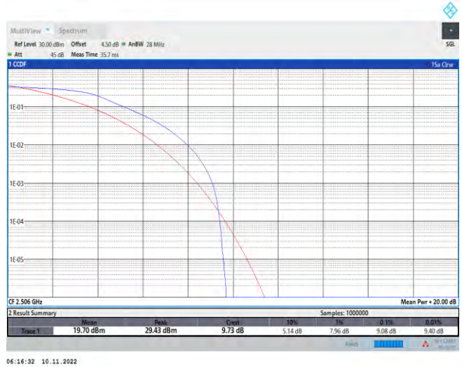
Band41-20MHz-QPSK-40620-100RB#0
