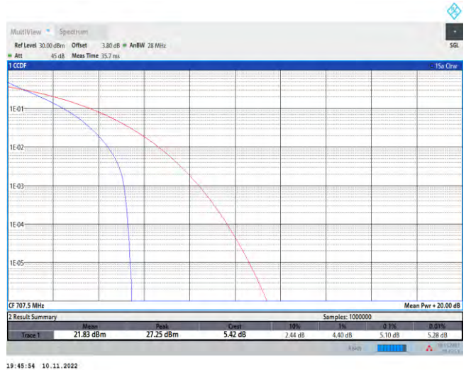
Band12-10MHz-QPSK-23095-50RB#0
