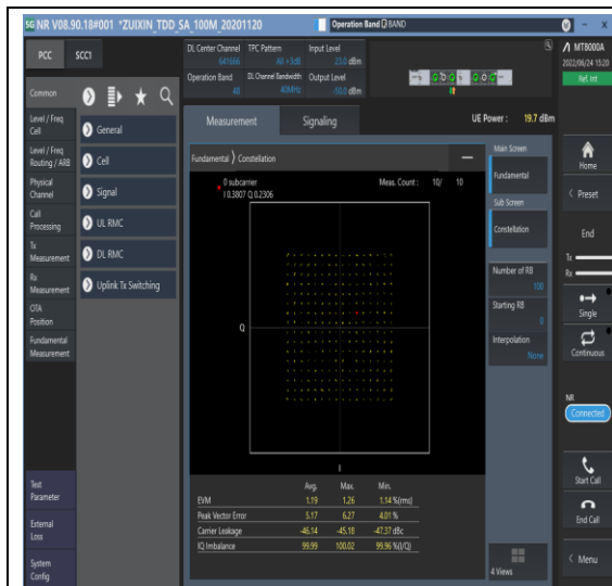
1-N48-PC3-30-40-M-5-DFT-256QAM-Outer_Full-100@0-Ant1-see graph-PASS
