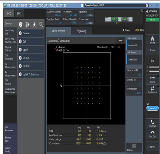
1-N48-PC3-30-40-M-8-CP-64QAM-Outer_Ful-I-106@0-Ant1-see graph-PASS
