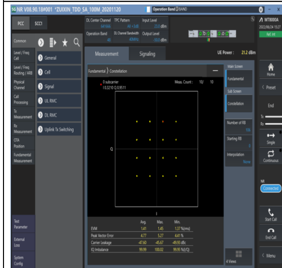
1-N48-PC3-30-40-M-7-CP-16QAM-Outer_Ful-I-106@0-Ant1-see graph-PASS
