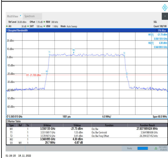
1-N48-PC2-30-30-L-9-CP-256QAM-Outer_F ull-78@0-Ant1-27.838-29.700-≤30-PASS
