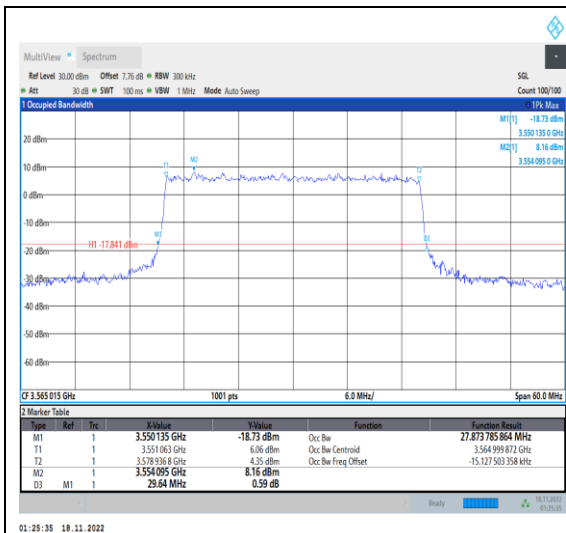
1-N48-PC2-30-30-L-7-CP-16QAM-Outer_Full -78@0-Ant1-27.874-29.640-≤30-PASS
