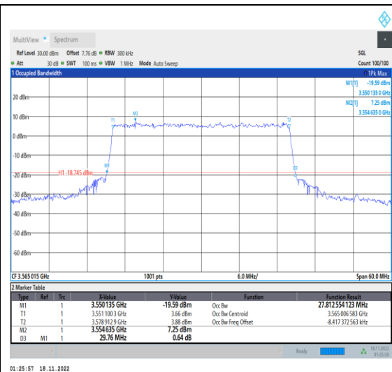
1-N48-PC2-30-30-L-8-CP-64QAM-Outer_Full -78@0-Ant1-27.813-29.760-≤30-PASS
