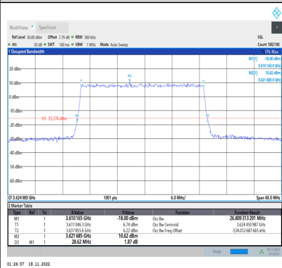
1-N48-PC2-30-30-M-1-DFT-QPSK-Outer_Ful l-75@0-Ant1-26.809-28.620-≤30-PASS
