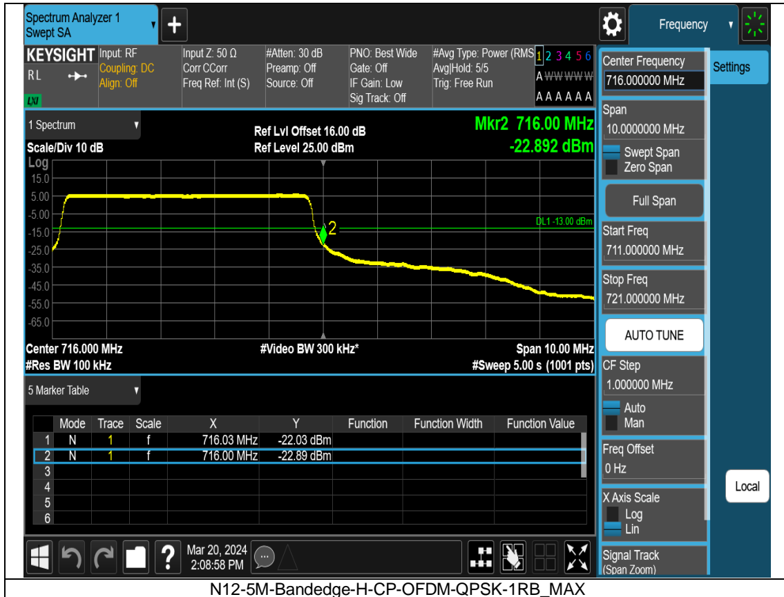
N12-5M-Bandedge-H-CP-OFDM-QPSK-1RB_MAX
