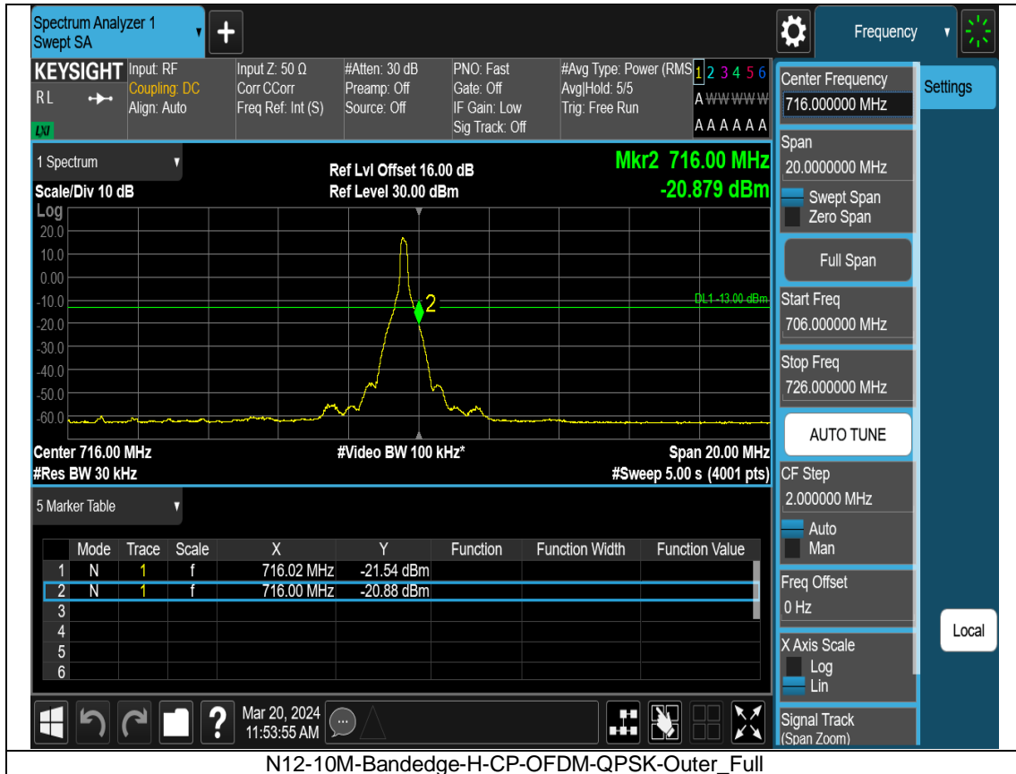
N12-10M-Bandedge-H-CP-OFDM-QPSK-Outer_Full
