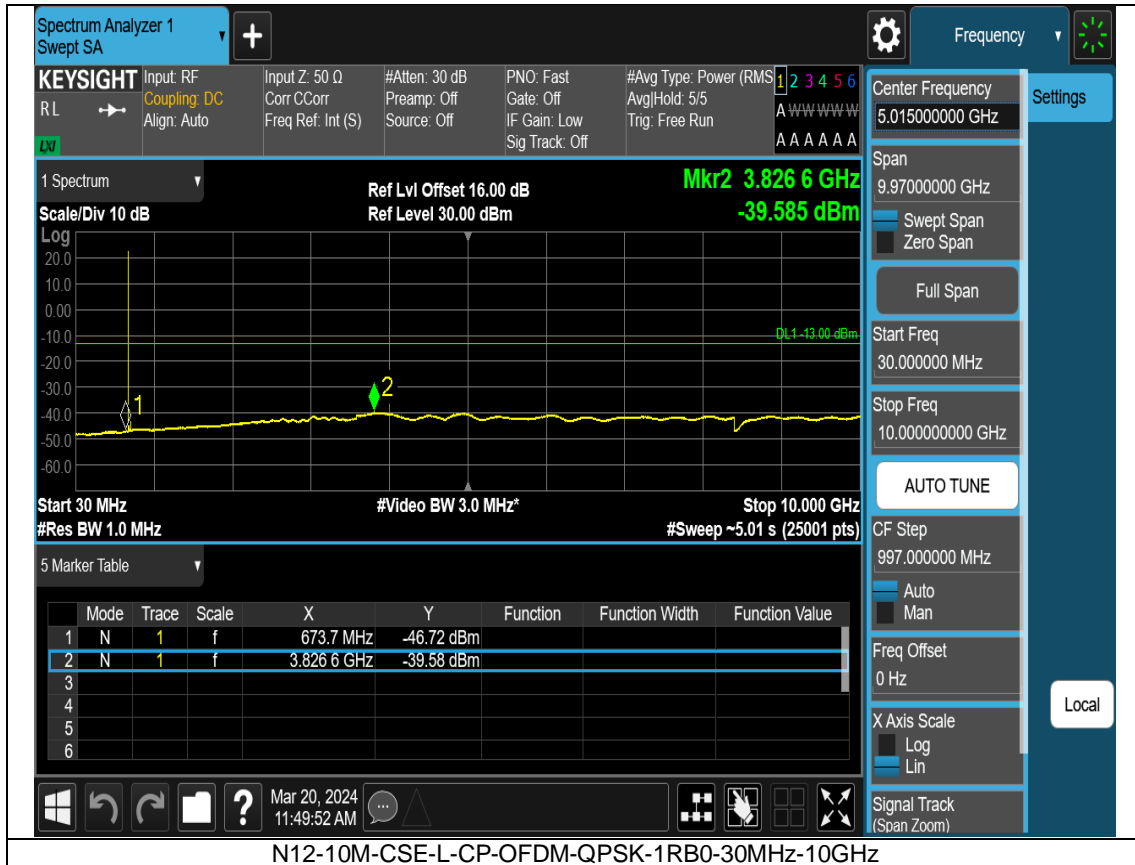
N12-10M-CSE-L-CP-OFDM-QPSK-1RB0-30MHz-10GHz
