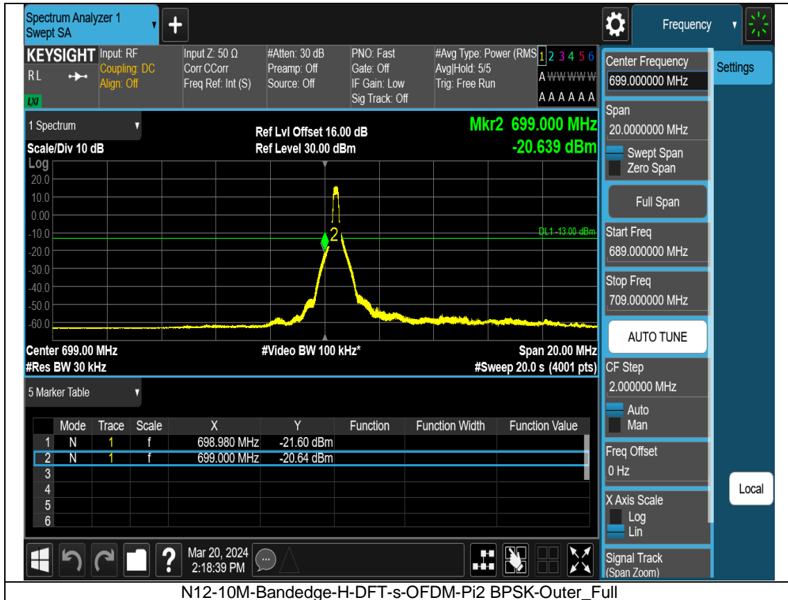
N12-10M-Bandedge-H-DFT-s-OFDM-Pi2 BPSK-Outer_Full
