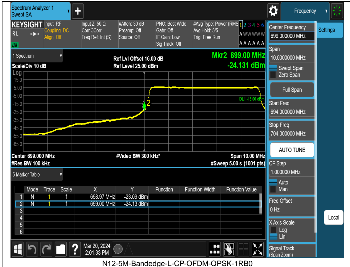
N12-5M-Bandedge-L-CP-OFDM-QPSK-1RB0
