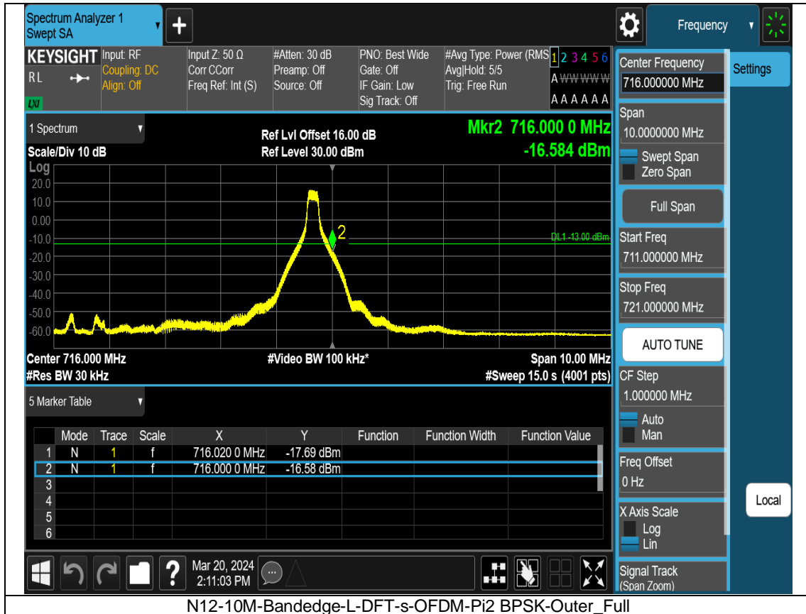
N12-10M-Bandedge-L-DFT-s-OFDM-Pi2 BPSK-Outer_Full
