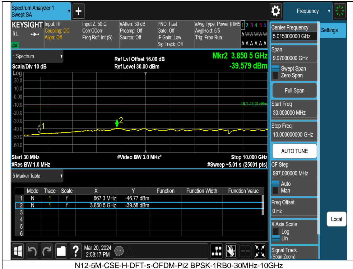
N12-5M-CSE-H-DFT-s-OFDM-Pi2 BPSK-1RB0-30MHz-10GHz
