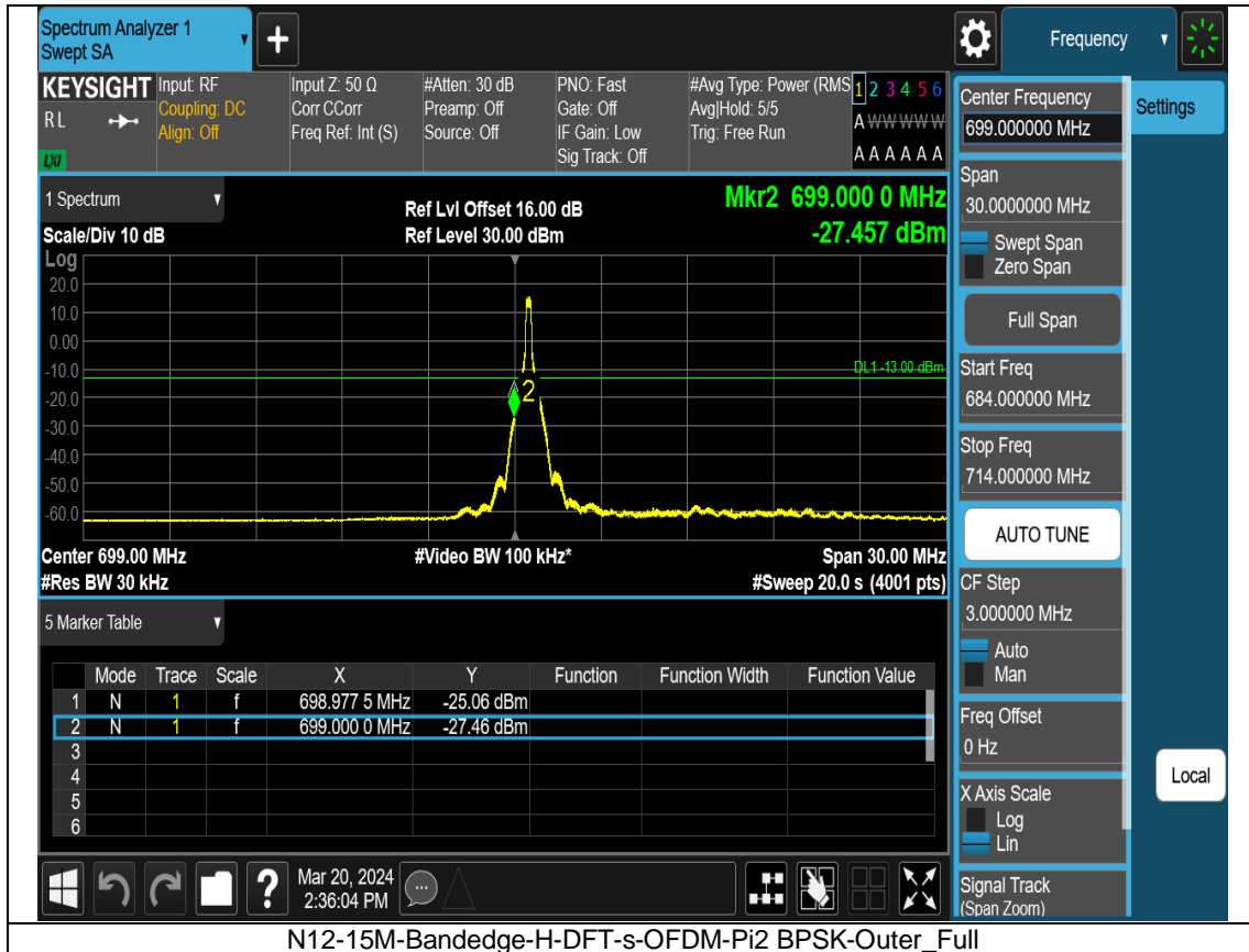
N12-15M-Bandedge-H-DFT-s-OFDM-Pi2 BPSK-Outer_Full
