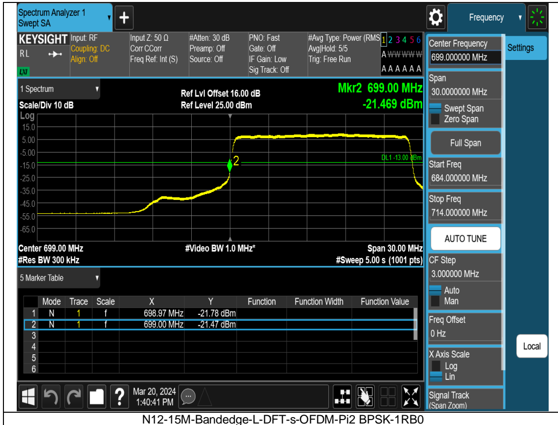
N12-15M-Bandedge-L-DFT-s-OFDM-Pi2 BPSK-1RB0
