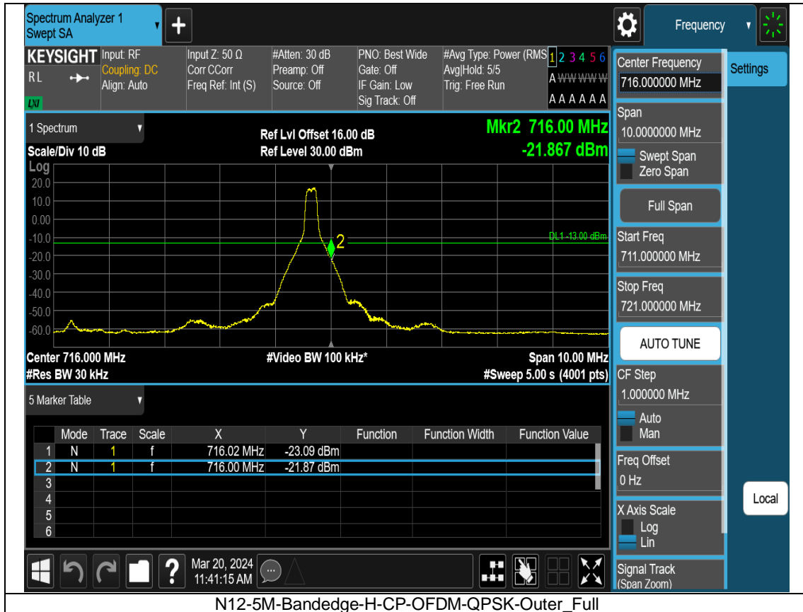
N12-5M-Bandedge-H-CP-OFDM-QPSK-Outer_Full
