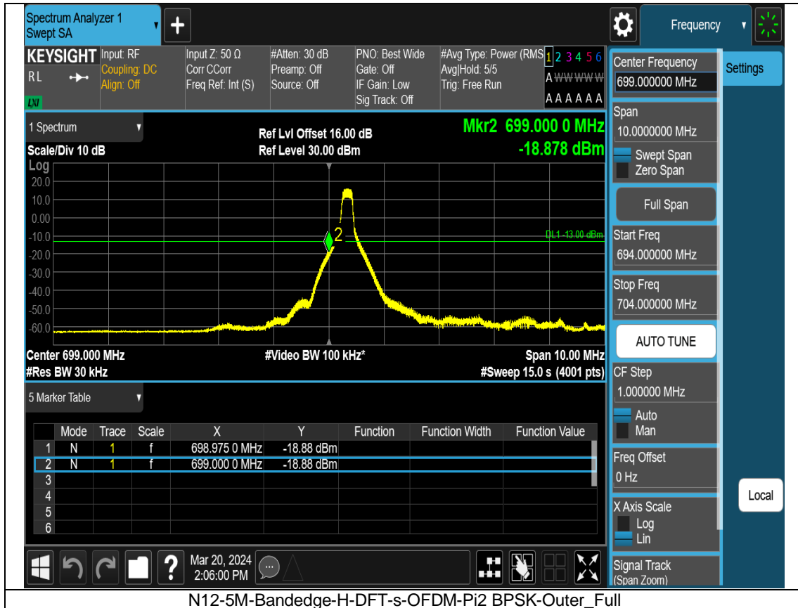
N12-5M-Bandedge-H-DFT-s-OFDM-Pi2 BPSK-Outer_Full
