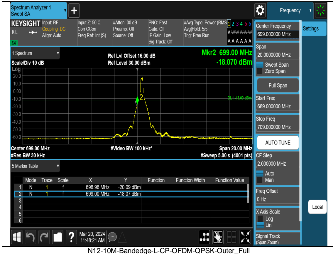
N12-10M-Bandedge-L-CP-OFDM-QPSK-Outer_Full
