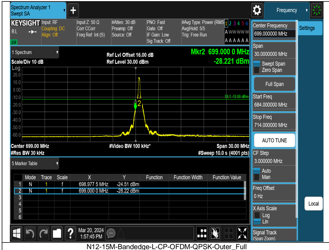
N12-15M-Bandedge-L-CP-OFDM-QPSK-Outer_Full
