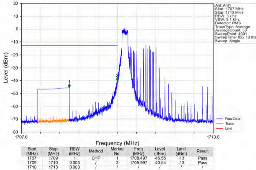
Band66_3MHz_64QAM_LCH_1711.5MHz_RB_1_0_NTNV
