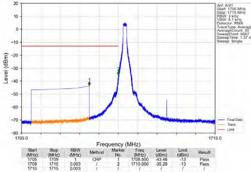
Band66_5MHz_64QAM_LCH_1712.5MHz_RB_1_0_NTNV
