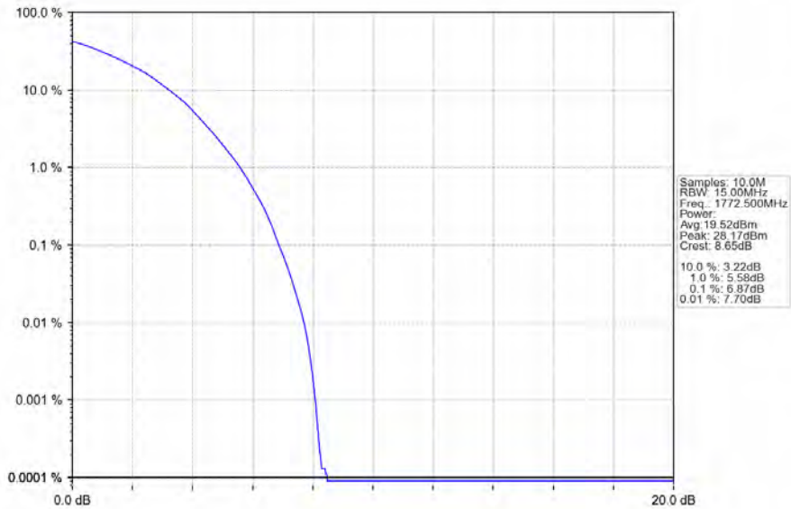
Band66_15MHz_64QAM_HCH_1772.5MHz_RB_75_0_NTNV
