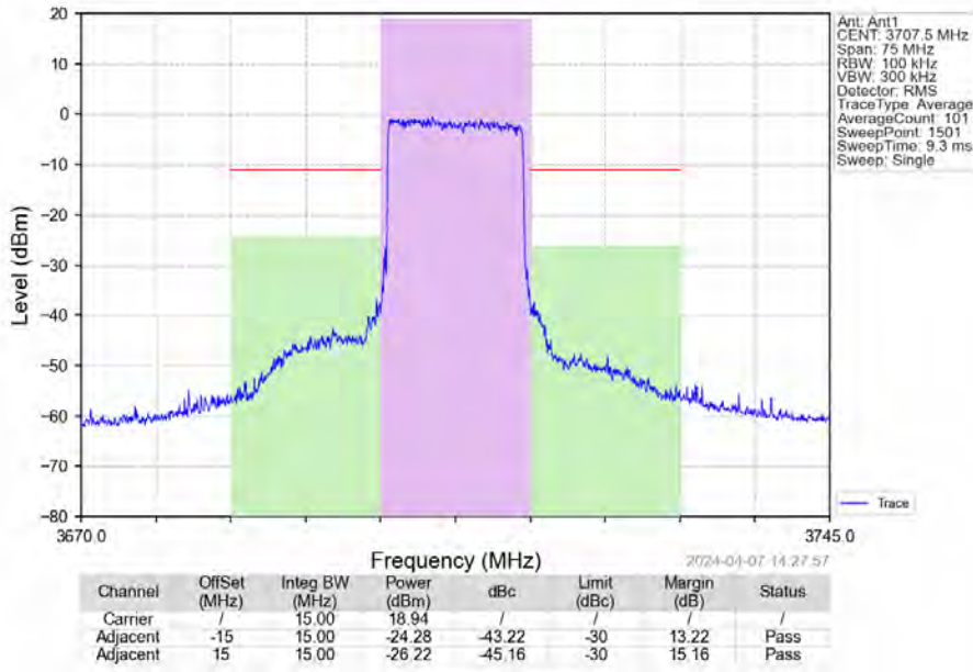
Band43d_15MHz_64QAM_LCH_3707.5MHz_RB_75_0_NTNV
