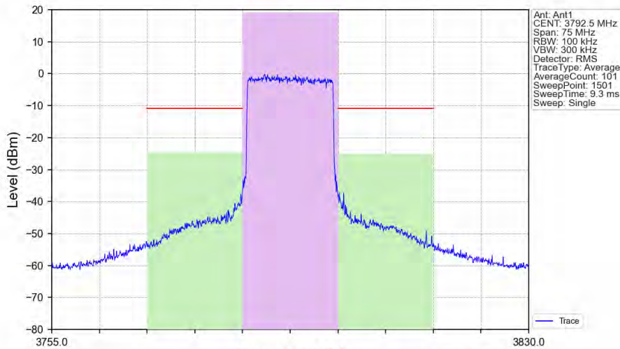
Band43d 15MHz 64QAM HCH 3792.5MHz RB 75_0 NTV
