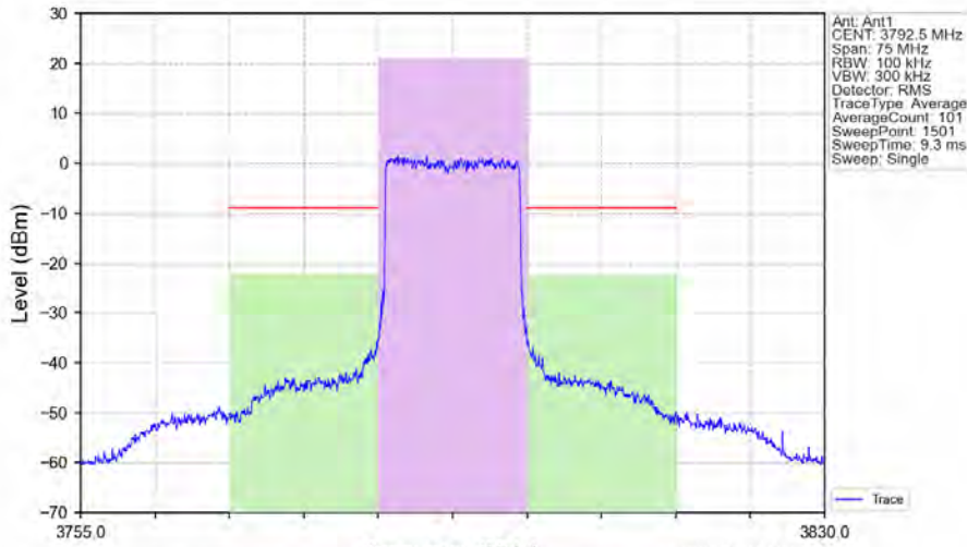
Band43d_15MHz_QPSK_HCH_3792.5MHz_RB_75_0_NTNV
