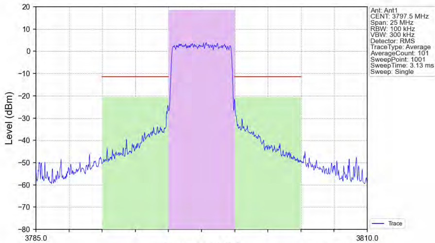
Band43d_5MHz_64QAM_HCH_3797.5MHz_RB_25_0_NTNV
