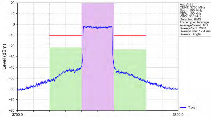
Band43d 20MHz 16QAM MCH 3750MHz RB 100 0 NTN
