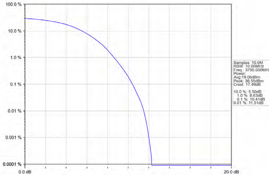
Band43d_10MHz_64QAM_HCH_3795MHz_RB_50_0_NTNV
