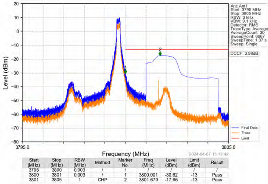
Band43d_5MHz_16QAM_HCH_3797.5MHz_RB_1_24_NTNV
