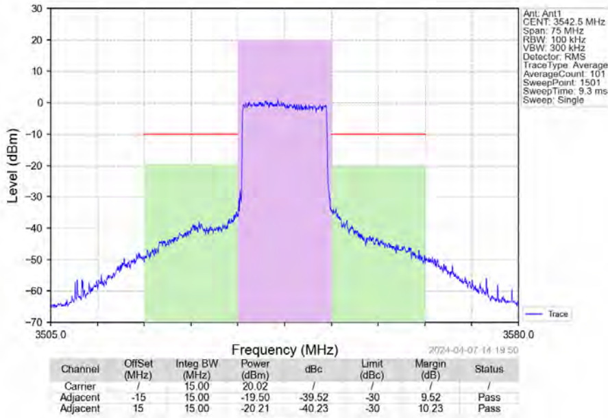
Band42a_15MHz_QPSK_HCH_3542.5MHz_RB_75_0_NTNV
