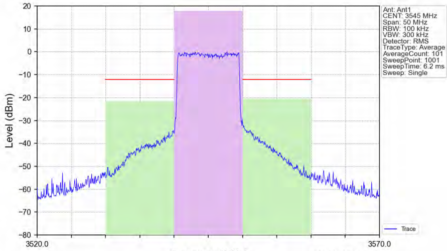
Band42a_10MHz_64QAM_HCH_3545MHz_RB_50_0_NTNV
