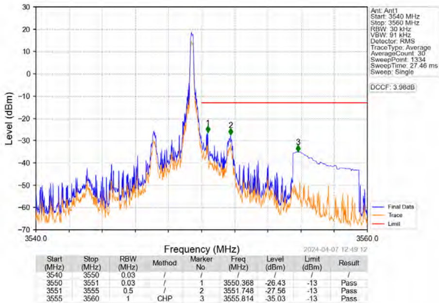
Band42a_10MHz_16QAM_HCH_3545MHz_RB_1_49_NTNV
