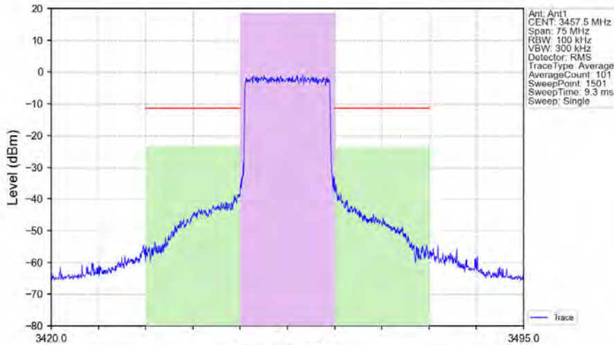
Band42a_15MHz_64QAM_LCH_3457.5MHz_RB_75_0_NTNV
