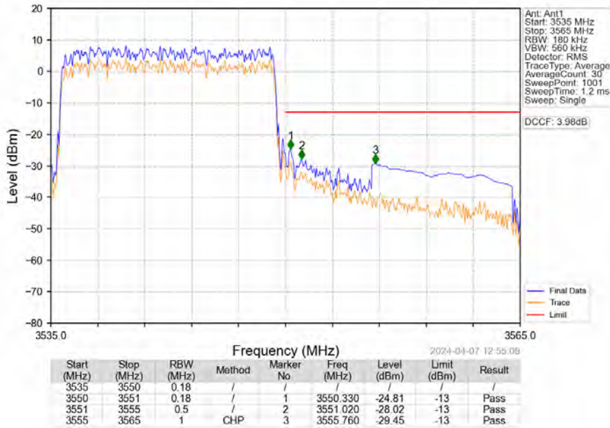
Band42a_15MHz_QPSK_HCH_3542.5MHz_RB_75_0_NTNV
