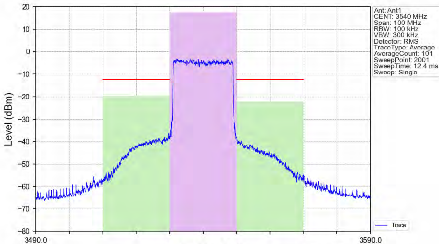
Band42a_20MHz_64QAM_HCH_3540MHz_RB_100_0_NTNV
