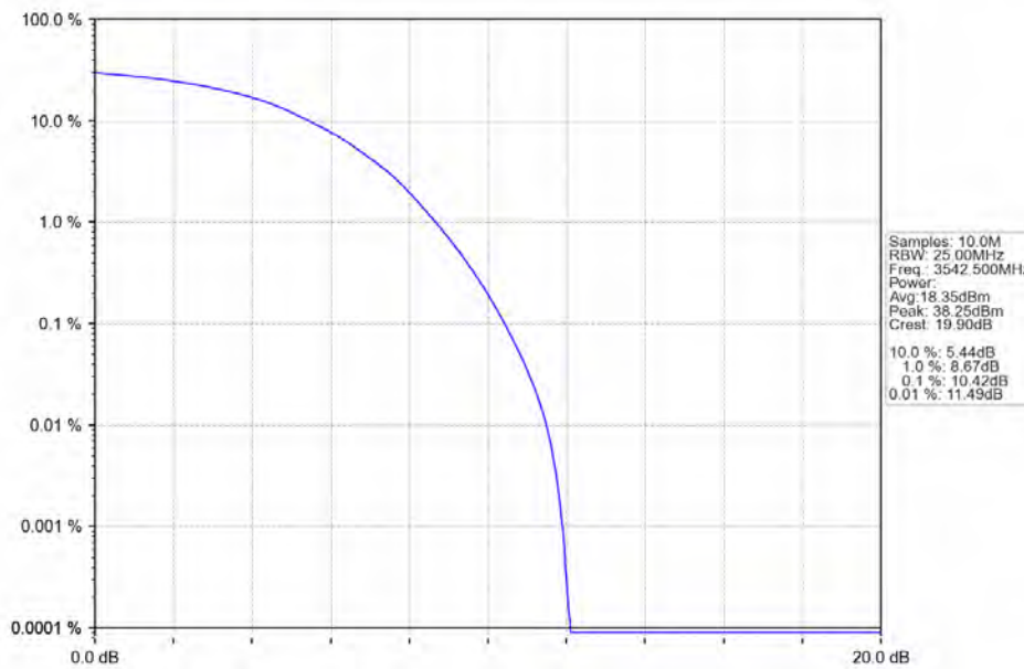
Band42a 15MHz 64QAM HCH 3542.5MHz RB 75_0 NTV
