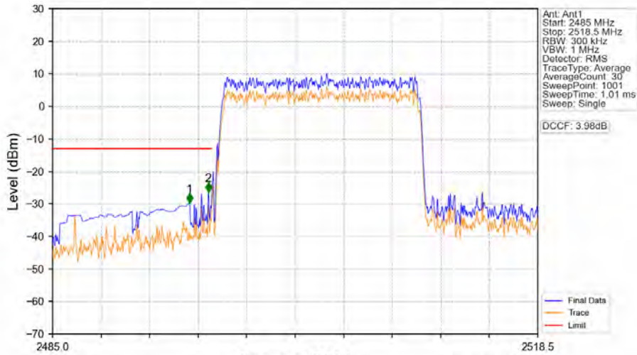
Band41_15MHz_64QAM_LCH_2503.5MHz_RB_75_0_NTNV
