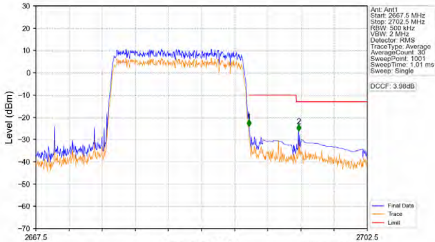
Band41_15MHz_64QAM_HCH_2682.5MHz_RB_75_0_NTNV
