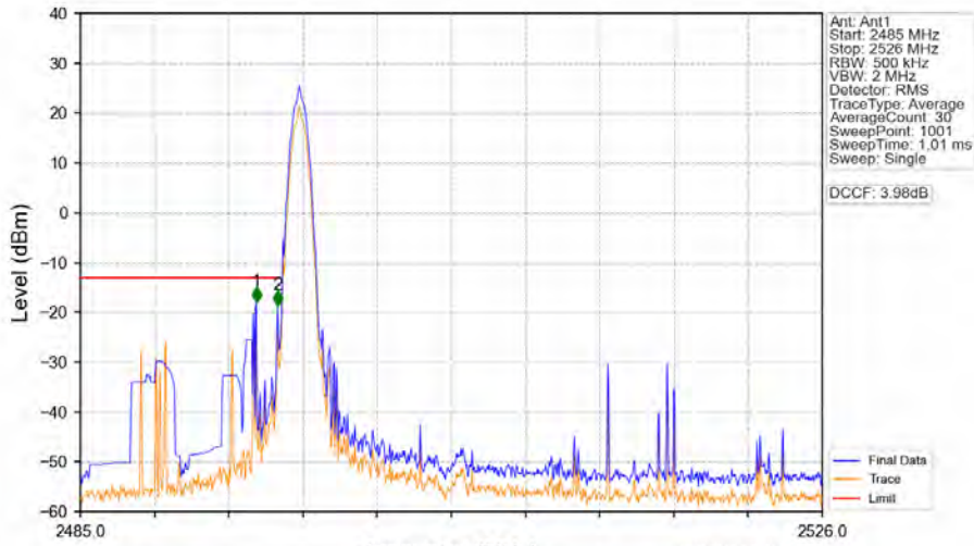
Band41_20MHz_64QAM_LCH_2506MHz_RB_1_0_NTNV
