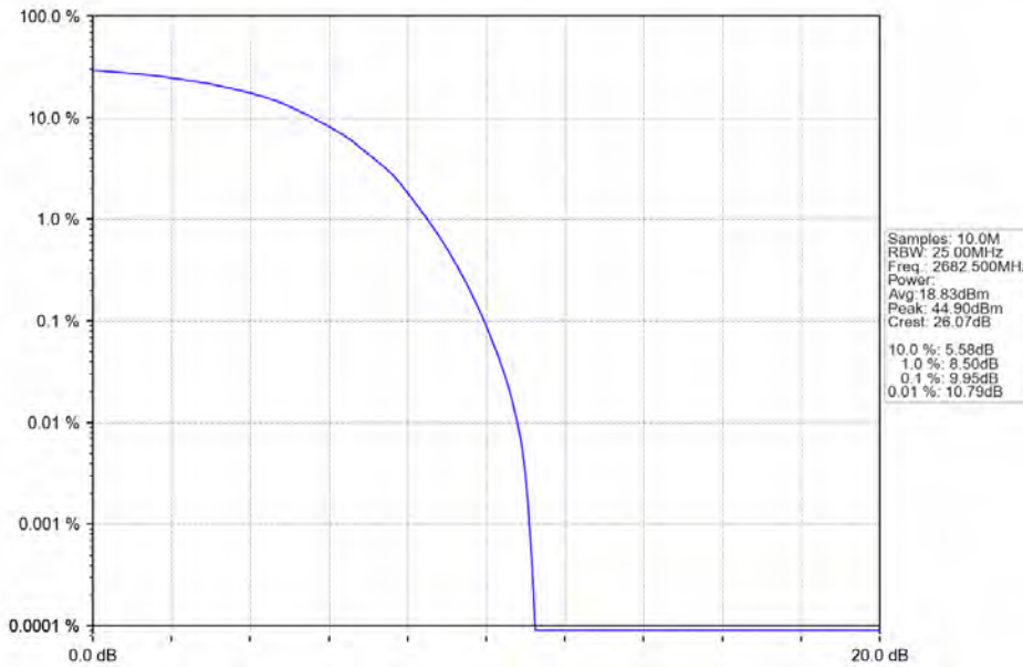
Band41_15MHz_64QAM_HCH_2682.5MHz_RB_75_0_NTNV
