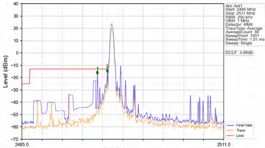
Band41_10MHz_64QAM_LCH_2501MHz_RB_1_0_NTNV
