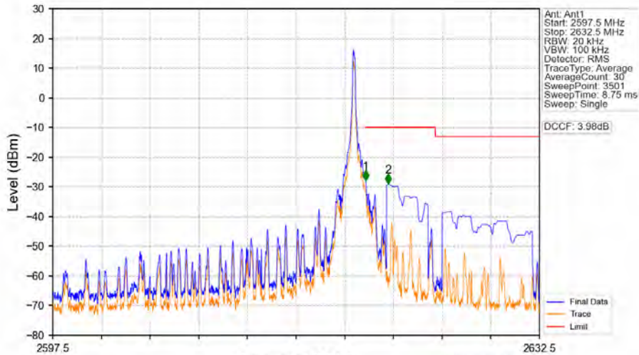
Band38_15MHz_16QAM_HCH_2612.5MHz_RB_1_74_NTNV
