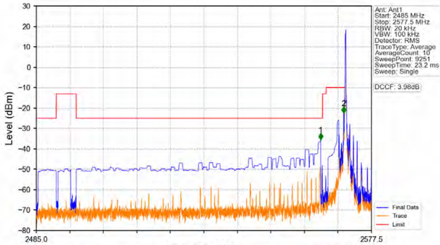
Band38_5MHz_64QAM_LCH_2572.5MHz_RB_1_0_NTNV
