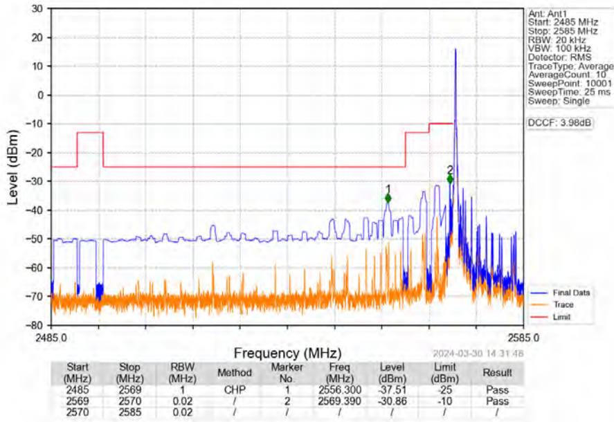
Band38_10MHz_64QAM_LCH_2575MHz_RB_1_0_NTNV
