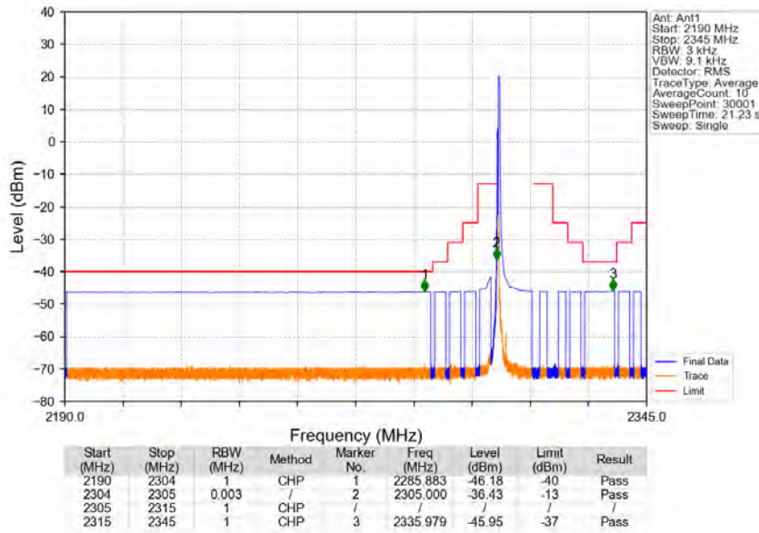
Band30_5MHz_64QAM_LCH_2307.5MHz_RB_1_0_NTNV
