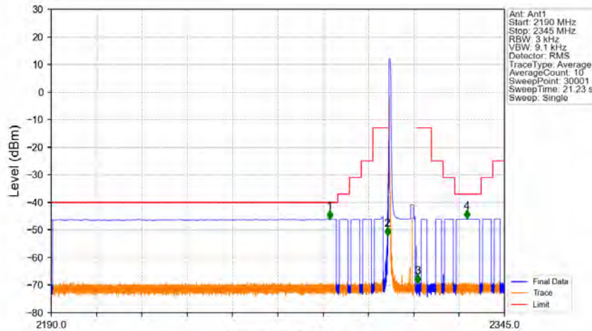
Band30_10MHz_64QAM_MCH_2310MHz_RB_1_0_NTNV
