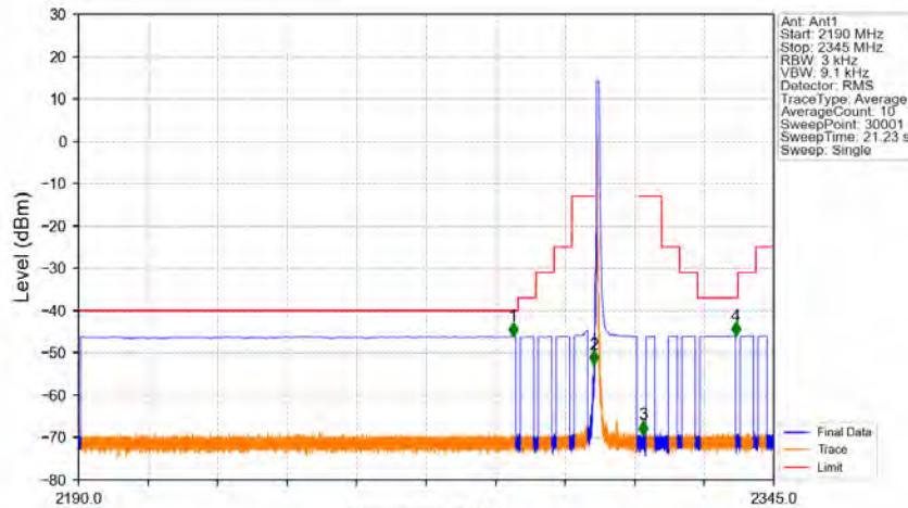
Band30_10MHz_64QAM_LCH_2310MHz_RB_1_0_NTNV
