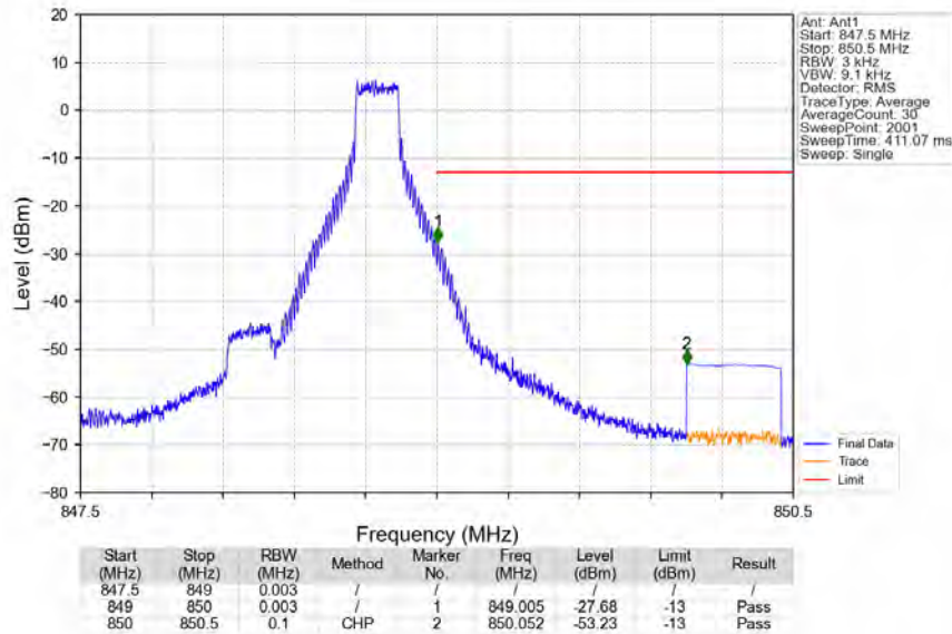
Band26b_1.4MHz_16QAM_HCH_848.3MHz_RB_1_5_NTNV
