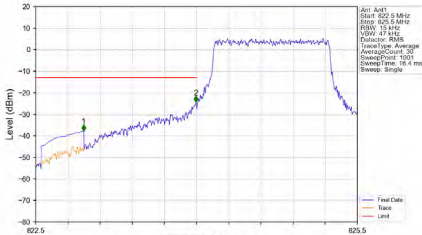
Band26b_1.4MHz_QPSK_LCH_824.7MHz_RB_6_0_NTNV
