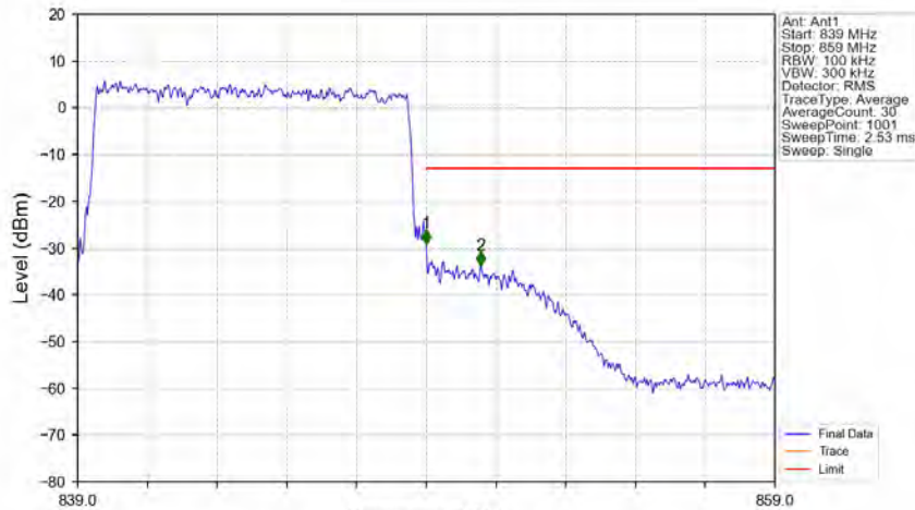
Band26b_10MHz_QPSK_HCH_844MHz_RB_50_0_NTNV
