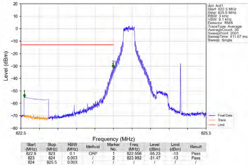
Band26b 1.4MHz 64QAM LCH 824.7MHz RB 1 0 NTV
