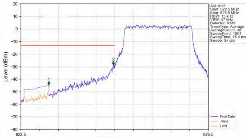
Band26b 1.4MHz 64QAM LCH 824.7MHz RB 6 0 NTV
