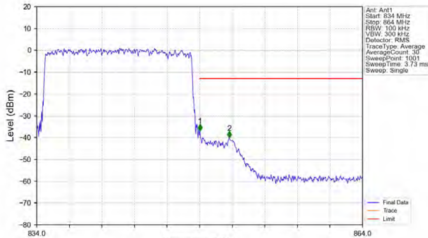
Band26c_15MHz_64QAM_HCH_841.5MHz_RB_75_0_NTNV
