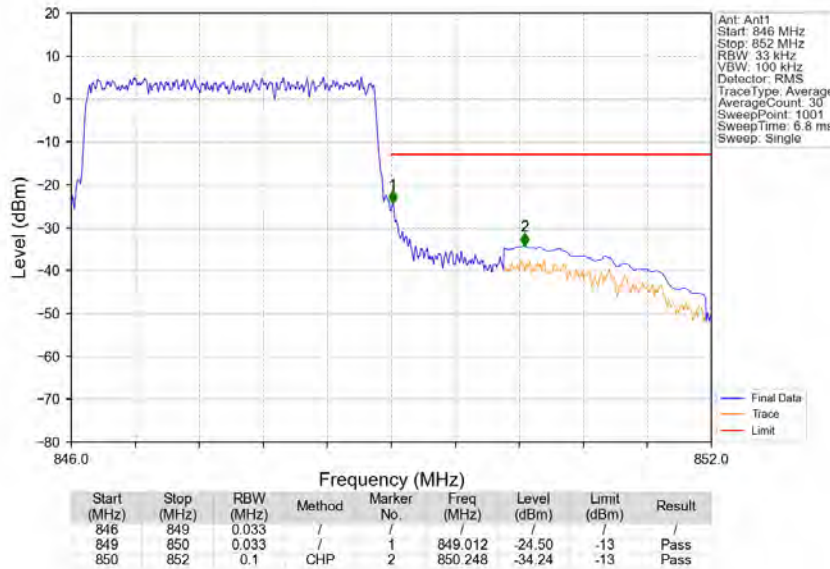
Band26b 3MHz QPSK HCH 847.5MHz RB 15 0 NTV
