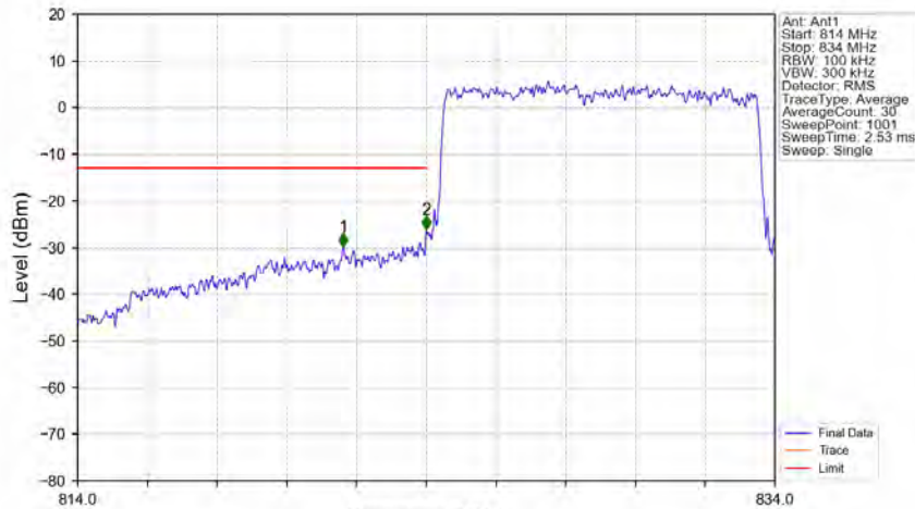
Band26b_10MHz_QPSK_LCH_829MHz_RB_50_0_NTNV
