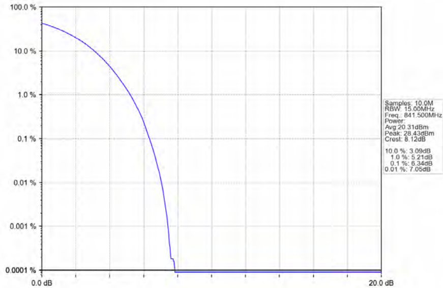
Band26c_15MHz_64QAM_HCH_841.5MHz_RB_75_0_NTNV
