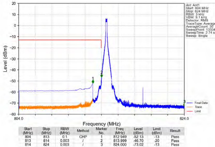
Band26a_10MHz_16QAM_LCH_819MHz_RB_1_0_NTNV
