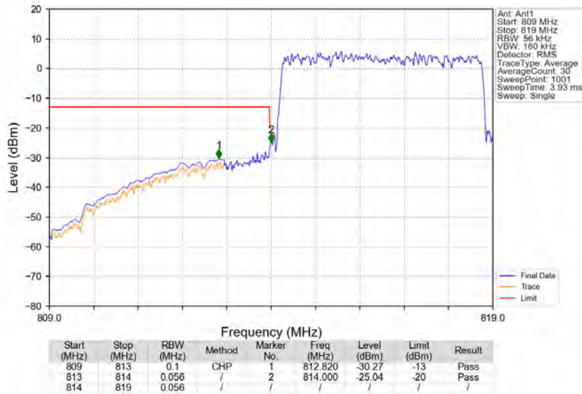
Band26a_5MHz_QPSK_LCH_816.5MHz_RB_25_0_NTNV
