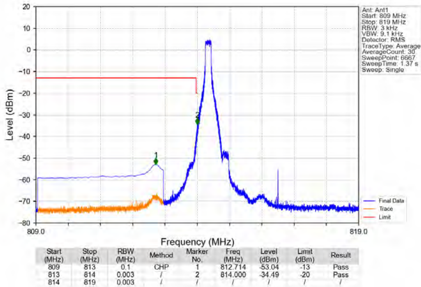
Band26a_5MHz_64QAM_LCH_816.5MHz_RB_1_0_NTNV
