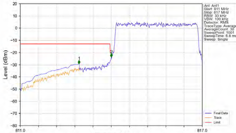
Band26a_3MHz_QPSK_LCH_815.5MHz_RB_15_0_NTNV
