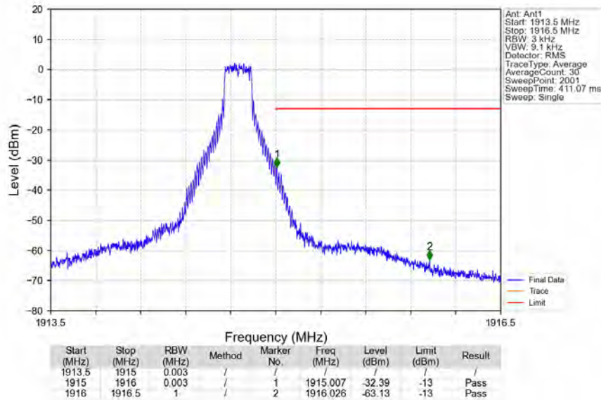
Band25_1.4MHz_64QAM_HCH_1914.3MHz_RB_1_5_NTNV
