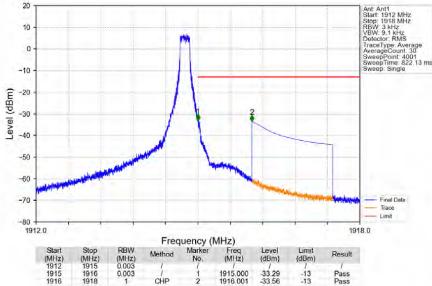
Band25_3MHz_QPSK_HCH_1913.5MHz_RB_1_14_NTNV
