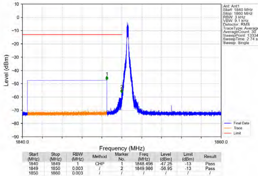
Band25_10MHz_64QAM_LCH_1855MHz_RB_1_0_NTNV
