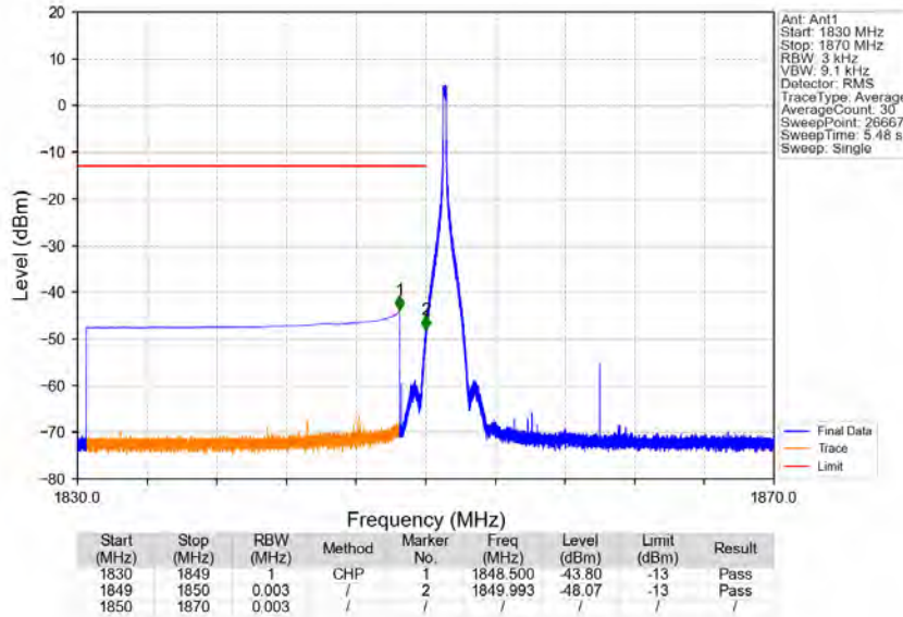
Band25_20MHz_64QAM_LCH_1860MHz_RB_1_0_NTNV
