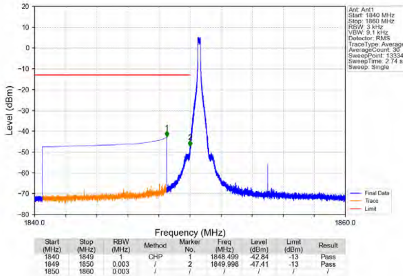
Band25_10MHz_16QAM_LCH_1855MHz_RB_1_0_NTNV
