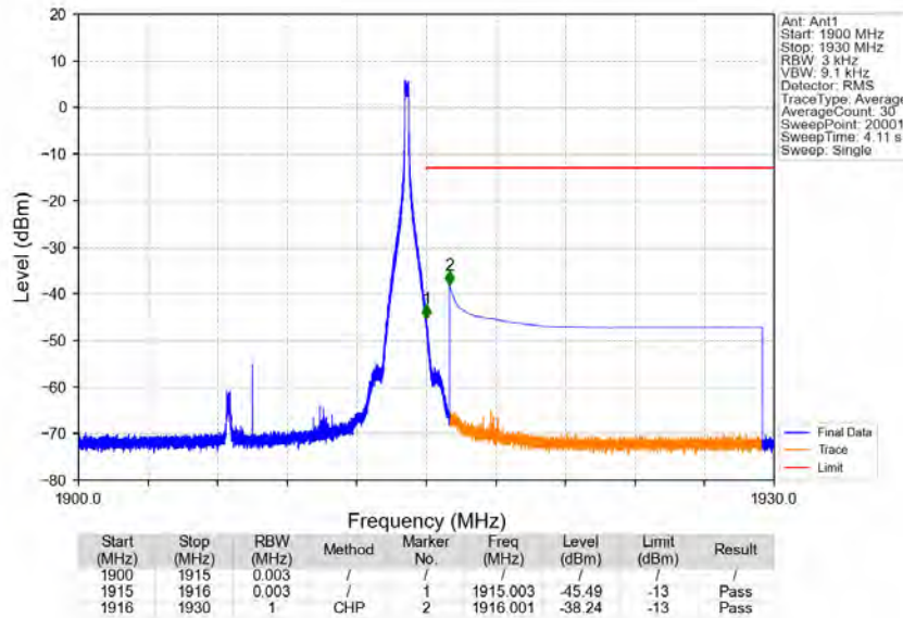
Band25_15MHz_16QAM_HCH_1907.5MHz_RB_1_74_NTNV
