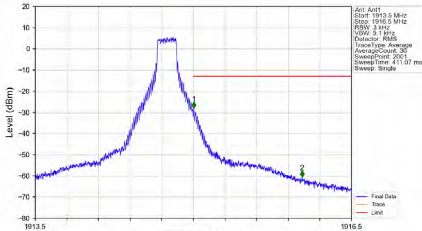
Band25_1.4MHz_16QAM_HCH_1914.3MHz_RB_1_5_NTNV
