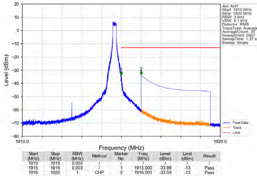
Band25_5MHz_QPSK_HCH_1912.5MHz_RB_1_24_NTNV
