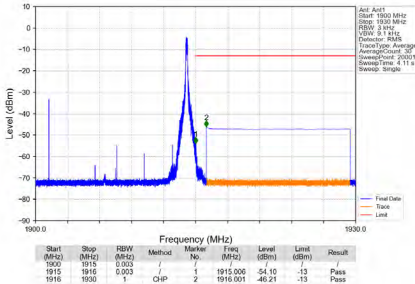
Band25_15MHz_64QAM_HCH_1907.5MHz_RB_1_74_NTNV
