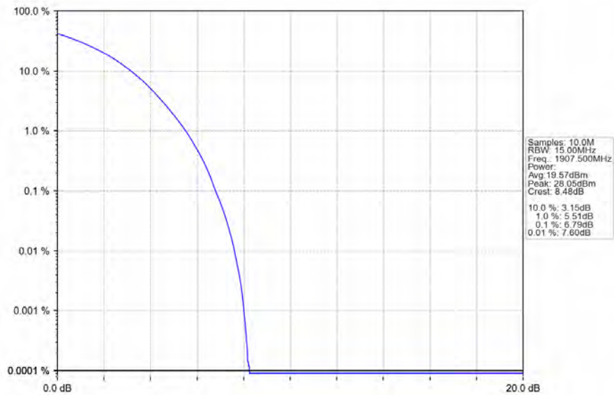
Band25_15MHz_64QAM_HCH_1907.5MHz_RB_75_0_NTNV
