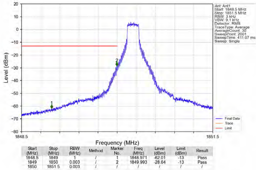
Band25_1.4MHz_16QAM_LCH_1850.7MHz_RB_1_0_NTNV
