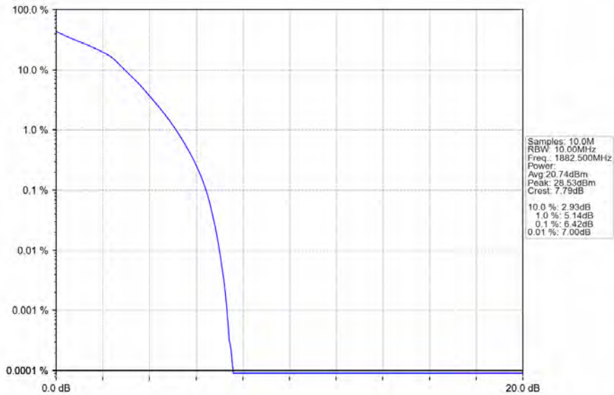
Band25_10MHz_16QAM_MCH_1882.5MHz_RB_50_0_NTNV
