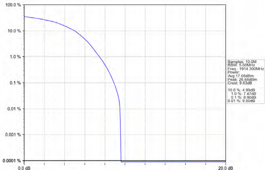
Band25_1.4MHz_64QAM_HCH_1914.3MHz_RB_6_0_NTNV
