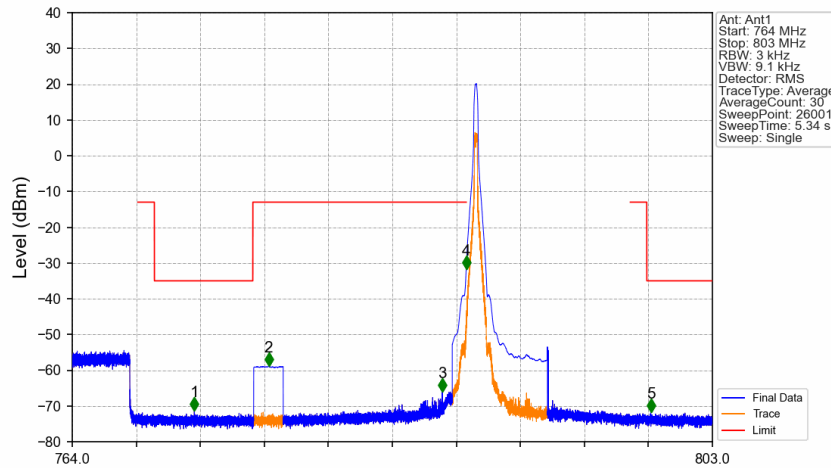
Band14_10MHz_16QAM_LCH_793MHz_RB_1_0_NTNV
