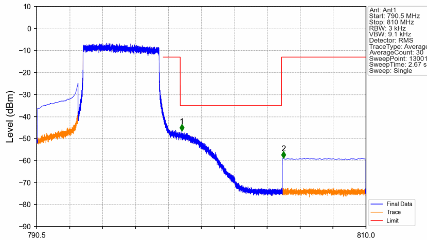
Band14_5MHz_QPSK_HCH_795.5MHz_RB_25_0_NTNV
