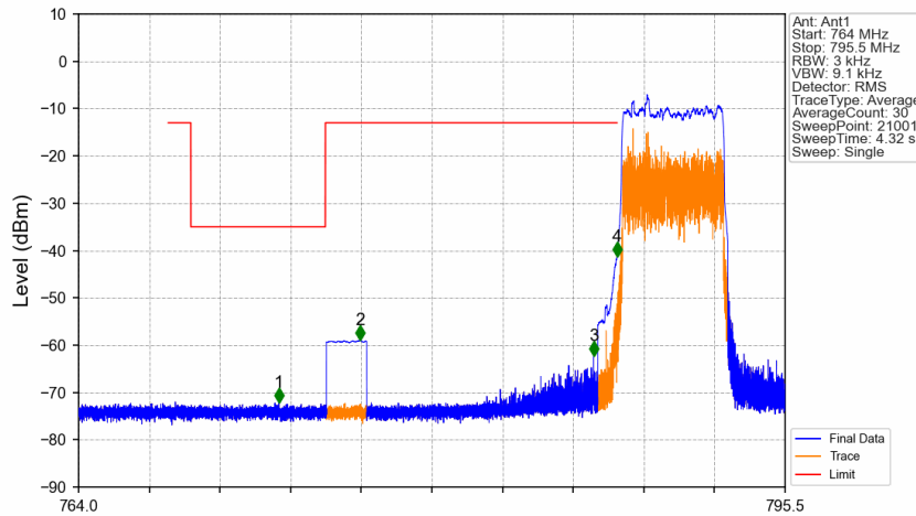
Band14_5MHz_64QAM_LCH_790.5MHz_RB_25_0_NTNV
