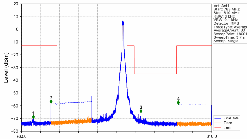
Band14_10MHz_16QAM_HCH_793MHz_RB_1_49_NTNV
