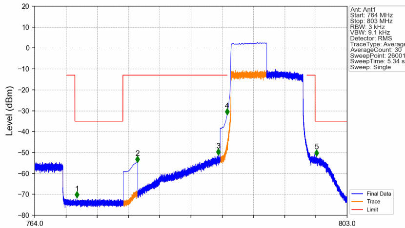
Band14_10MHz_16QAM_LCH_793MHz_RB_50_0_NTNV
