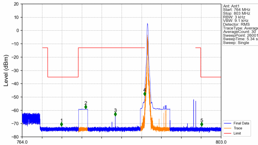
Band14_10MHz_64QAM_LCH_793MHz_RB_1_0_NTNV
