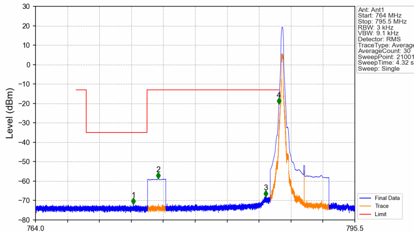
Band14_5MHz_64QAM_LCH_790.5MHz_RB_1_0_NTNV
