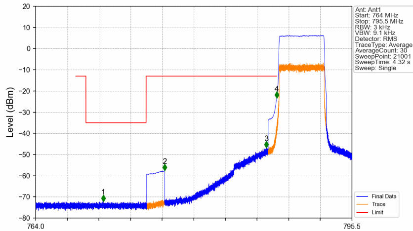
Band14_5MHz_QPSK_LCH_790.5MHz_RB_25_0_NTNV
