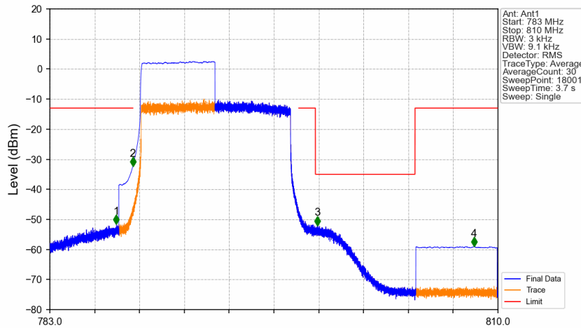
Band14_10MHz_16QAM_MCH_793MHz_RB_50_0_NTNV
