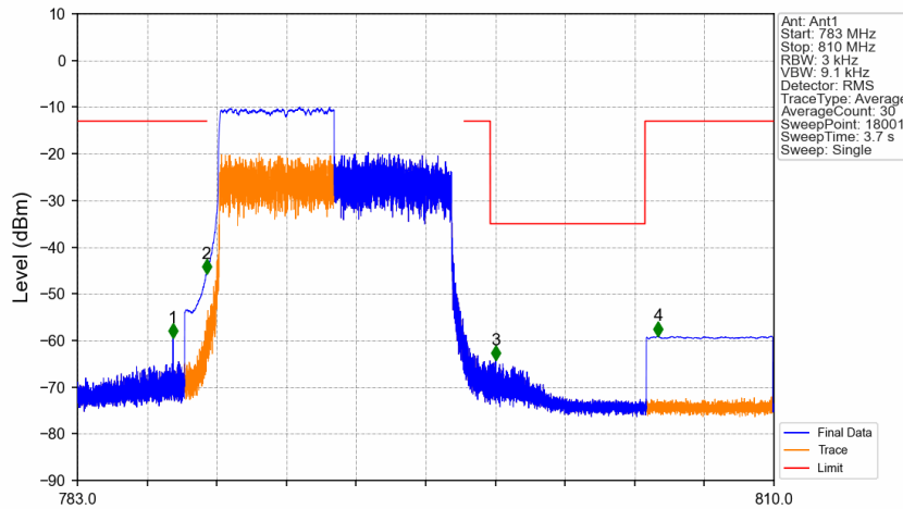
Band14_10MHz_64QAM_MCH_793MHz_RB_50_0_NTNV
