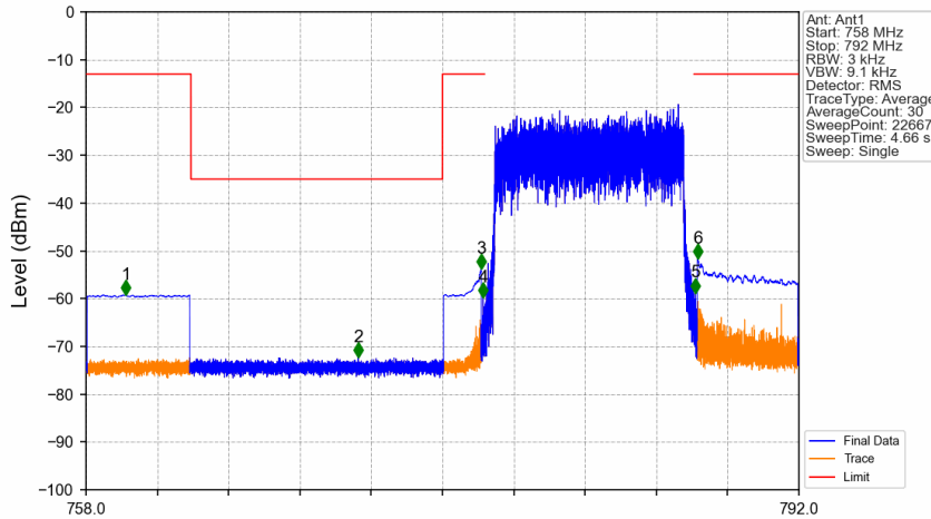
Band13_10MHz_64QAM_LCH_782MHz_RB_50_0_NTNV
