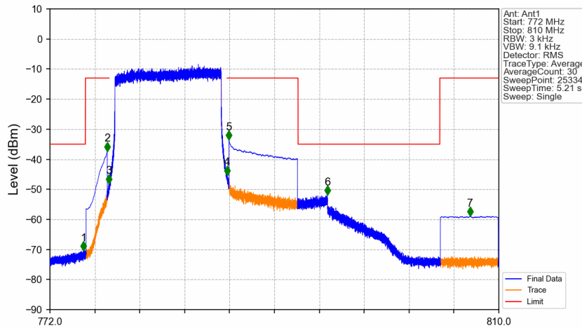
Band13_10MHz_QPSK_HCH_782MHz_RB_50_0_NTNV
