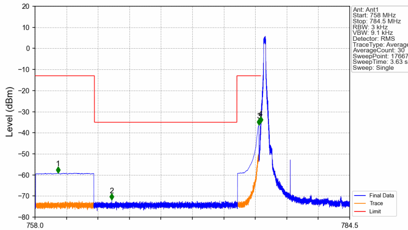
Band13_5MHz_64QAM_LCH_779.5MHz_RB_1_0_NTNV
