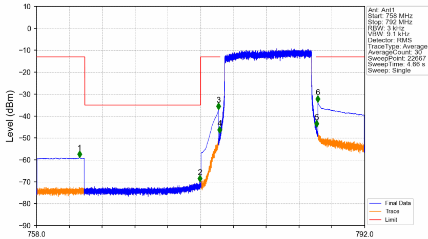
Band13_10MHz_QPSK_LCH_782MHz_RB_50_0_NTNV
