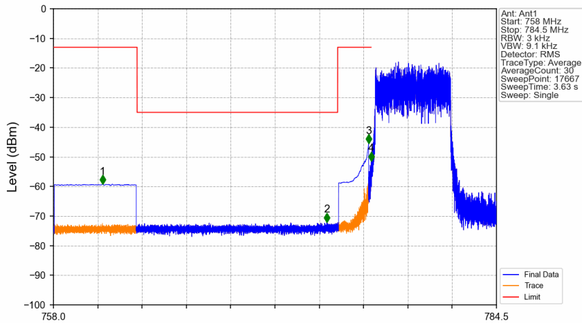
Band13_5MHz_64QAM_LCH_779.5MHz_RB_25_0_NTNV
