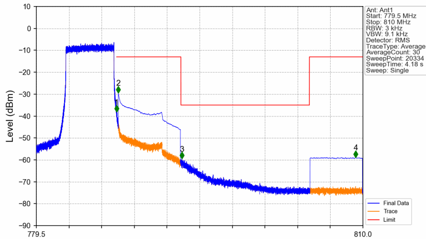
Band13_5MHz_QPSK_HCH_784.5MHz_RB_25_0_NTNV
