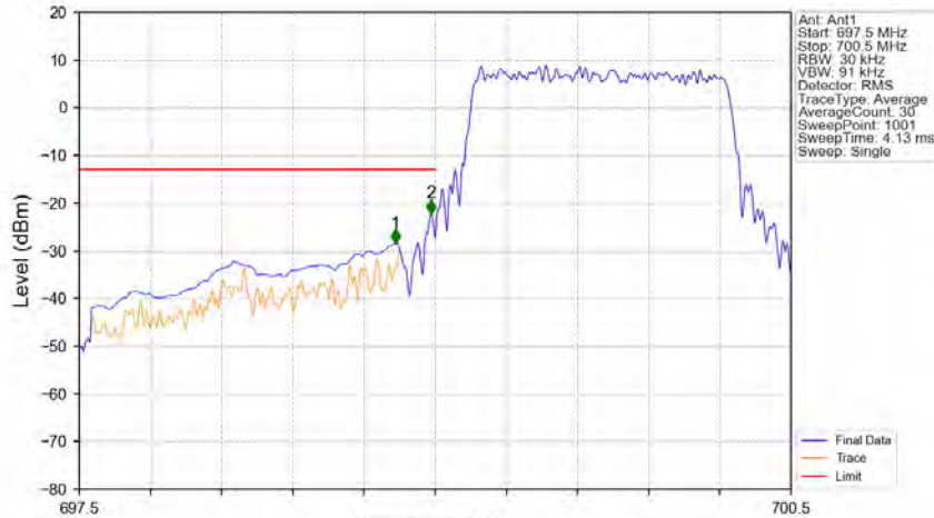
Band12_1.4MHz_QPSK_LCH_699.7MHz_RB_6_0_NTNV
