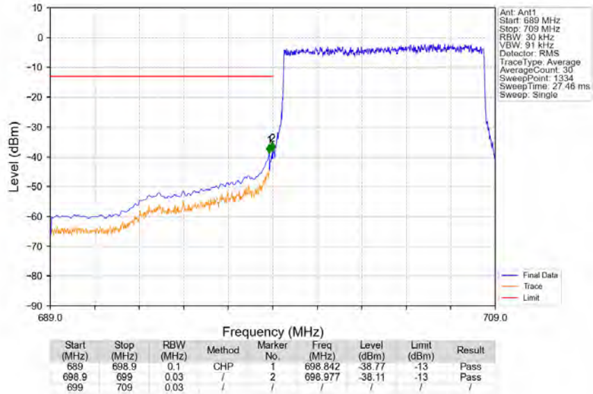
Band12_10MHz_64QAM_LCH_704MHz_RB_50_0_NTNV
