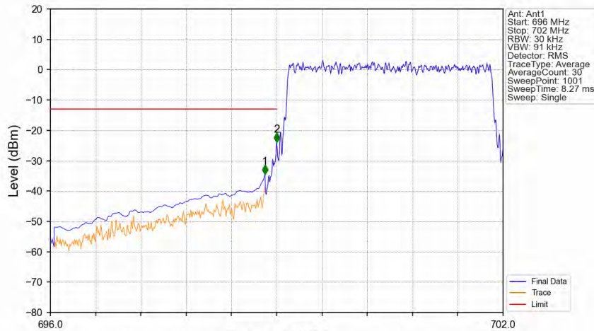
Band12_3MHz_64QAM_LCH_700.5MHz_RB_15_0_NTNV
