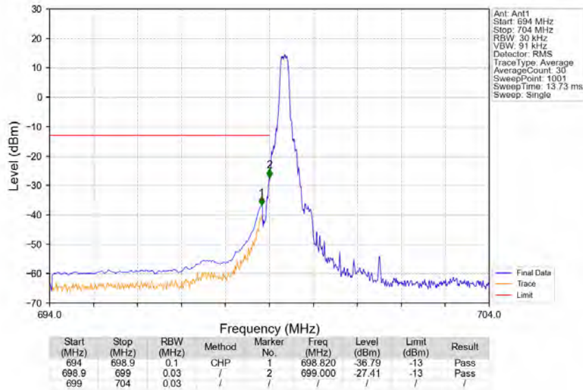
Band12_5MHz_64QAM_LCH_701.5MHz_RB_1_0_NTNV
