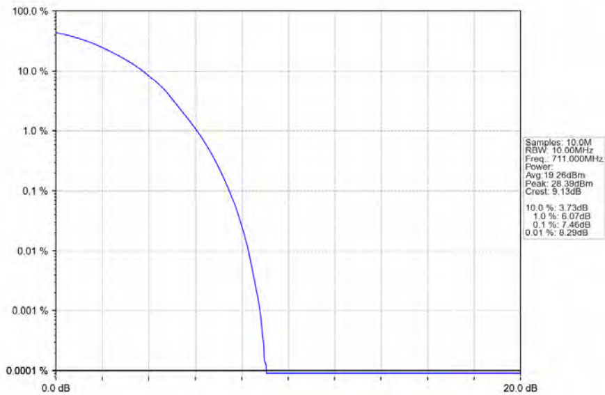
Band12_10MHz_64QAM_HCH_711MHz_RB_50_0_NTNV
