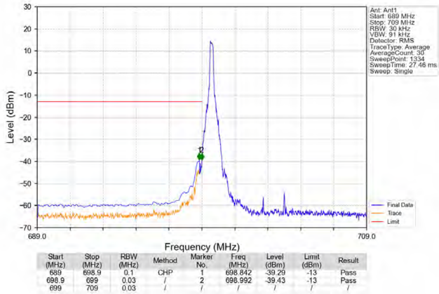
Band12_10MHz_64QAM_LCH_704MHz_RB_1_0_NTNV
