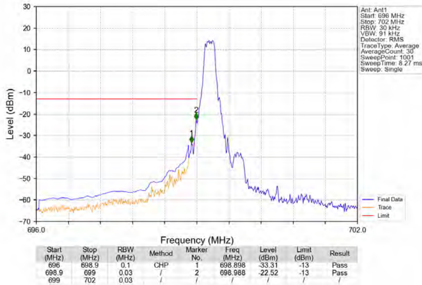
Band12_3MHz_64QAM_LCH_700.5MHz_RB_1_0_NTNV
