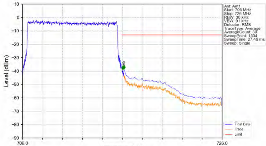
Band12_10MHz_64QAM_HCH_711MHz_RB_50_0_NTNV
