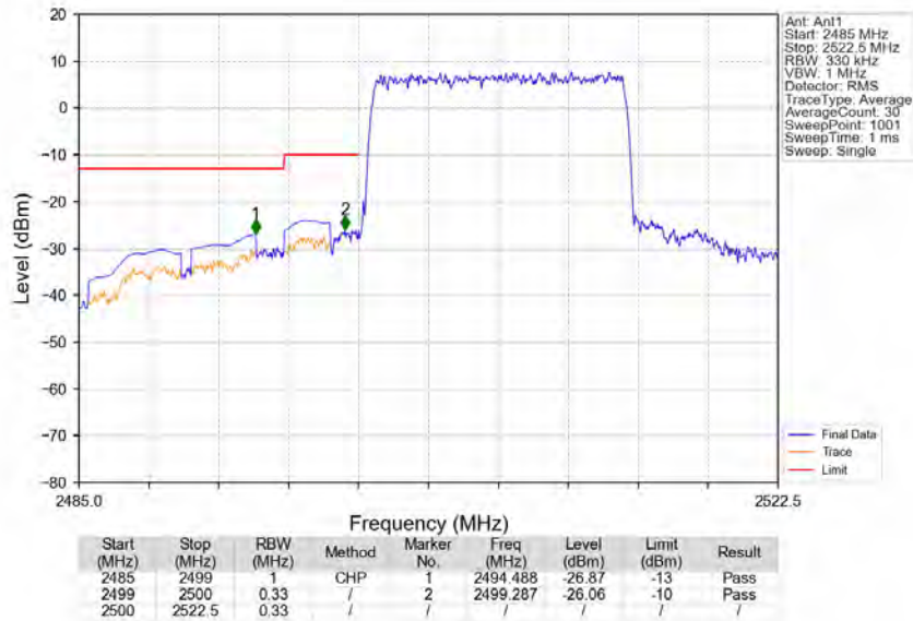
Band7_15MHz_QPSK_LCH_2507.5MHz_RB_75_0_NTNV
