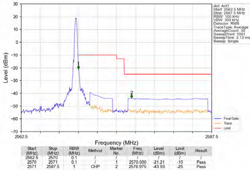
Band7_5MHz_16QAM_HCH_2567.5MHz_RB_1_24_NTNV
