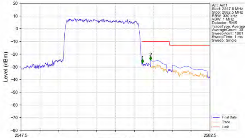
Band7_15MHz_QPSK_HCH_2562.5MHz_RB_75_0_NTNV
