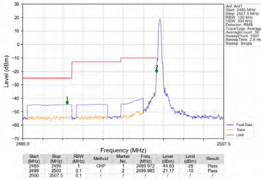
Band7_5MHz_64QAM_LCH_2502.5MHz_RB_1_0_NTNV
