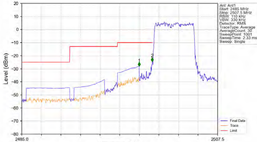
Band7_5MHz_64QAM_LCH_2502.5MHz_RB_25_0_NTNV
