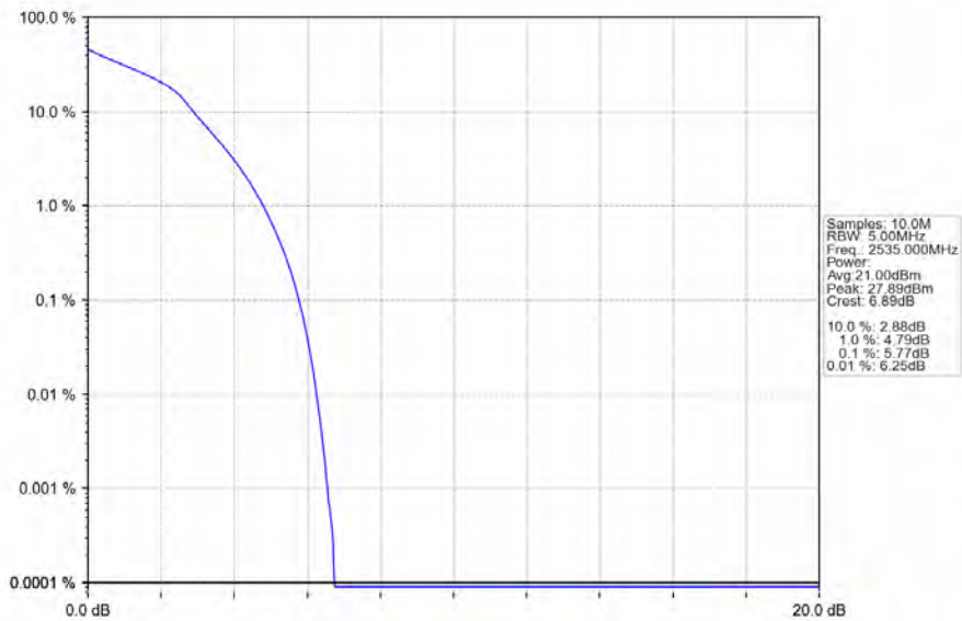
Band7_5MHz_16QAM_MCH_2535MHz_RB_25_0_NTNV
