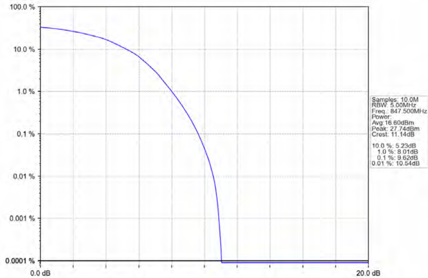
Band5_3MHz_64QAM_HCH_847.5MHz_RB_15_0_NTNV
