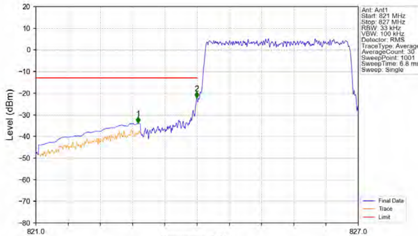
Band5_3MHz_QPSK_LCH_825.5MHz_RB_15_0_NTNV
