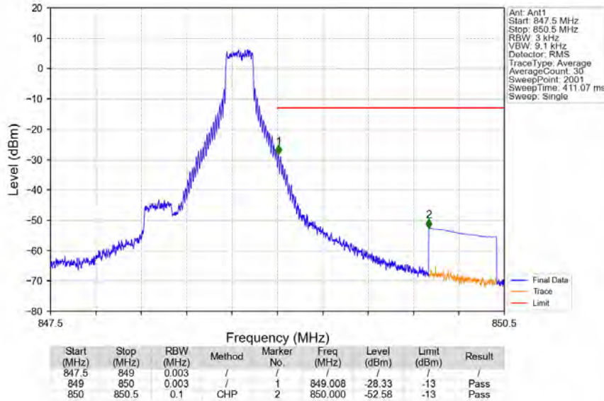
Band5_1.4MHz_16QAM_HCH_848.3MHz_RB_1_5_NTNV
