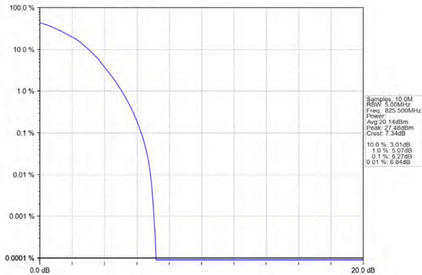
Band5_3MHz_64QAM_LCH_825.5MHz_RB_15_0_NTNV
