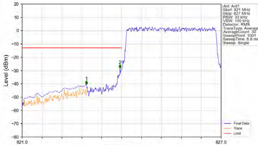
Band5_3MHz_64QAM_LCH_825.5MHz_RB_15_0_NTNV
