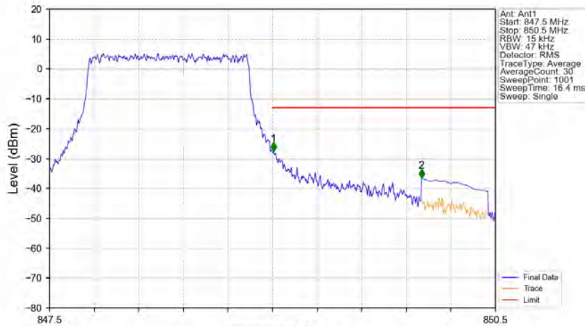
Band5_1.4MHz_QPSK_HCH_848.3MHz_RB_6_0_NTNV
