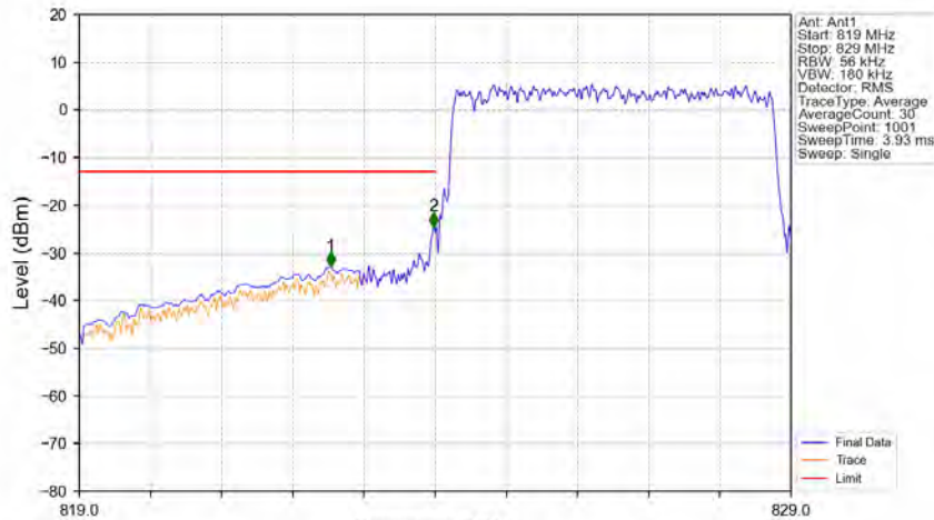
Band5_5MHz_QPSK_LCH_826.5MHz_RB_25_0_NTNV
