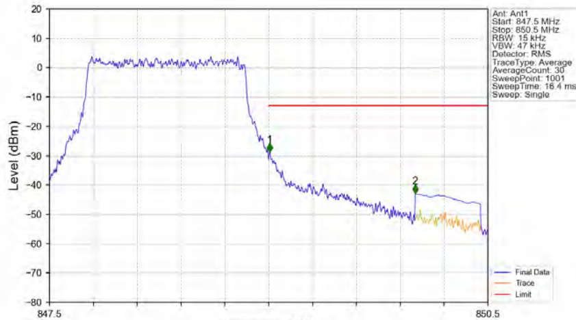
Band5_1.4MHz_64QAM_HCH_848.3MHz_RB_6_0_NTNV
