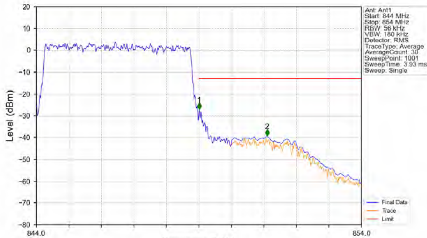
Band5_5MHz_64QAM_HCH_846.5MHz_RB_25_0_NTNV
