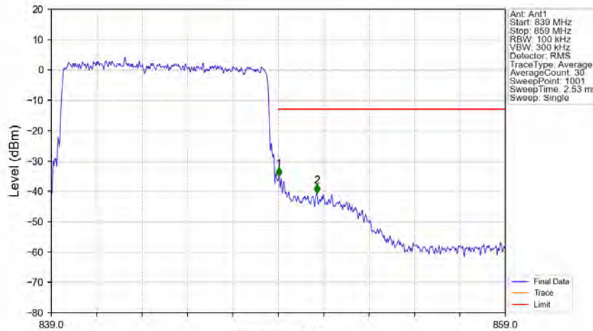
Band5_10MHz_64QAM_HCH_844MHz_RB_50_0_NTNV
