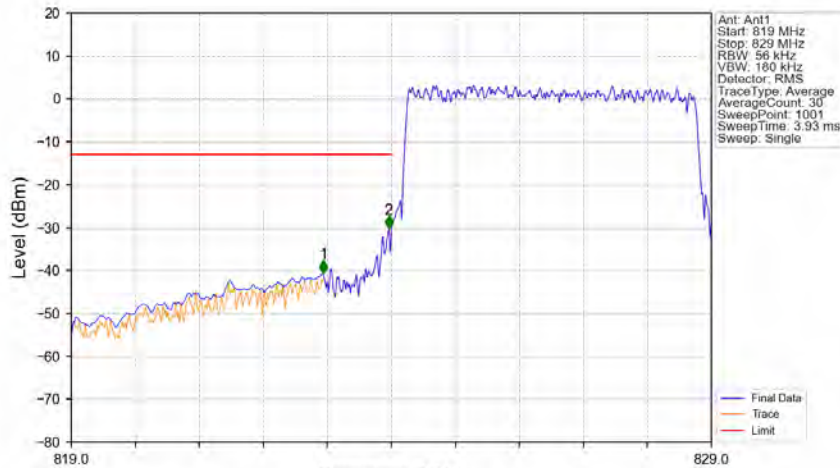
Band5_5MHz_64QAM_LCH_826.5MHz_RB_25_0_NTNV
