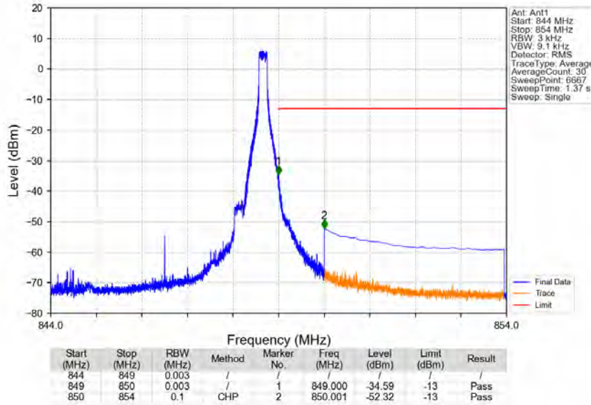
Band5_5MHz_16QAM_HCH_846.5MHz_RB_1_24_NTNV
