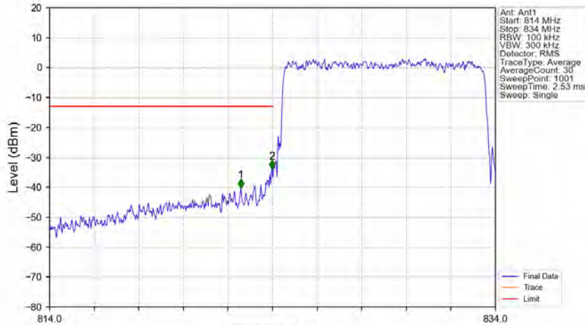
Band5_10MHz_64QAM_LCH_829MHz_RB_50_0_NTNV
