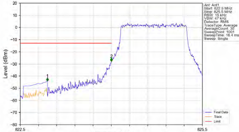
Band5_1.4MHz_64QAM_LCH_824.7MHz_RB_6_0_NTNV
