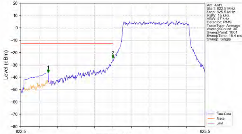
Band5_1.4MHz_QPSK_LCH_824.7MHz_RB_6_0_NTNV
