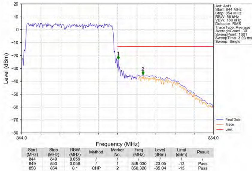
Band5_5MHz_QPSK_HCH_846.5MHz_RB_25_0_NTNV
