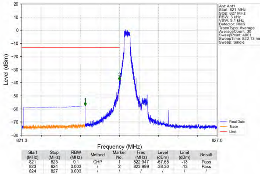
Band5_3MHz_64QAM_LCH_825.5MHz_RB_1_0_NTNV
