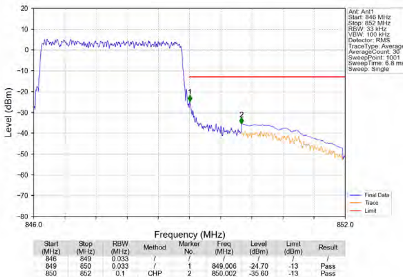
Band5_3MHz_QPSK_HCH_847.5MHz_RB_15_0_NTNV
