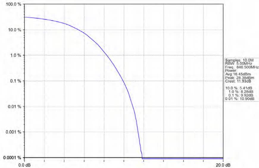
Band5_5MHz_64QAM_HCH_846.5MHz_RB_25_0_NTNV
