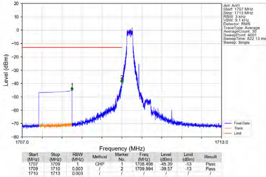
Band4_3MHz_64QAM_LCH_1711.5MHz_RB_1_0_NTNV
