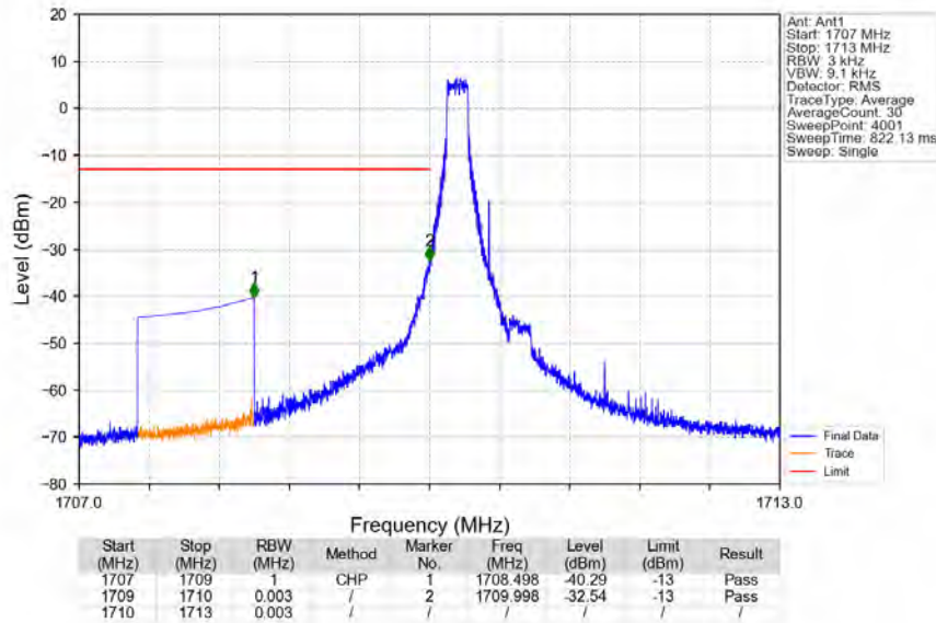
Band4_3MHz_16QAM_LCH_1711.5MHz_RB_1_0_NTNV
