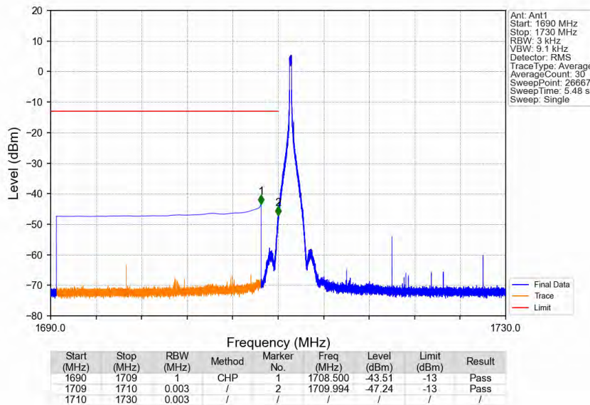
Band4_20MHz_64QAM_LCH_1720MHz_RB_1_0_NTNV
