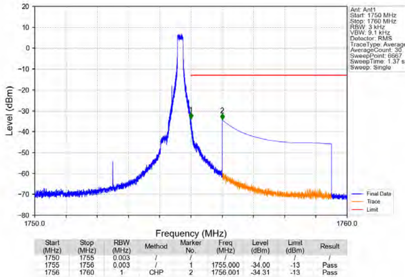
Band4_5MHz_QPSK_HCH_1752.5MHz_RB_1_24_NTNV
