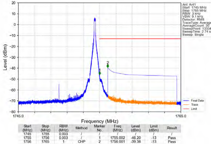
Band4_10MHz_16QAM_HCH_1750MHz_RB_1_49_NTNV
