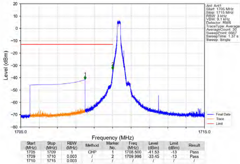
Band4_5MHz_16QAM_LCH_1712.5MHz_RB_1_0_NTNV
