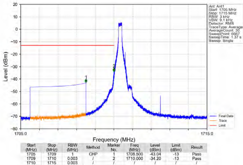
Band4_5MHz_64QAM_LCH_1712.5MHz_RB_1_0_NTNV
