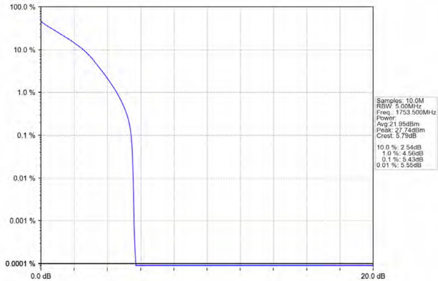
Band4_3MHz_QPSK_HCH_1753.5MHz_RB_15_0_NTNV
