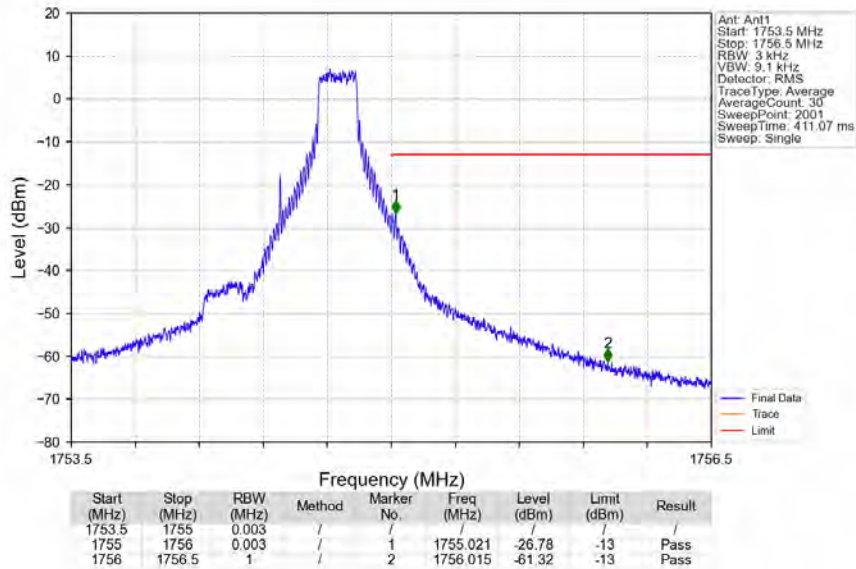
Band4_1.4MHz_QPSK_HCH_1754.3MHz_RB_1_5_NTNV
