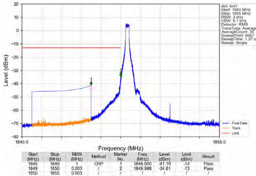
Band2_5MHz_16QAM_LCH_1852.5MHz_RB_1_0_NTNV
