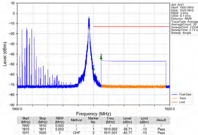
Band2_10MHz_64QAM_HCH_1905MHz_RB_1_49_NTNV
