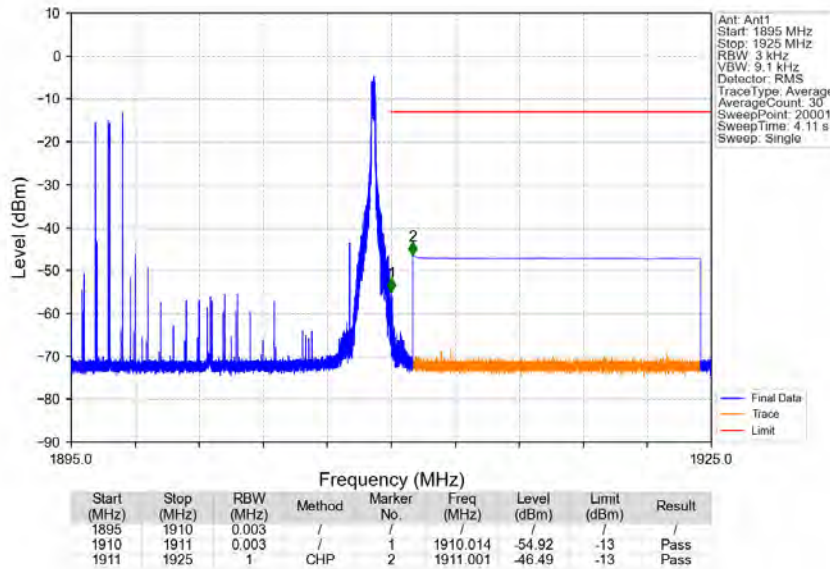
Band2_15MHz_64QAM_HCH_1902.5MHz_RB_1_74_NTNV
