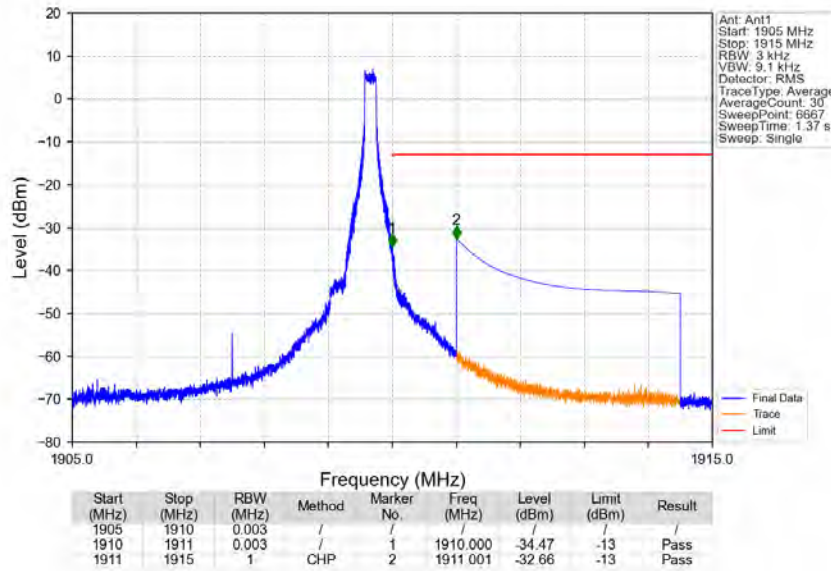
Band2_5MHz_QPSK_HCH_1907.5MHz_RB_1_24_NTNV
