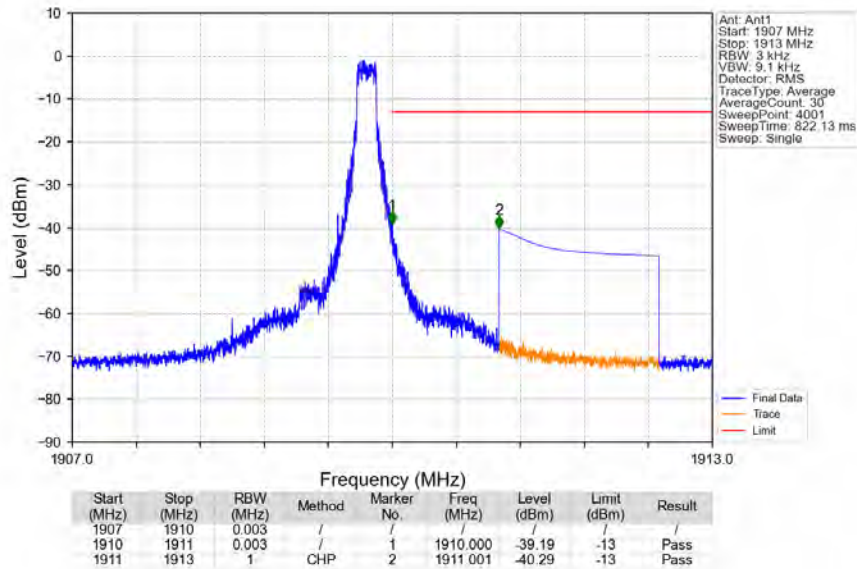
Band2_3MHz_64QAM_HCH_1908.5MHz_RB_1_14_NTNV
