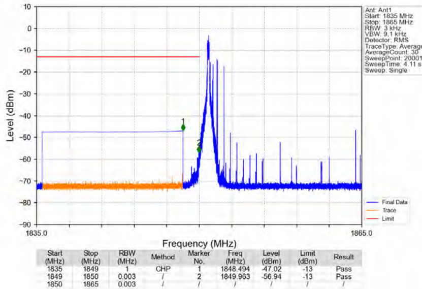
Band2_15MHz_64QAM_LCH_1857.5MHz_RB_1_0_NTNV
