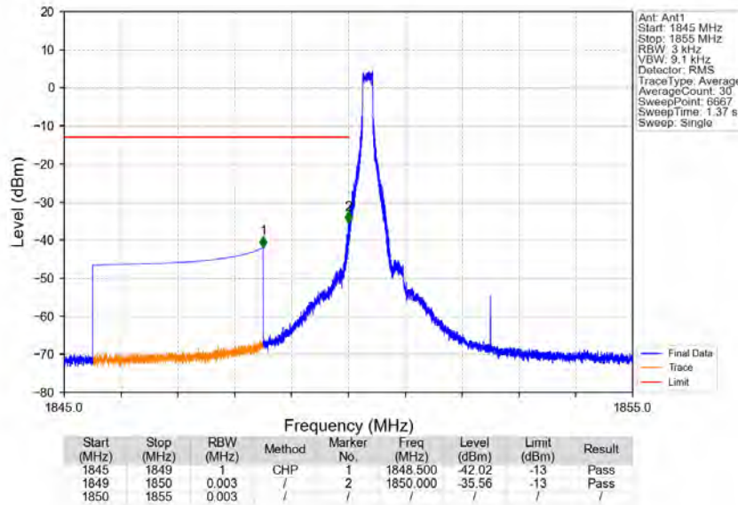
Band2_5MHz_64QAM_LCH_1852.5MHz_RB_1_0_NTNV
