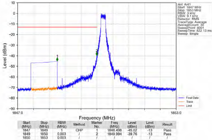
Band2_3MHz_64QAM_LCH_1851.5MHz_RB_1_0_NTNV
