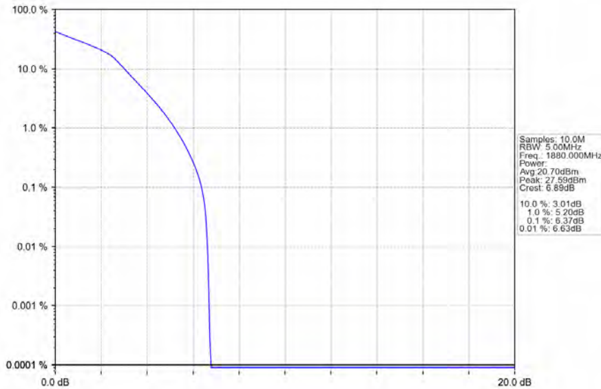
Band2_3MHz_16QAM_MCH_1880MHz_RB_15_0_NTNV
