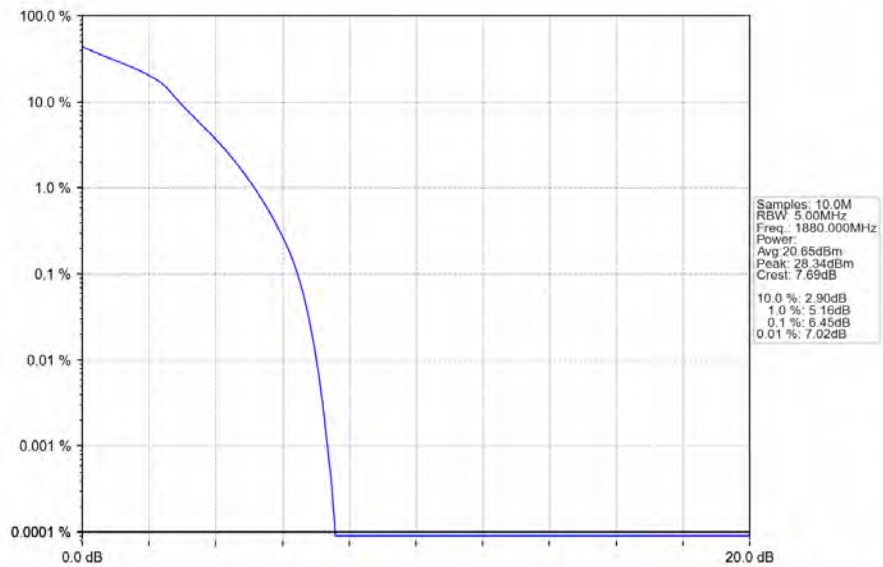
Band2_5MHz_16QAM_MCH_1880MHz_RB_25_0_NTNV
