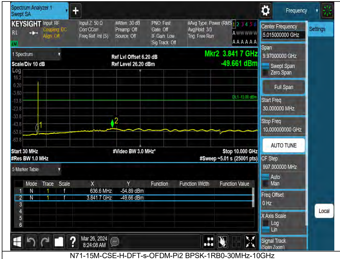
N71-15M-CSE-H-DFT-s-OFDM-Pi2 BPSK-1RB0-30MHz-10GHz
