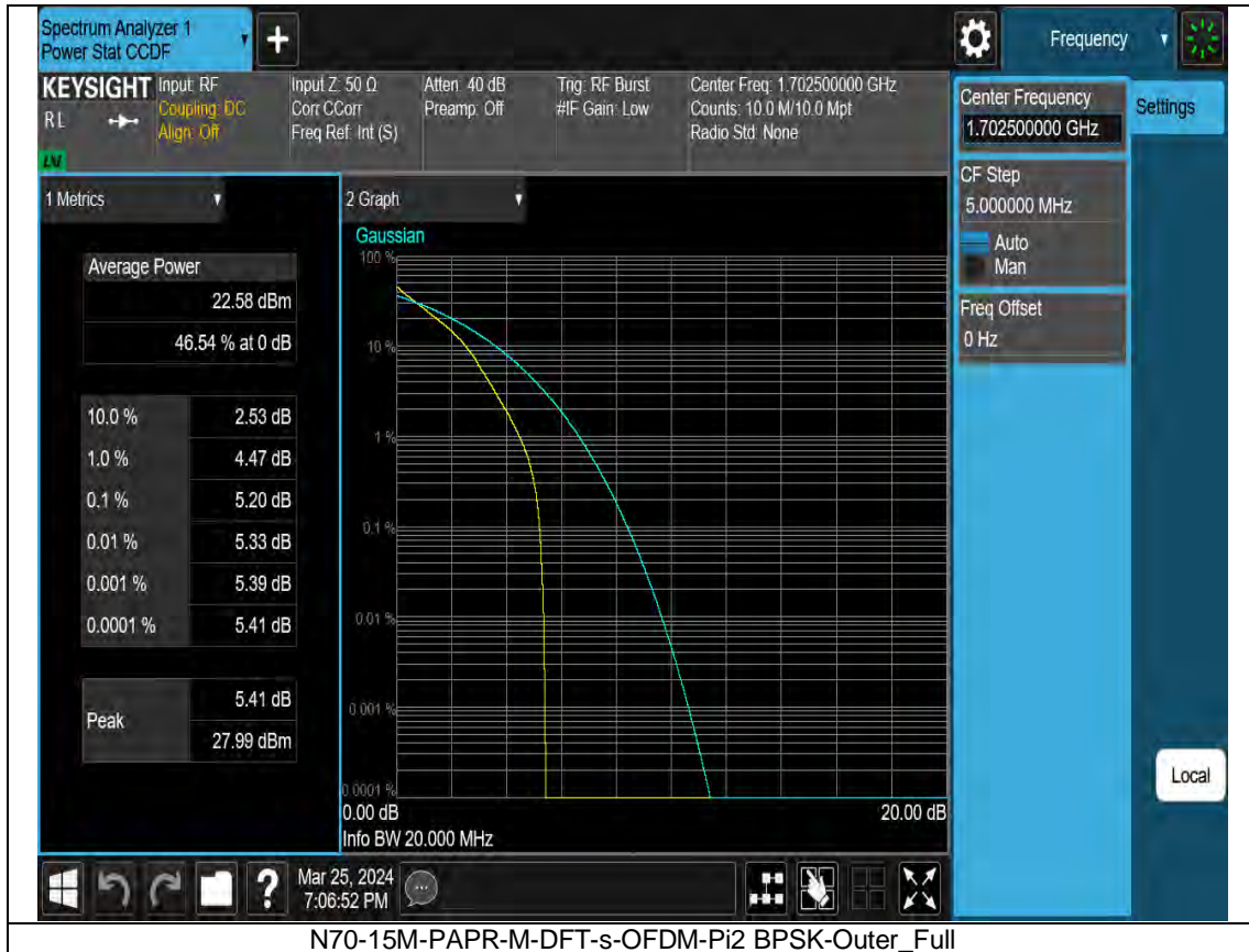
N70-15M-PAPR-M-DFT-s-OFDM-Pi2 BPSK-Outer_Full
