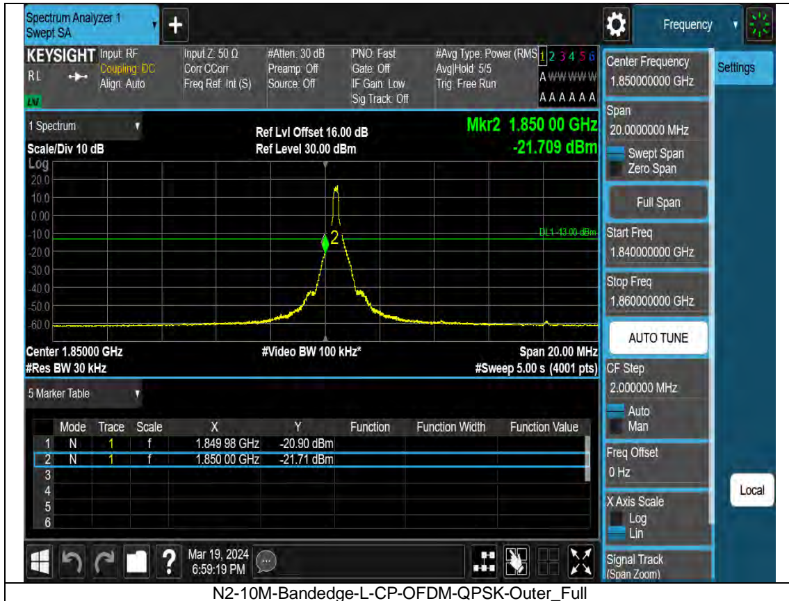
N2-10M-Bandedge-L-CP-OFDM-QPSK-Outer_Full
