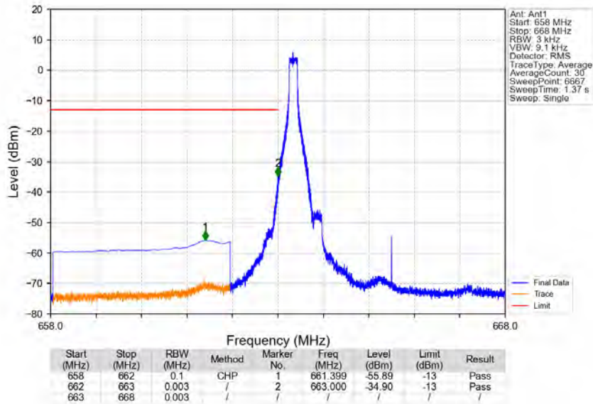
Band71_5MHz_64QAM_LCH_665.5MHz_RB_1_0_NTNV
