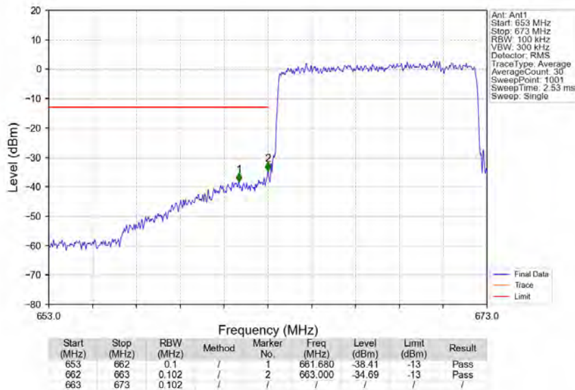
Band71_10MHz_64QAM_LCH_668MHz_RB_50_0_NTNV
