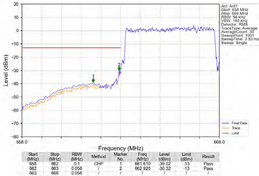
Band71 5MHz 64QAM_LCH 665.5MHz RB 25 0 NTV
