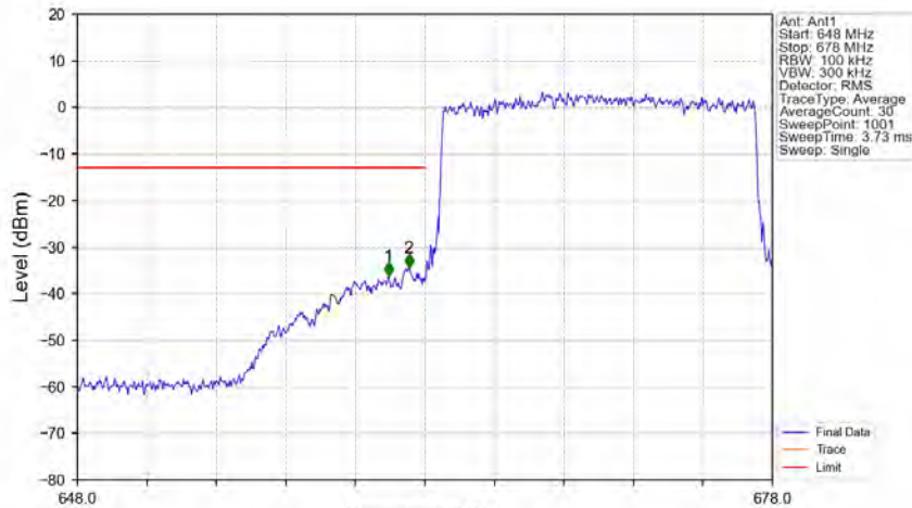
Band71_15MHz_QPSK_LCH_670.5MHz_RB_75_0_NTNV
