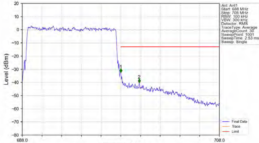
Band71_10MHz_64QAM_HCH_693MHz_RB_50_0_NTNV
