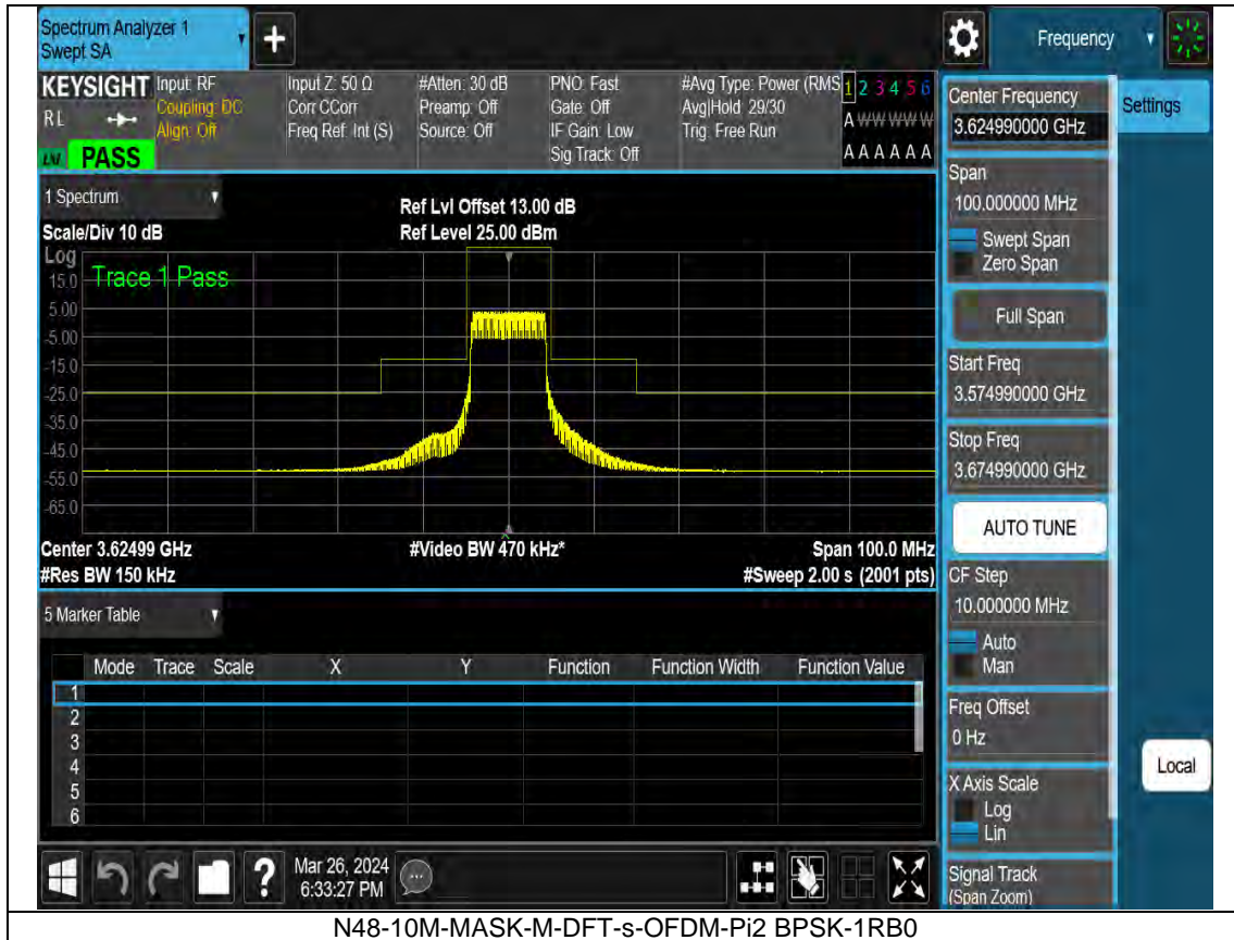
N48-10M-MASK-M-DFT-s-OFDM-Pi2 BPSK-1RB0
