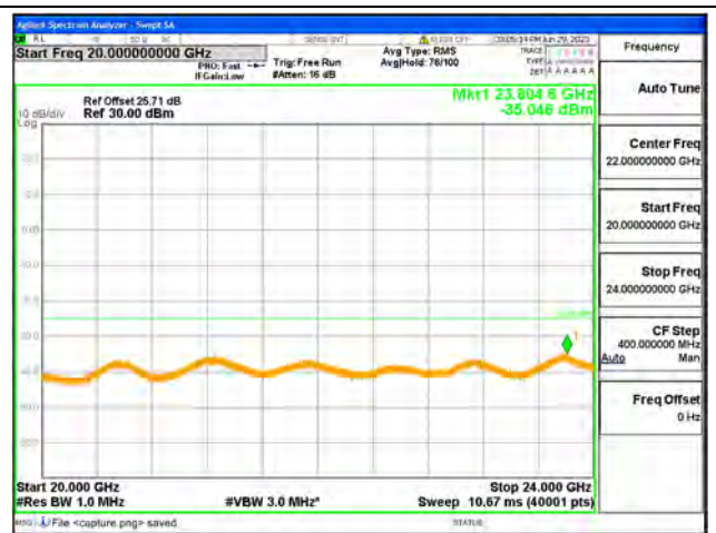
Band30-20G-24G / 10MHz / Mid CH / QPSK
