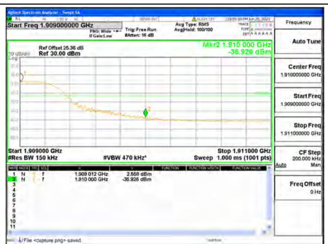
Band2 / 15MHz / High CH / QPSK / FULL RB
