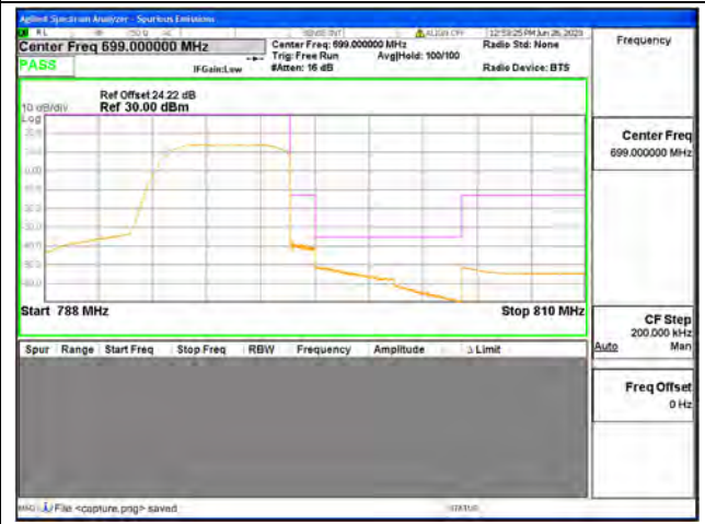
Band14 / 5MHz / High CH / QPSK / FULL RB
