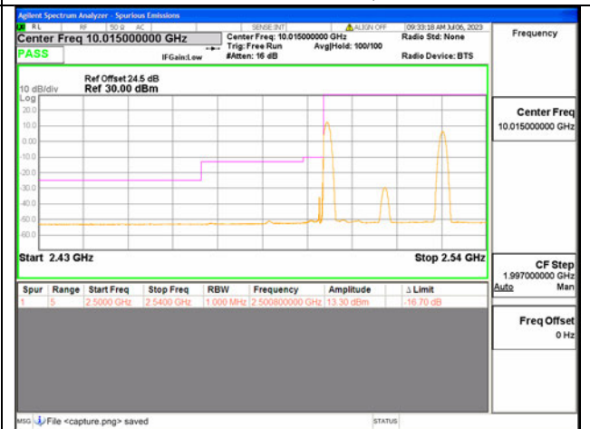
7C / 15+10MHz / Low CH / QPSK / 1#0-1#74
