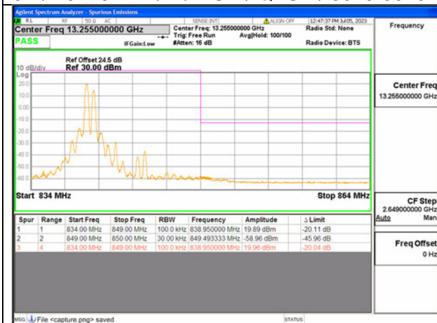
5B / 5+10MHz / High CH / QPSK / 1#24-1#0
