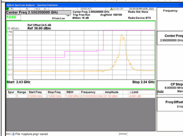
7C / 15+15MHz / Low CH / QPSK / 1#74-1#0
