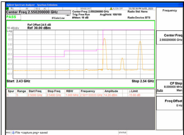
7C / 10+20MHz / Low CH / QPSK / 1#0-1#99
