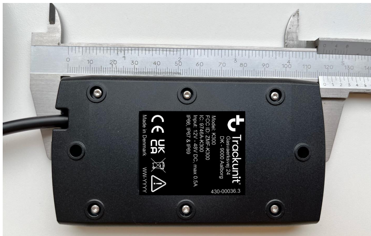
K300 from the back
