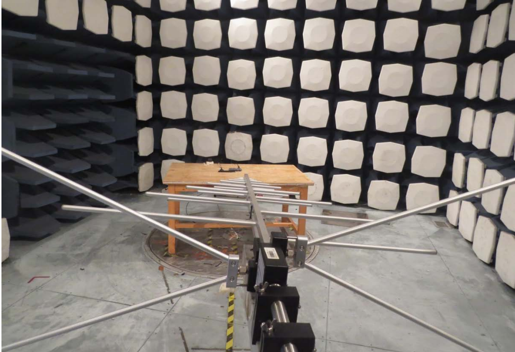
30MHz-1GHz
