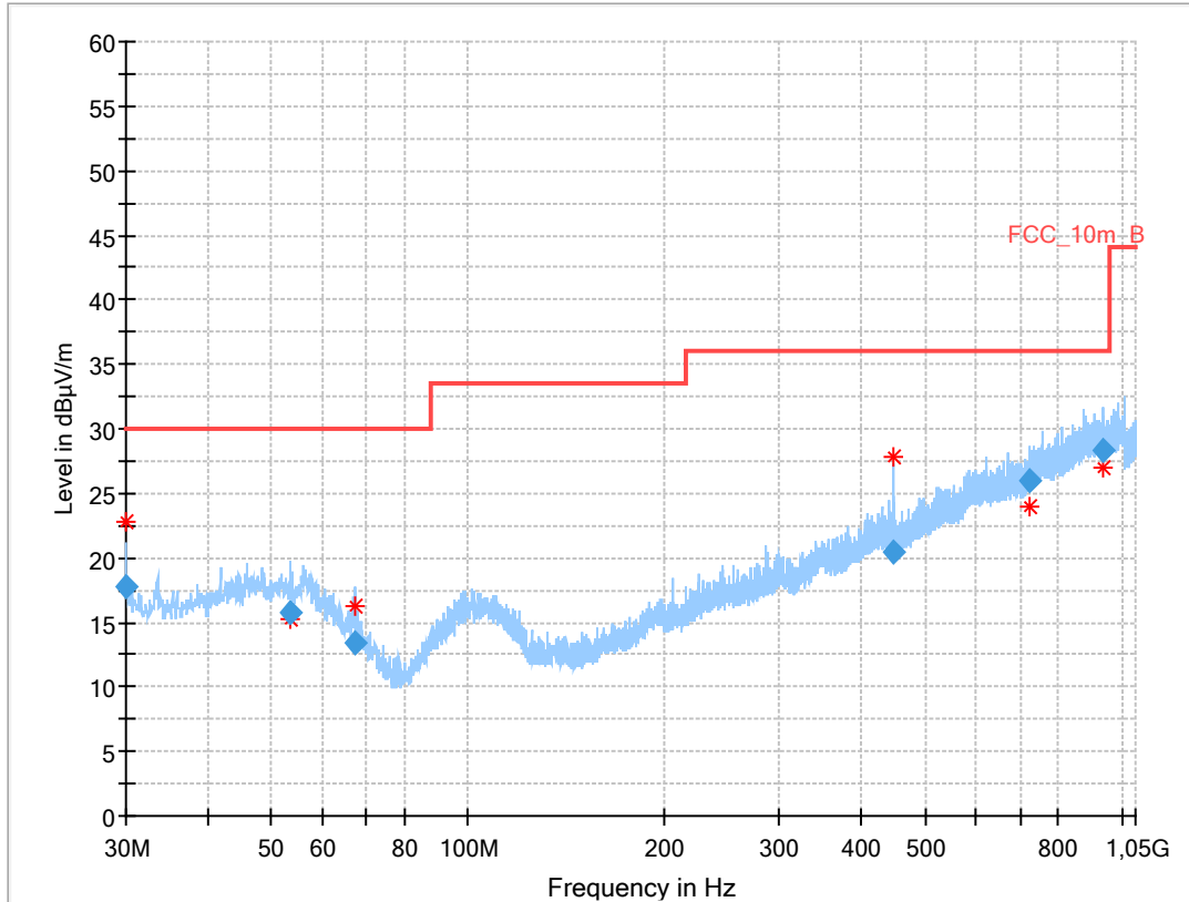
Plot 2: 30 MHz to 1 GHz, TX mode, 2446 MHz, vertical & horizontal polarization, 1 Msps
