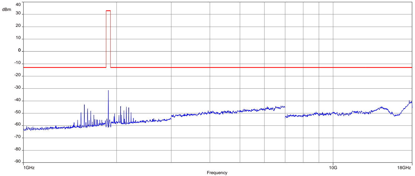
Carrier notched with 1.9 GHz rejection filter
