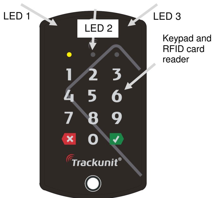
LED indications
