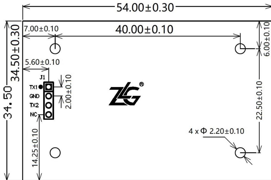
Figure 4 ZLG600A-ANT Dimension
