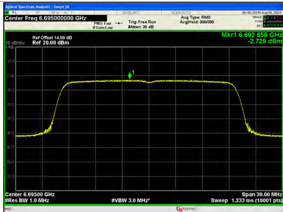
PSD NVNT ax20 6695MHz Ant2 SISO
